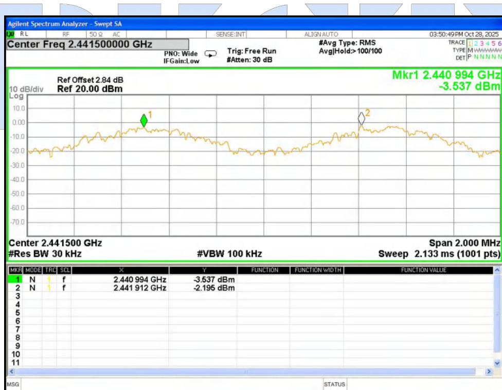
CFS NVNT 1-DH5 2441MHz Ant1
