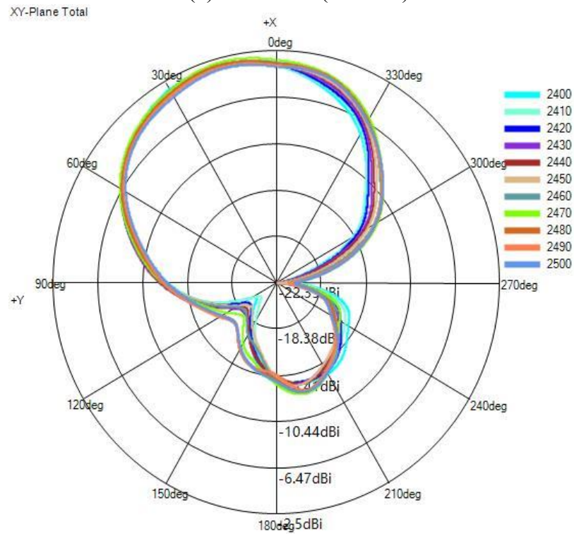
(3) X-Y Plane(unit:dBi):
