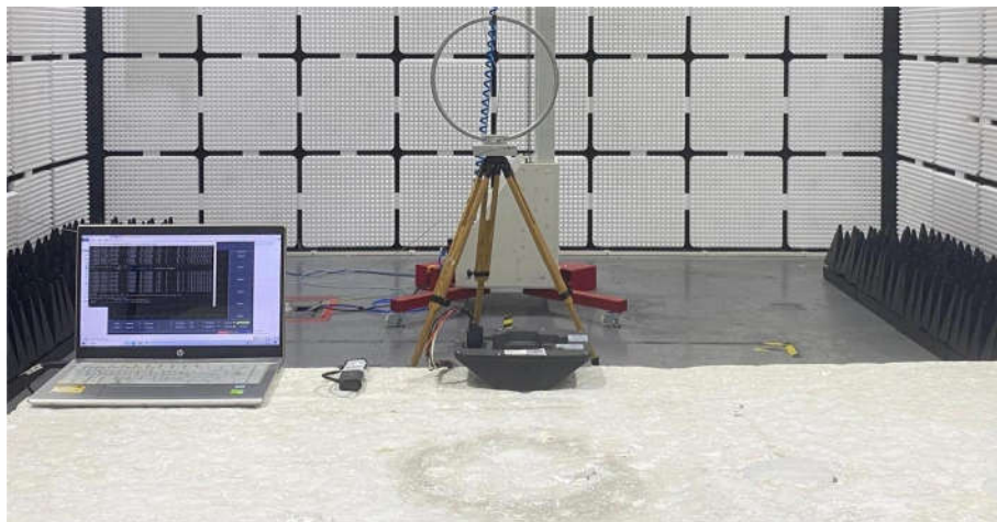
Radiated spurious emission Test Setup-1 (Below 30MHz)
