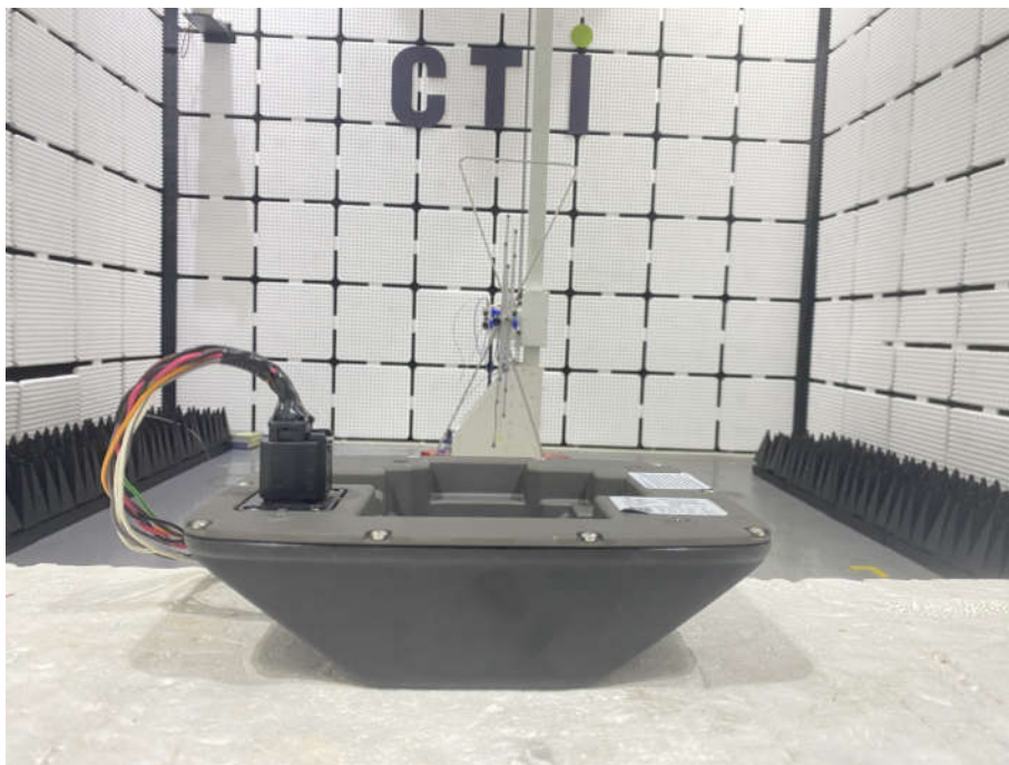
Radiated spurious emission Test Setup-3(Below 1GHz) close up
