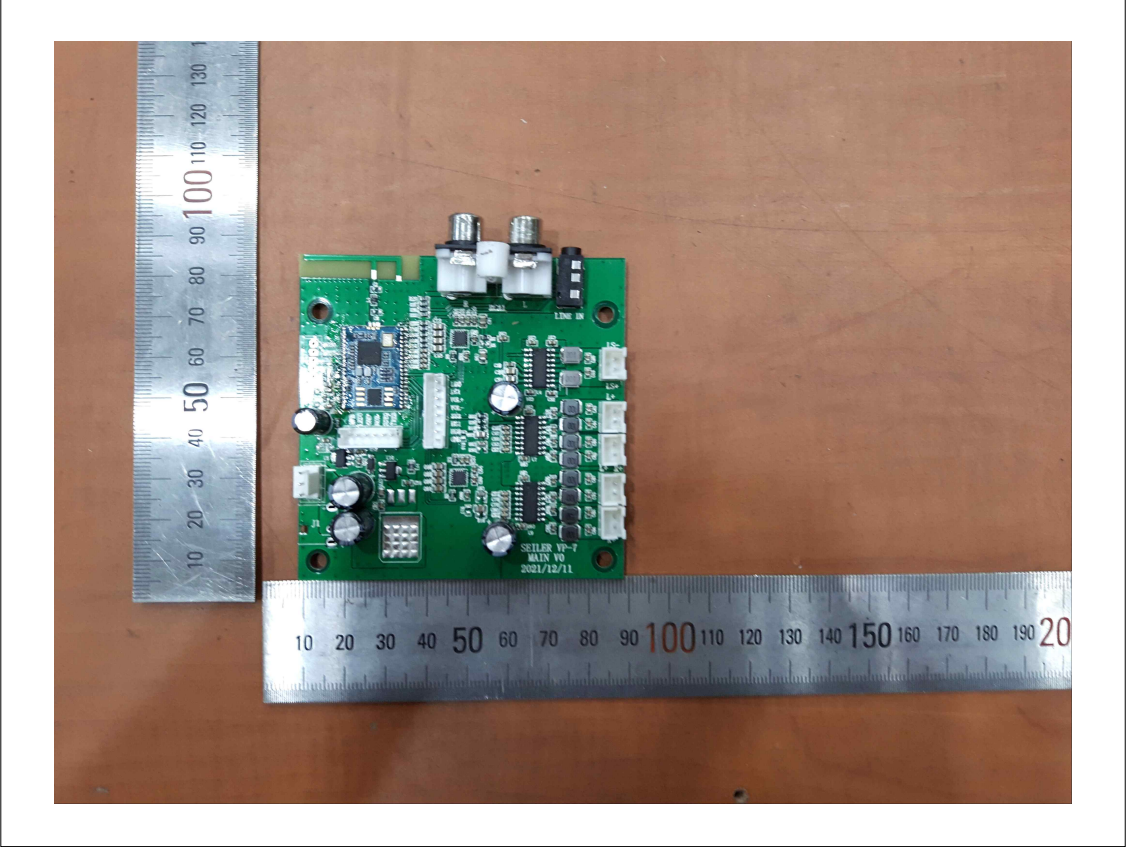
View of BT PCB (Top)
