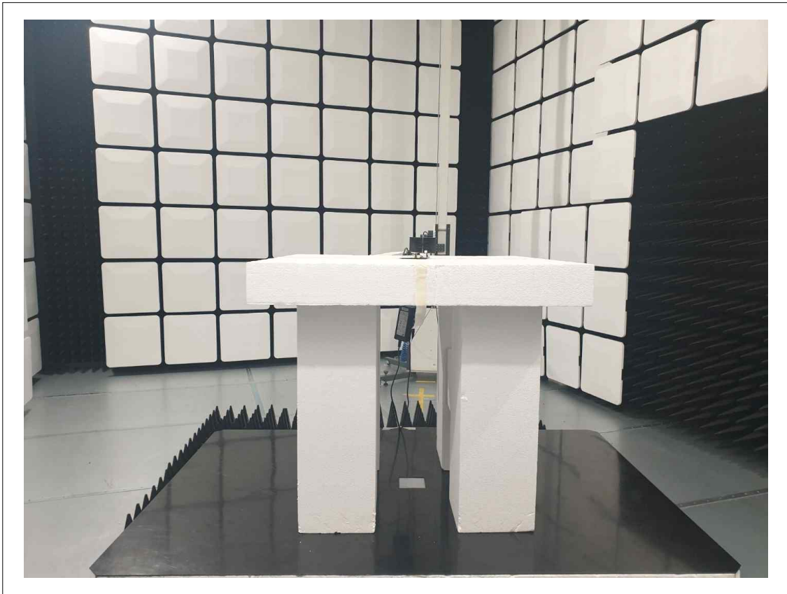
Radiated Emission Test Setup Above 1GHz_V
