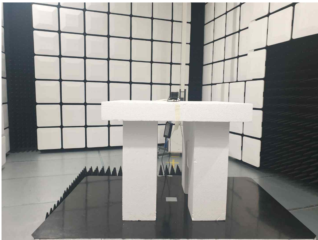
Radiated Emission Test Setup Above 1GHz_H
