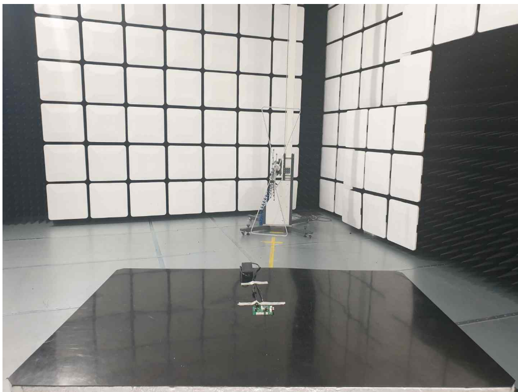
Radiated Emission Test Setup Below 1GHz_V
