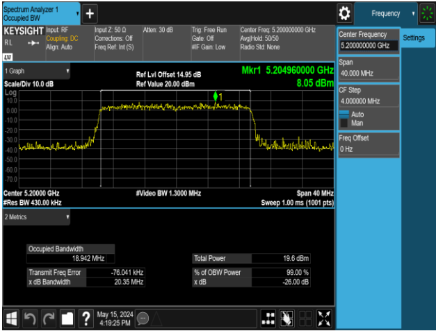
11AX20MIMO-Ant2-5200-106Tone-RU54
