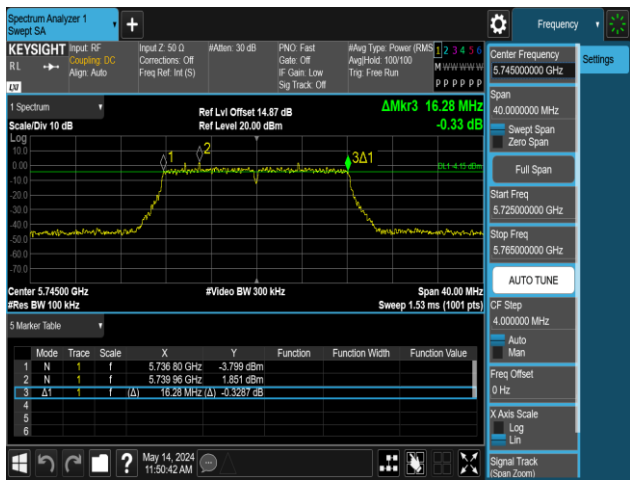
11A-Ant1-5745-PASS
