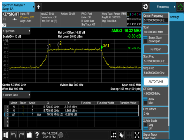
11A-Ant1-5785-PASS
