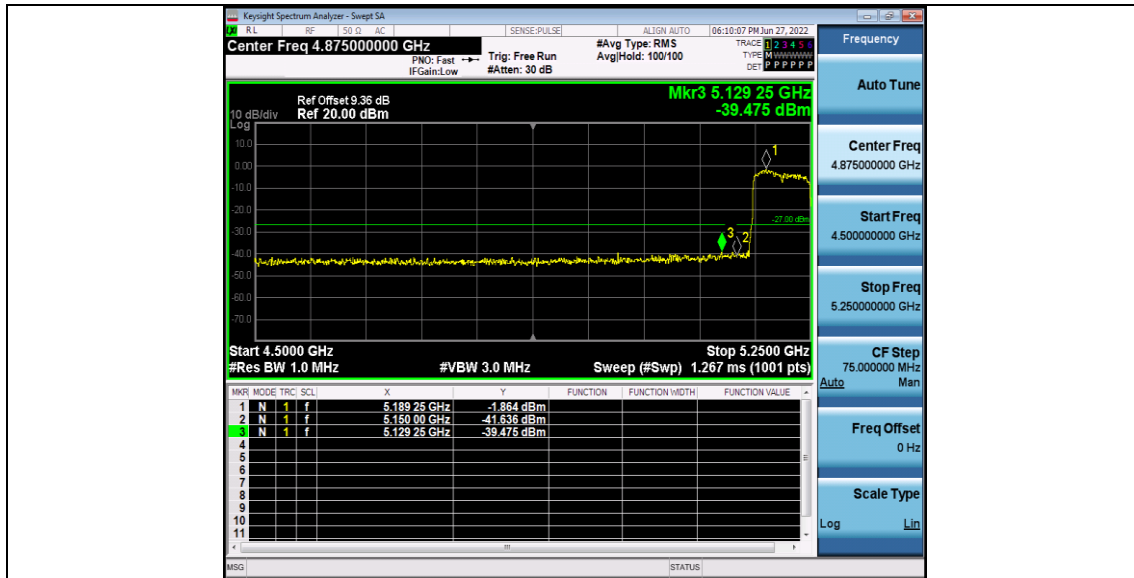
11AC80SISO_Ant1_High_5290
