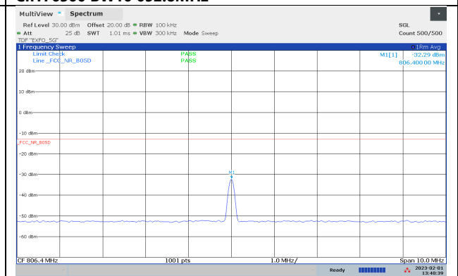
Ch176300 BW10 806.4MHz
