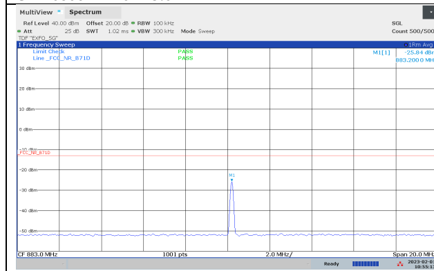
Ch126800 BW10 883.2MHz
