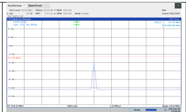
Ch176300 BW10 576MHz
