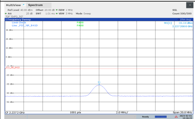
Ch392500 BW10 2227.2MHz
