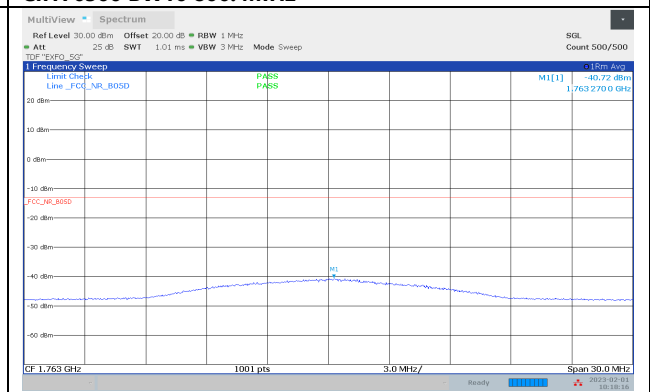
Ch176300 BW10 1763.2MHz
