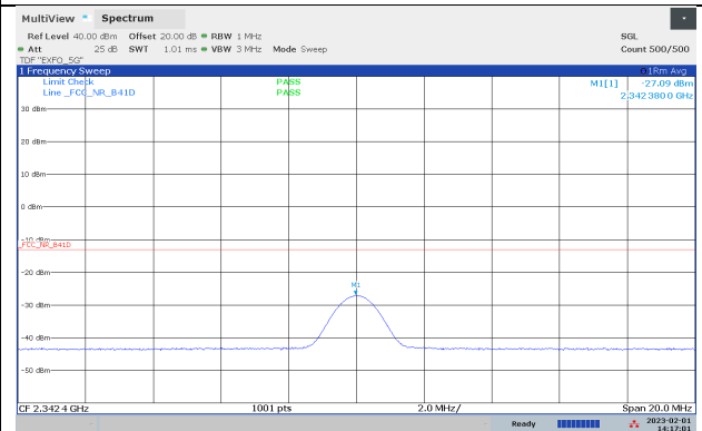
Ch392500 BW10 2342.4MHz
