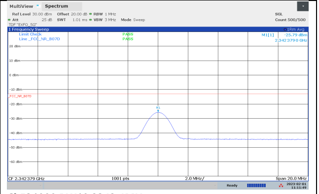
Ch531000 BW10 2342.4MHz
