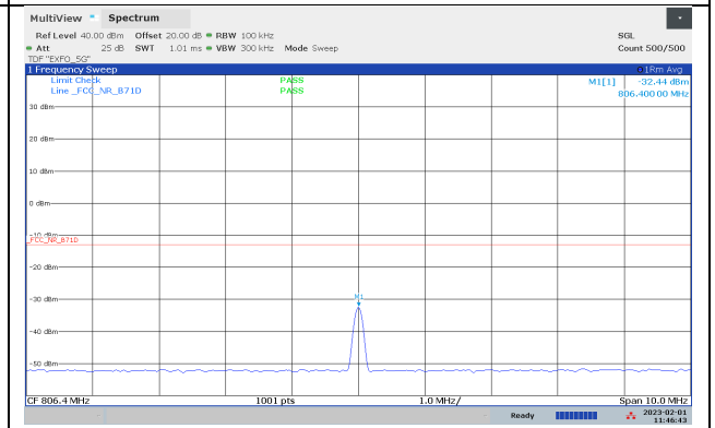
Ch126800 BW10 806.4MHz
