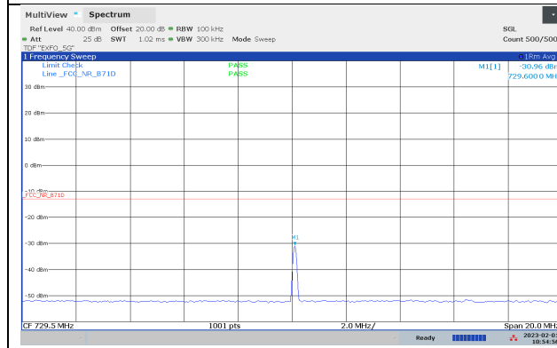
Ch126800 BW10 729.6MHz
