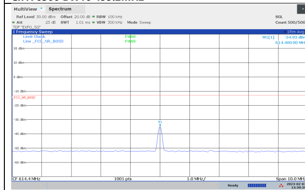
Ch176300 BW10 614.4MHz
