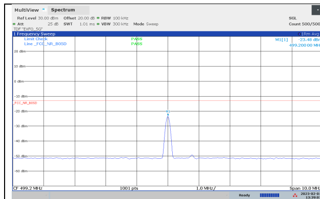
Ch176300 BW10 499.2MHz
