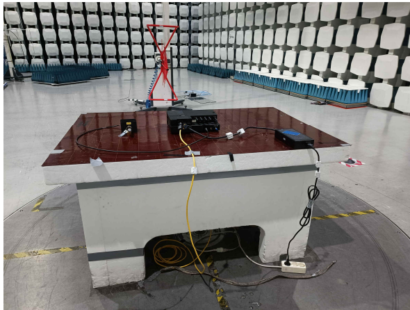
Radiated Emissions 30 – 1000 MHz, Transmitter Active
