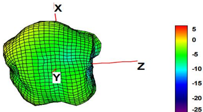
3-D Pattern Plots (2.92 dBi Max)
