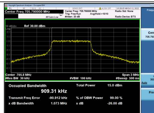
B12-5M-Mid CH-OBW-Q16
