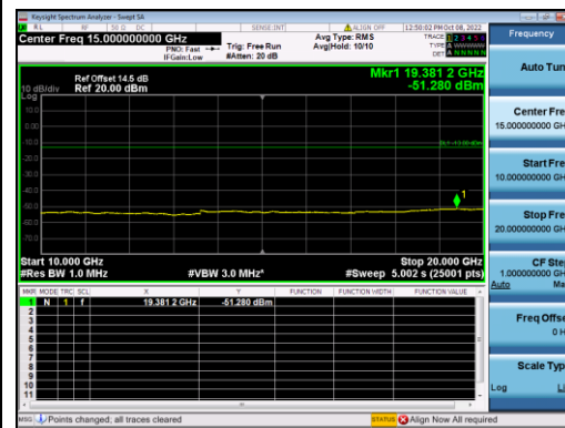
B4-3M-Low CH-CSE-2-QPSK-1 RB 0
