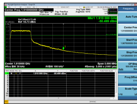
B2-20M-High CH-BE-QPSK-Full RB 0
