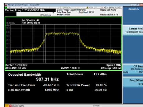
B4-1.4M-Mid CH-OBW-Q16
