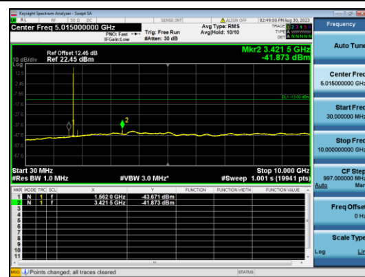
B4-10M-Mid CH-CSE-1-QPSK-1 RB 0
