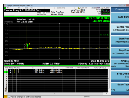
B4-5M-Mid CH-CSE-1-QPSK-1 RB 0
