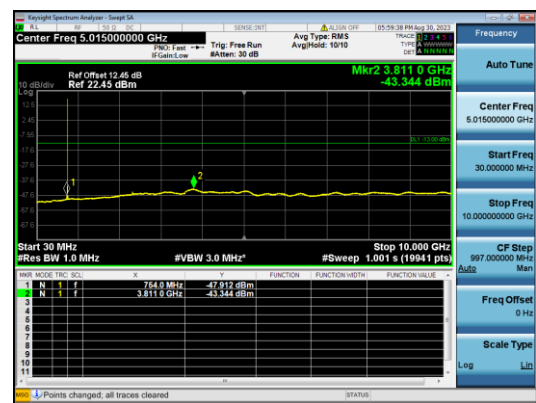
B13-10M-Low CH-CSE-1-QPSK-1 RB 0
