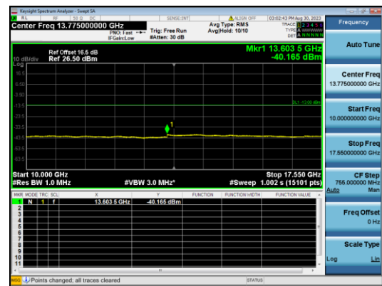
B4-10M-Low CH-CSE-2-QPSK-1 RB 0
