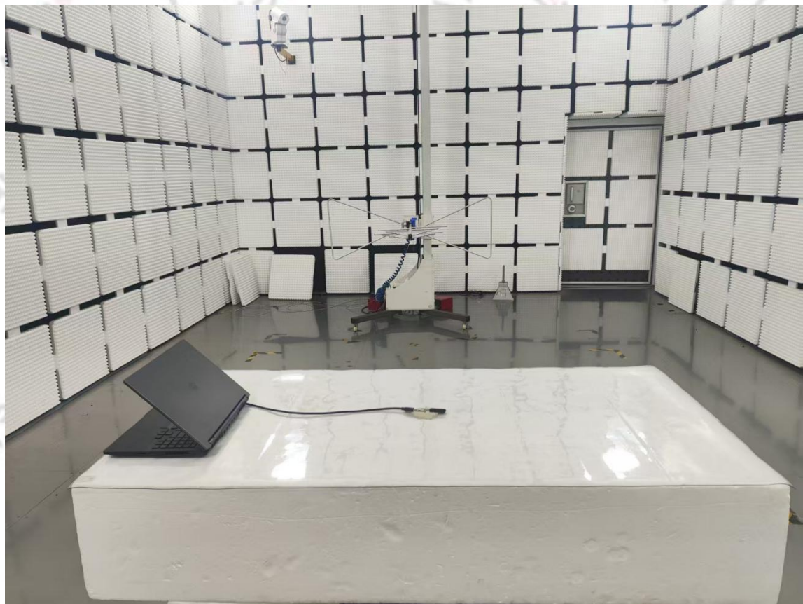
Above 1GHz
