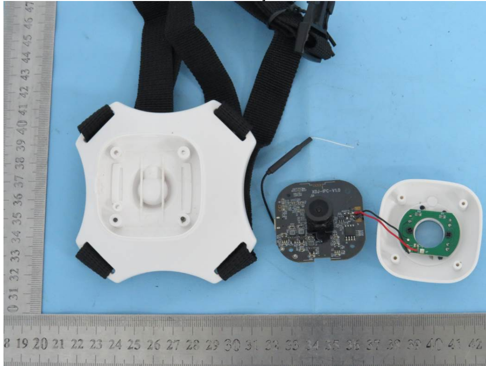
The EUT without battery– model J5045-A
