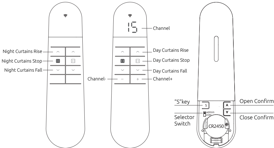
1-Channel Emitter AC2001-01D
