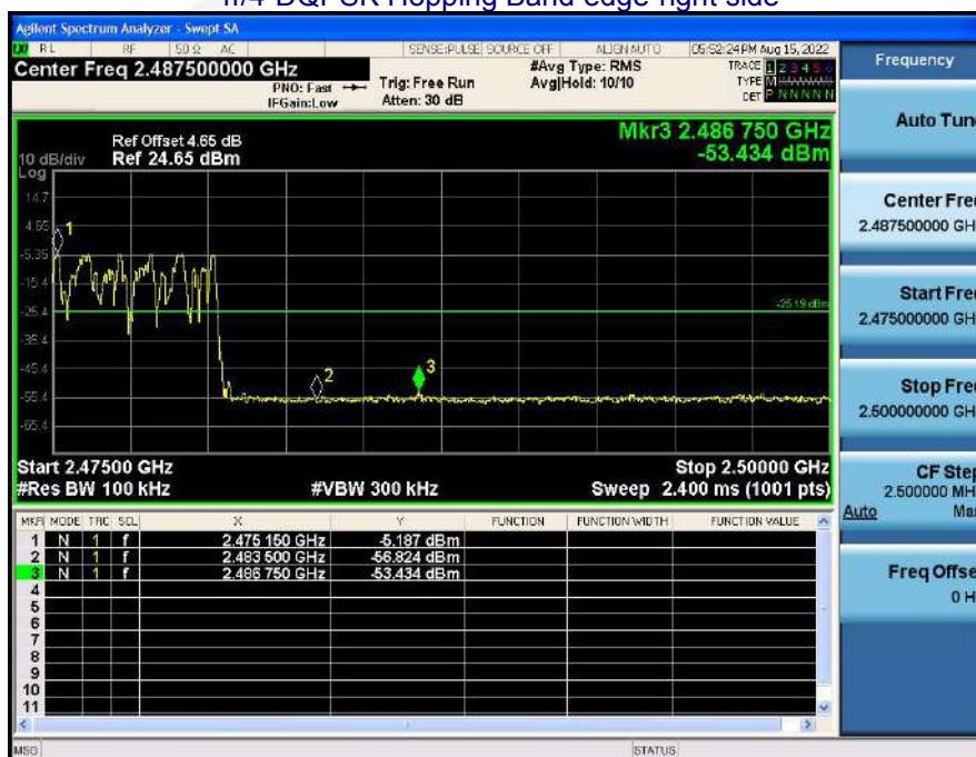
\pi/4 -DQPSK Hopping Band edge-right side
