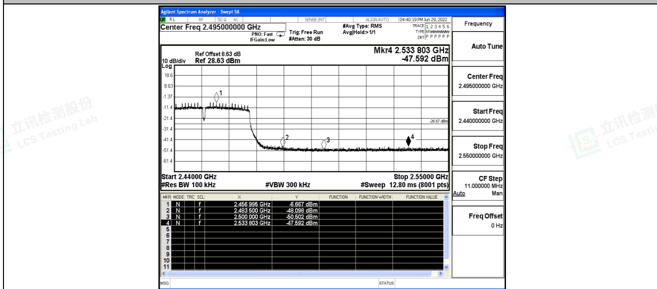
11N40SISO_Ant1_High_2452
