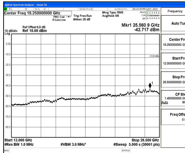
Band2-3MHz-16QAM-18615-1-0-Low-12000-26500--42.72-PASS
