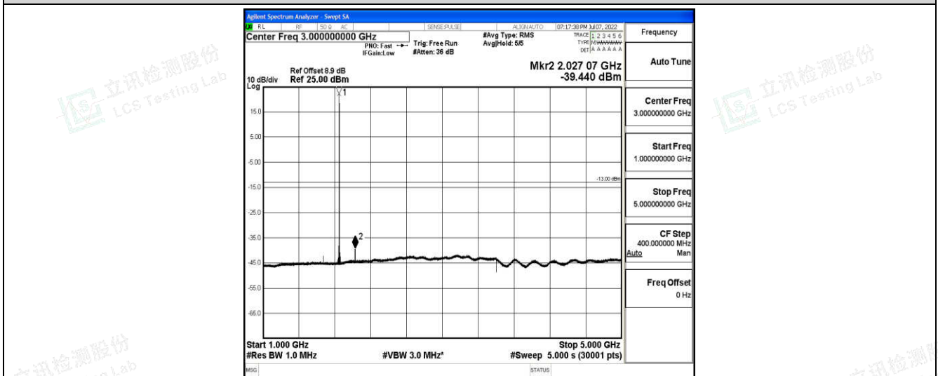
Band2-10MHz-16QAM-18650-1-0-Low-1000-5000--39.44-PASS
