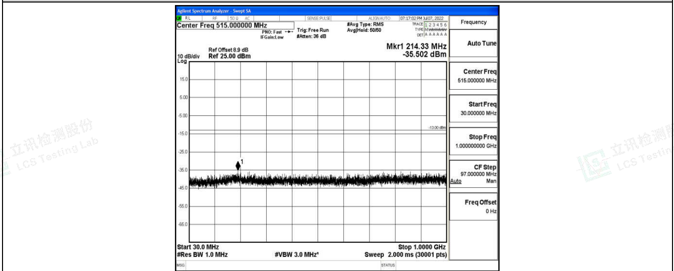
Band2-10MHz-16QAM-18650-1-0-Low-30-1000--35.5-PASS
