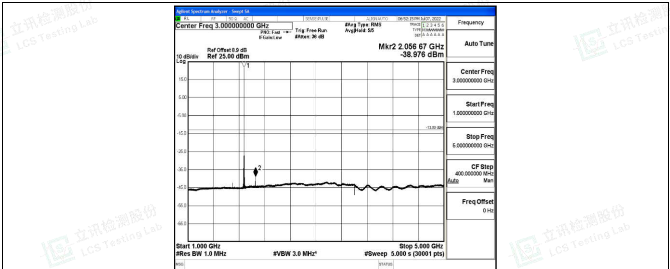
Band2-5MHz-QPSK-18900-1-0-Low-1000-5000--38.98-PASS
