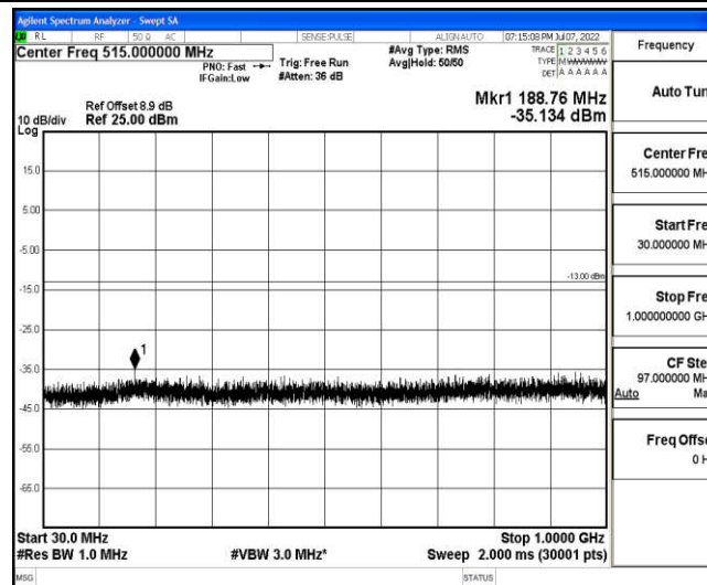
Band2-10MHz-QPSK-18650-1-0-Low-30-1000--35.13-PASS
