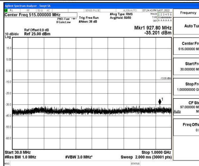
Band2-10MHz-16QAM-19150-1-0-High-30-1000--35.2-PASS
