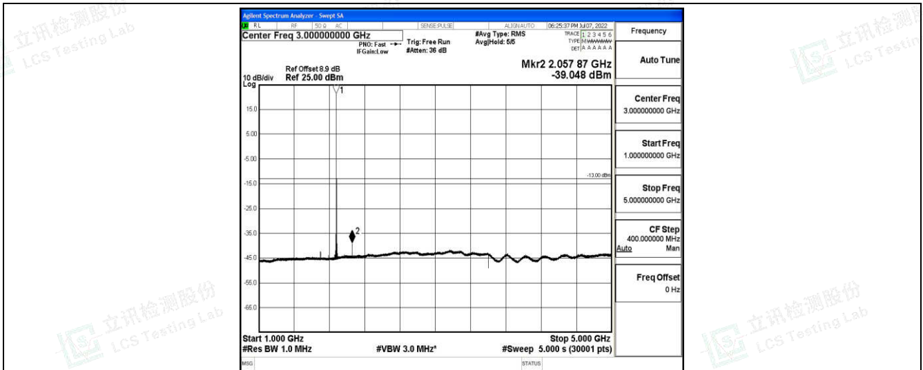
Band2-3MHz-QPSK-18900-1-0-Low-1000-5000--39.05-PASS
