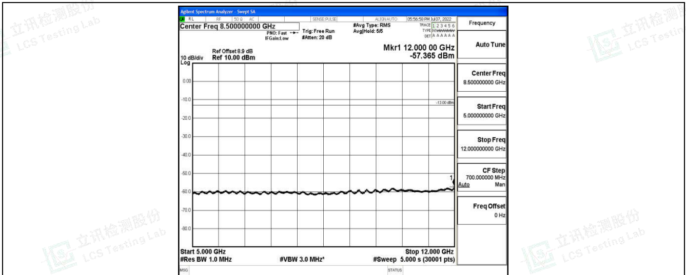
Band2-1.4MHz-16QAM-18607-1-0-Low-5000-12000--57.37-PASS
