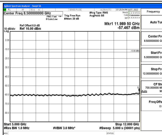
Band2-10MHz-16QAM-19150-1-0-High-5000-12000--57.47-PASS
