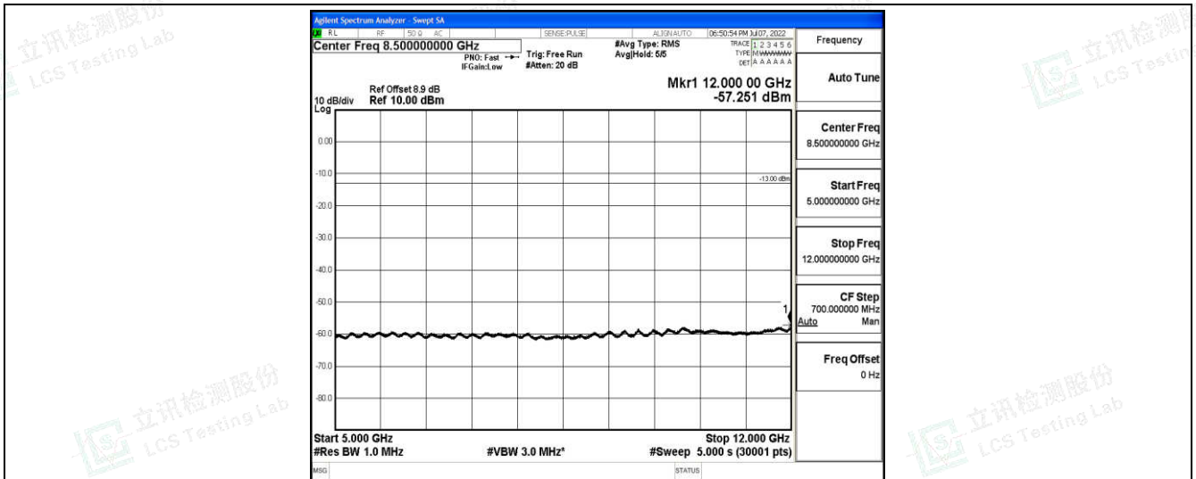
Band2-5MHz-16QAM-18625-1-0-Low-5000-12000--57.25-PASS
