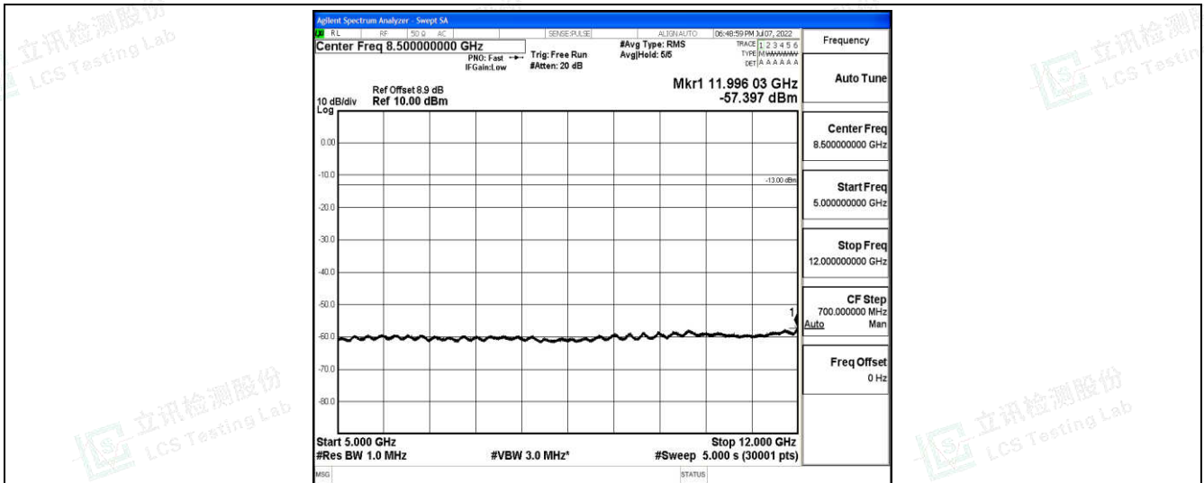
Band2-5MHz-QPSK-18625-1-0-Low-5000-12000--57.4-PASS
