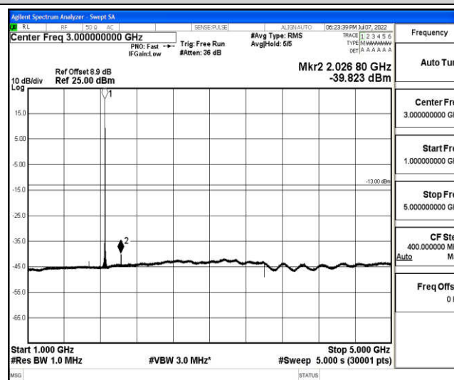
Band2-3MHz-16QAM-18615-1-0-Low-1000-5000--39.82-PASS
