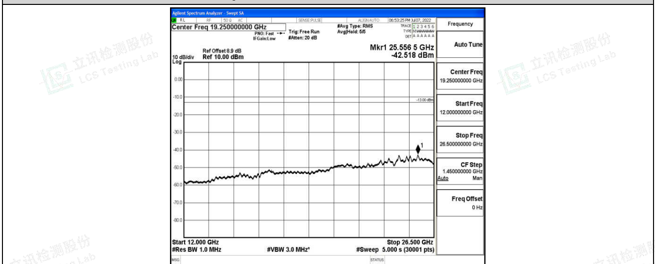
Band2-5MHz-QPSK-18900-1-0-Low-12000-26500--42.52-PASS
