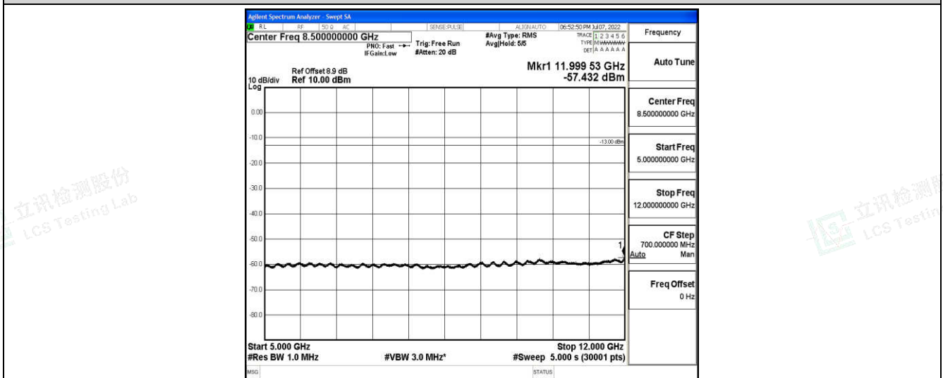
Band2-5MHz-QPSK-18900-1-0-Low-5000-12000--57.43-PASS
