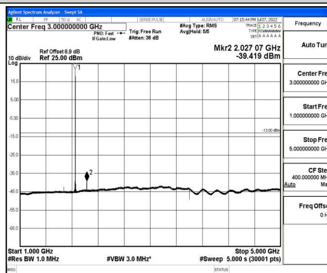
Band2-10MHz-QPSK-18650-1-0-Low-1000-5000--39.42-PASS
