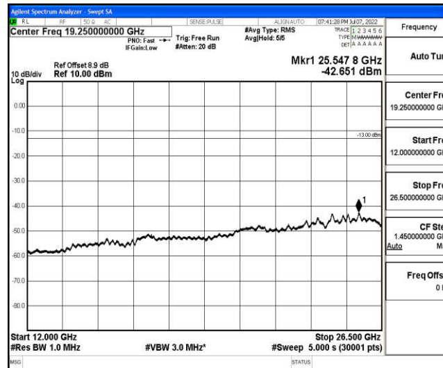
Band2-15MHz-QPSK-18675-1-0-Low-12000-26500--42.65-PASS
