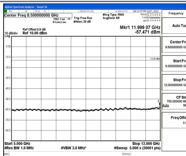
Band2-3MHz-16QAM-19185-1-0-High-5000-12000--57.47-PASS
