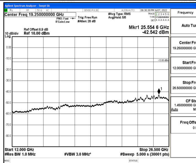
Band2-3MHz-QPSK-19185-1-0-High-12000-26500--42.54-PASS
