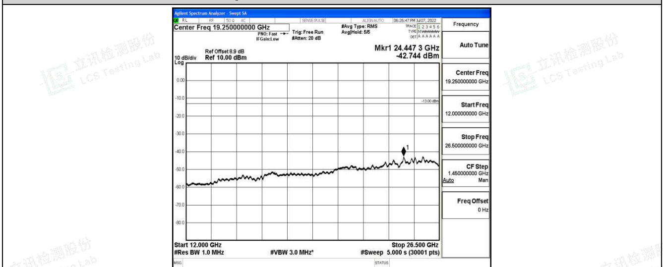
Band2-3MHz-QPSK-18900-1-0-Low-12000-26500--42.74-PASS
