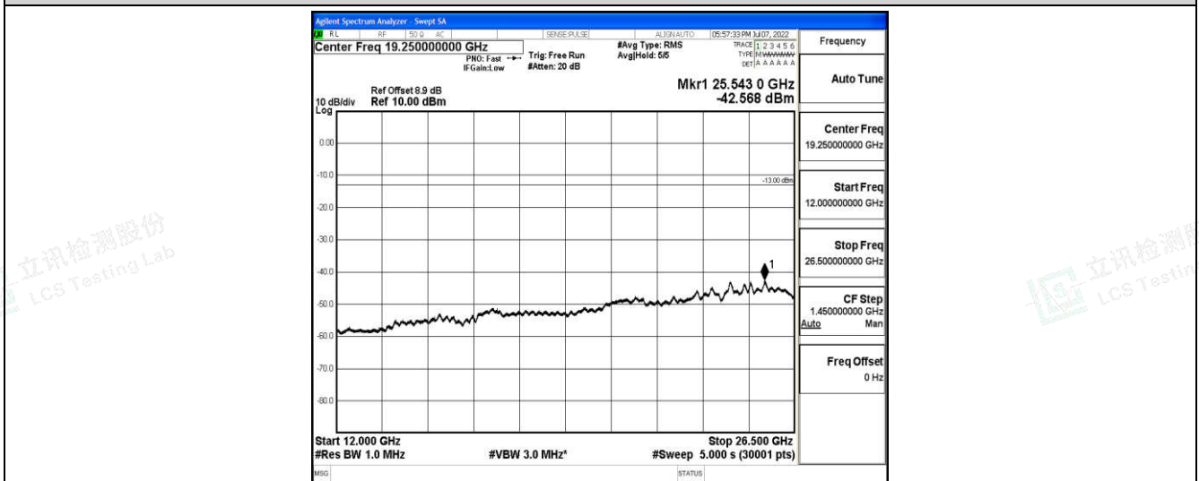
Band2-1.4MHz-16QAM-18607-1-0-Low-12000-26500--42.57-PASS
