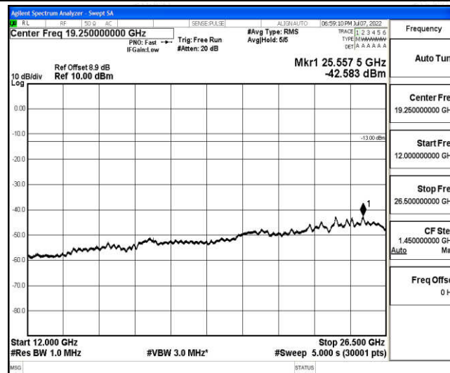
Band2-5MHz-16QAM-19175-1-0-High-12000-26500--42.58-PASS
