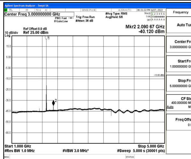
Band2-3MHz-16QAM-19185-1-0-High-1000-5000--40.12-PASS
