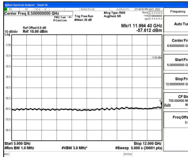
Band2-15MHz-QPSK-18675-1-0-Low-5000-12000--57.61-PASS
