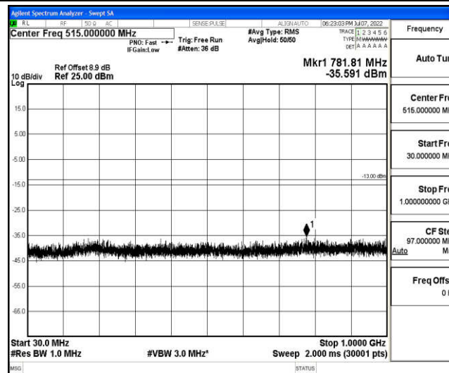
Band2-3MHz-16QAM-18615-1-0-Low-30-1000--35.59-PASS
