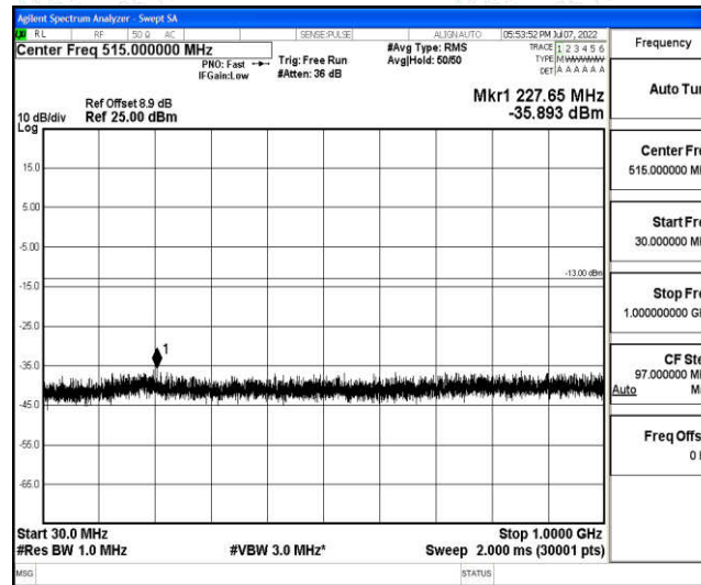
Band2-1.4MHz-QPSK-18607-1-0-Low-30-1000--35.89-PASS
