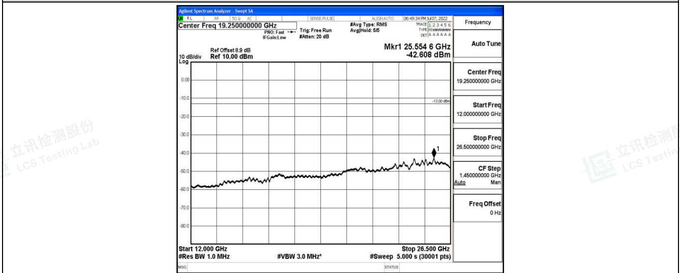
Band2-5MHz-QPSK-18625-1-0-Low-12000-26500--42.61-PASS
