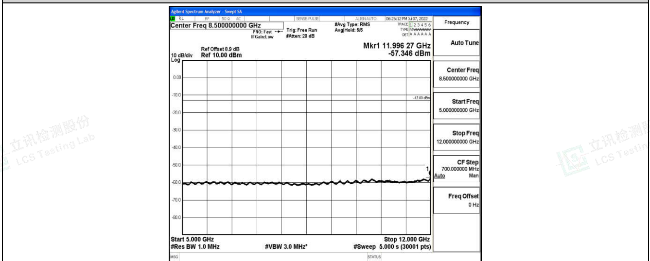
Band2-3MHz-QPSK-18900-1-0-Low-5000-12000--57.35-PASS
