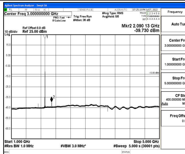
Band2-10MHz-16QAM-19150-1-0-High-1000-5000--39.73-PASS
