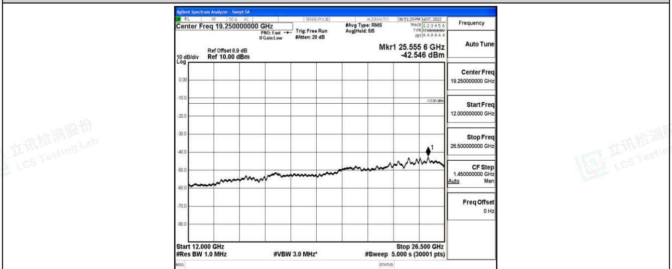
Band2-5MHz-16QAM-18625-1-0-Low-12000-26500--42.55-PASS
