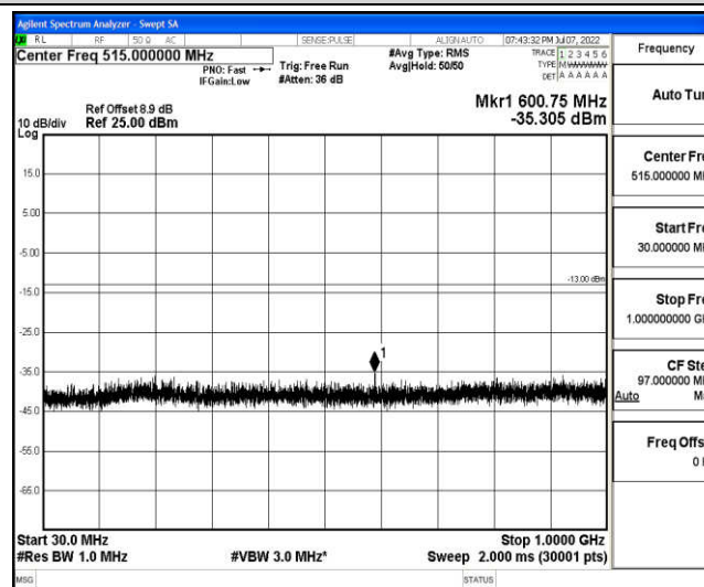
Band2-15MHz-QPSK-18900-1-0-Low-30-1000--35.31-PASS
