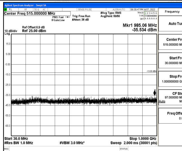
Band2-3MHz-16QAM-19185-1-0-High-30-1000--35.53-PASS
