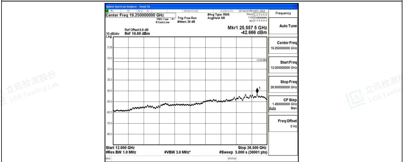
Band2-15MHz-16QAM-18675-1-0-Low-12000-26500--42.67-PASS
