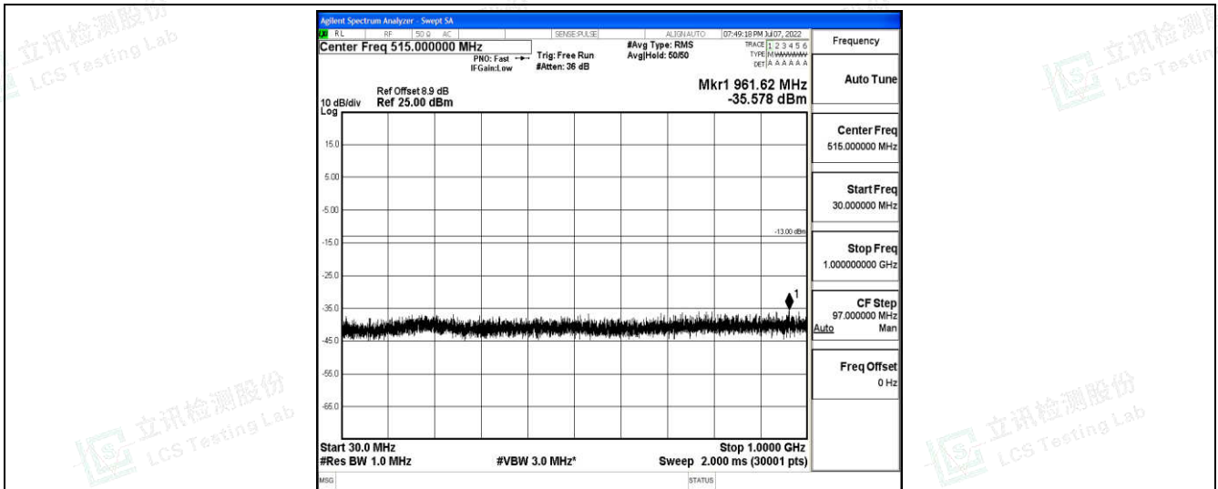
Band2-15MHz-16QAM-19125-1-0-High-30-1000--35.58-PASS
