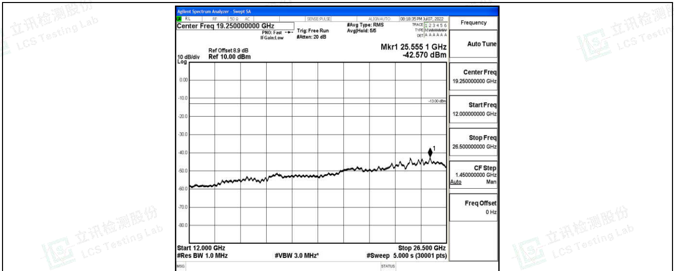
Band2-20MHz-QPSK-19100-1-0-High-12000-26500--42.57-PASS
