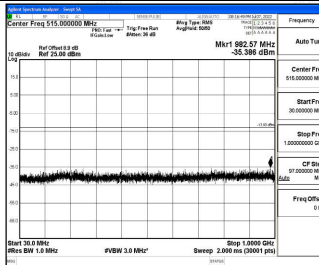
Band2-20MHz-QPSK-19100-1-0-High-30-1000--35.39-PASS
