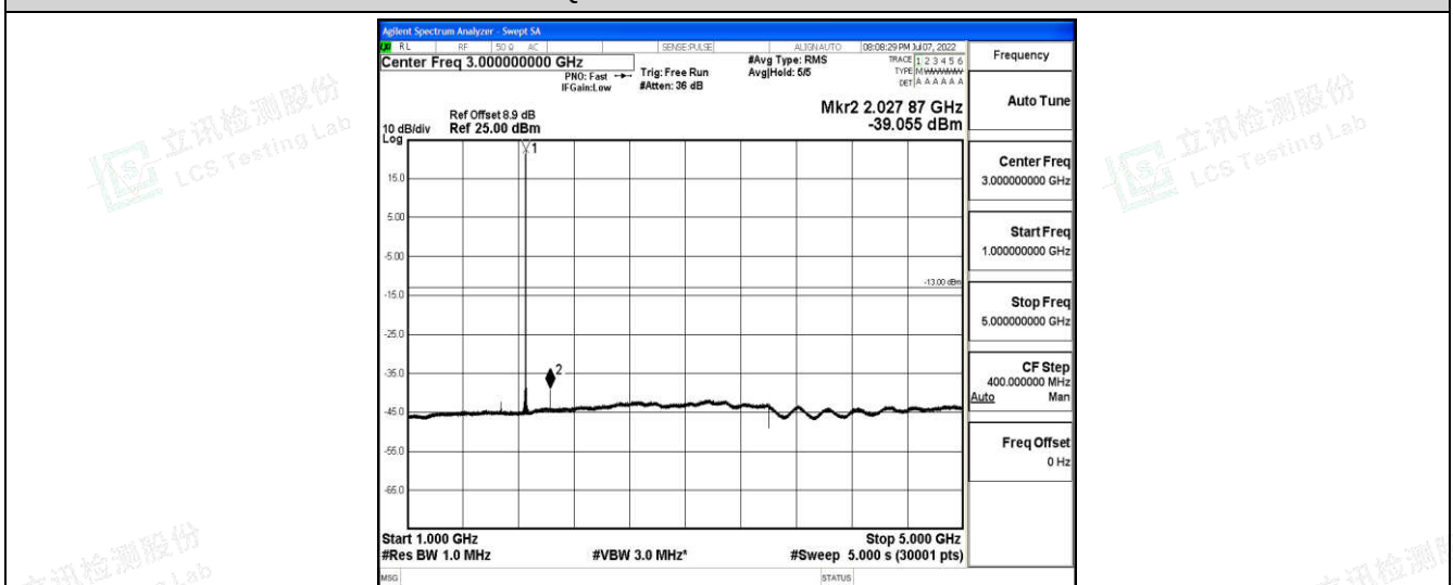
Band2-20MHz-16QAM-18700-1-0-Low-1000-5000--39.06-PASS
