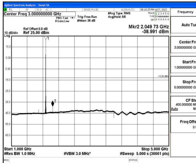
Band2-20MHz-QPSK-18900-1-0-Low-1000-5000--38.99-PASS
