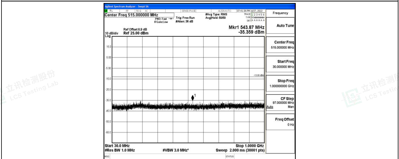
Band2-15MHz-16QAM-18675-1-0-Low-30-1000--35.36-PASS
