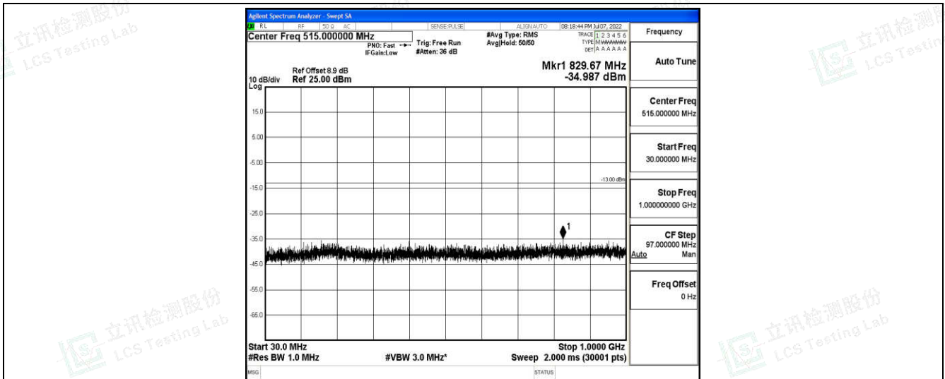
Band2-20MHz-16QAM-19100-1-0-High-30-1000--34.99-PASS
