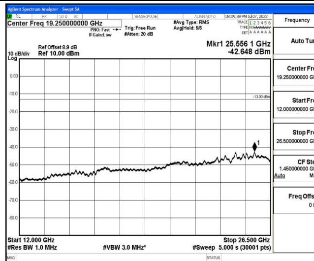
Band2-20MHz-16QAM-18700-1-0-Low-12000-26500--42.65-PASS
