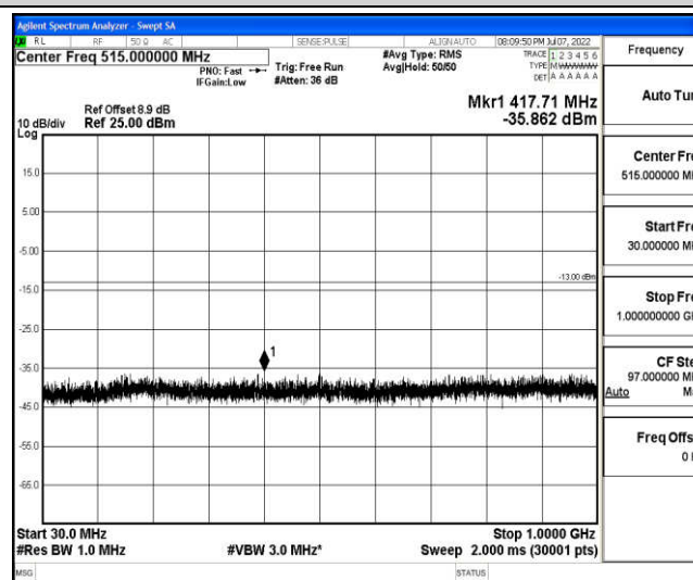
Band2-20MHz-QPSK-18900-1-0-Low-30-1000--35.86-PASS
