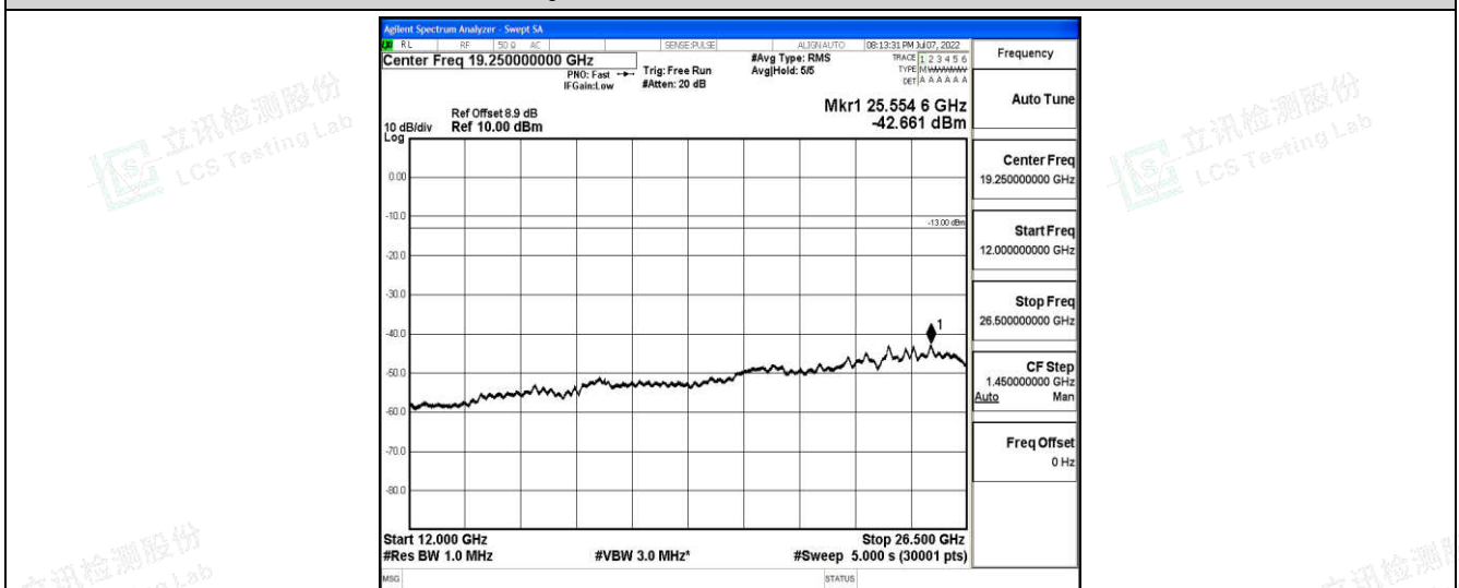
Band2-20MHz-16QAM-18900-1-0-Low-12000-26500--42.66-PASS
