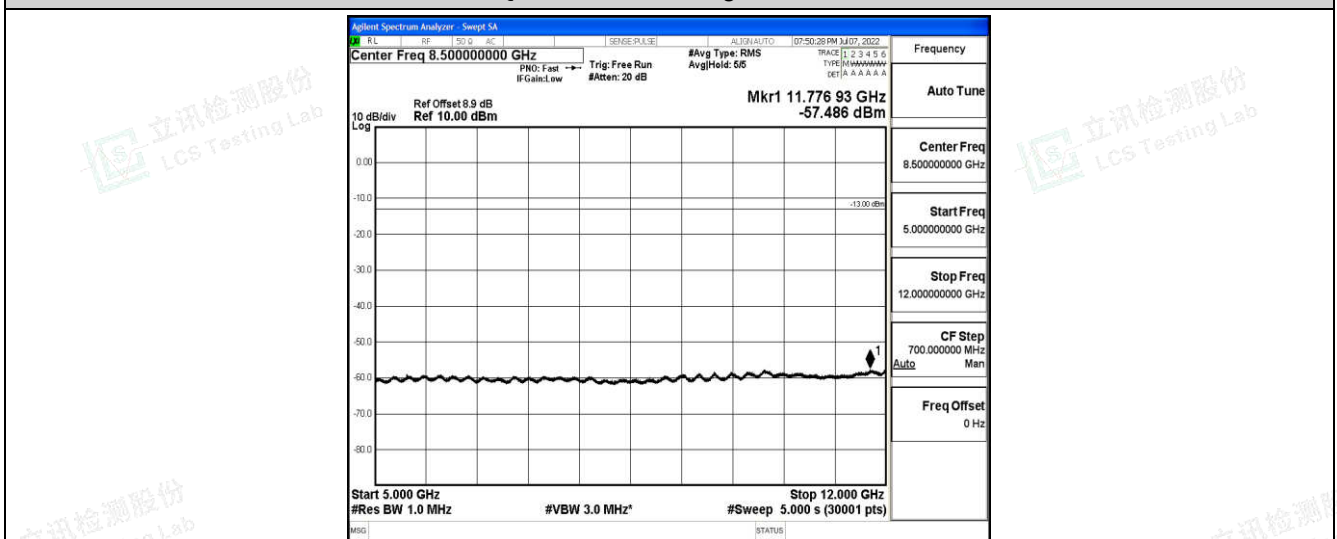
Band2-15MHz-16QAM-19125-1-0-High-5000-12000--57.49-PASS
