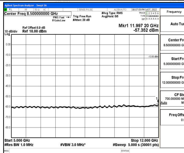
Band2-20MHz-QPSK-18700-1-0-Low-5000-12000--57.35-PASS
