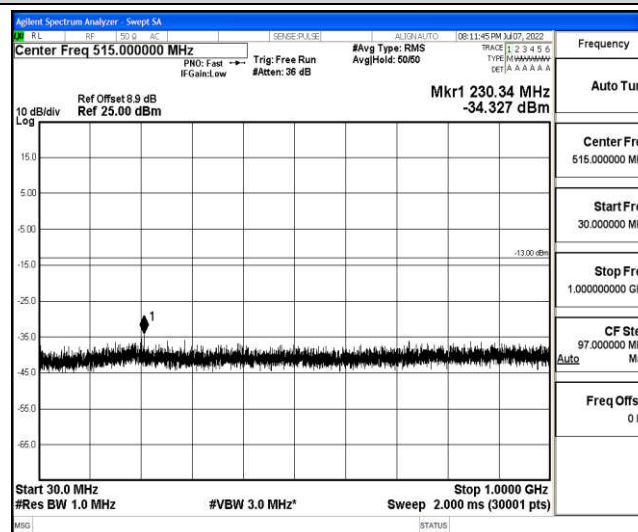
Band2-20MHz-16QAM-18900-1-0-Low-30-1000--34.33-PASS
