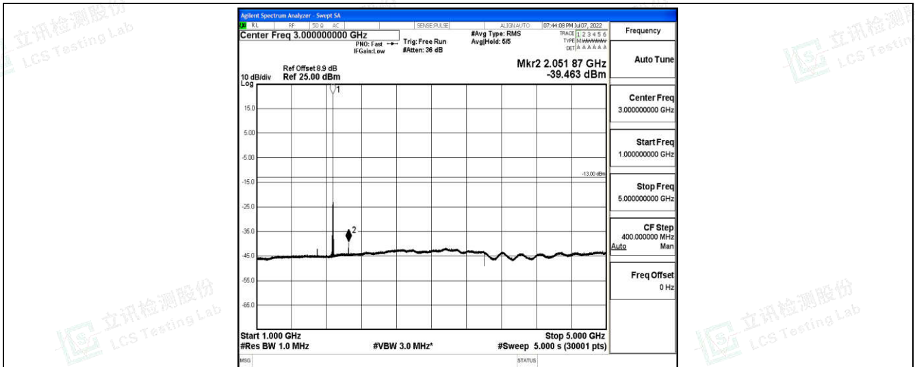
Band2-15MHz-QPSK-18900-1-0-Low-1000-5000--39.46-PASS
