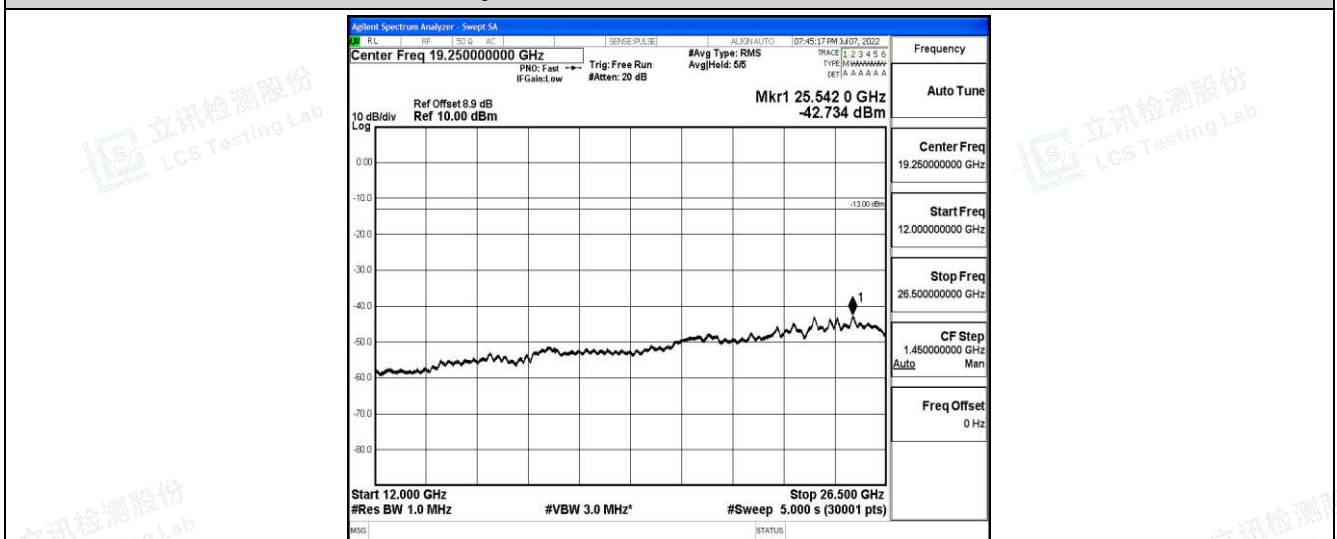
Band2-15MHz-QPSK-18900-1-0-Low-12000-26500--42.73-PASS
