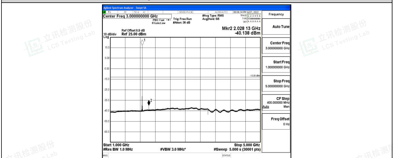
Band2-20MHz-QPSK-18700-1-0-Low-1000-5000--40.14-PASS
