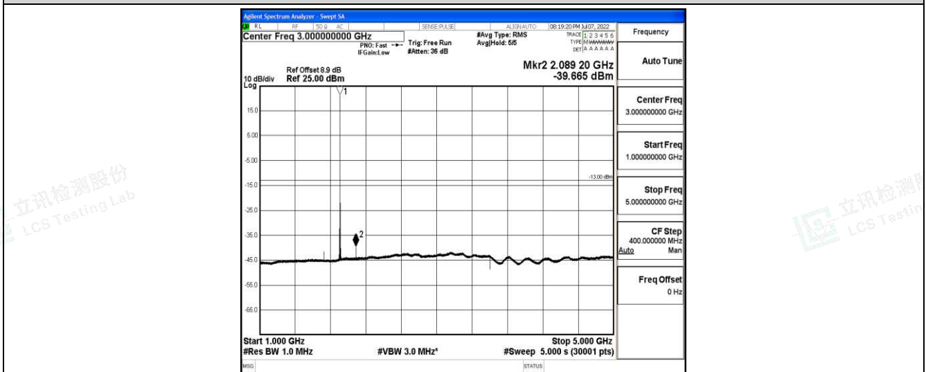
Band2-20MHz-16QAM-19100-1-0-High-1000-5000--39.67-PASS
