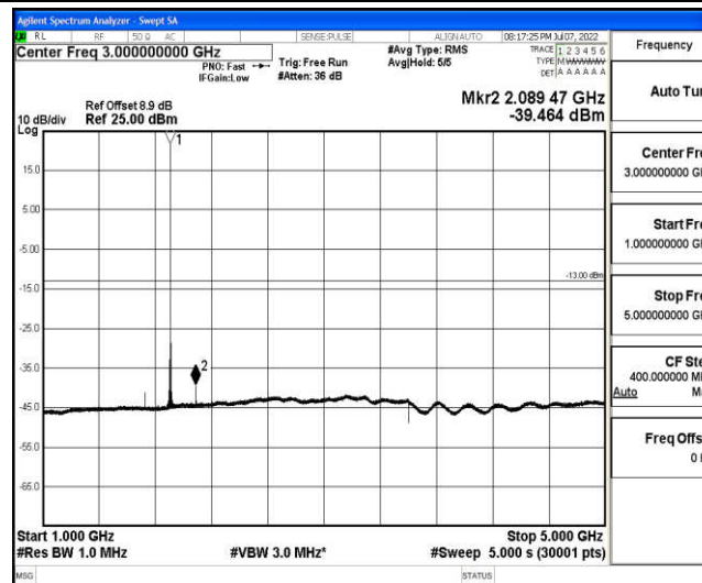
Band2-20MHz-QPSK-19100-1-0-High-1000-5000--39.46-PASS
