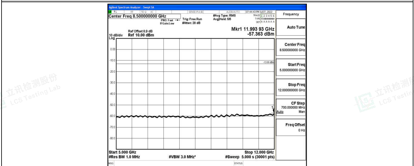
Band2-15MHz-QPSK-18900-1-0-Low-5000-12000--57.36-PASS
