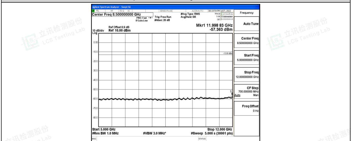
Band2-20MHz-16QAM-19100-1-0-High-5000-12000--57.36-PASS
