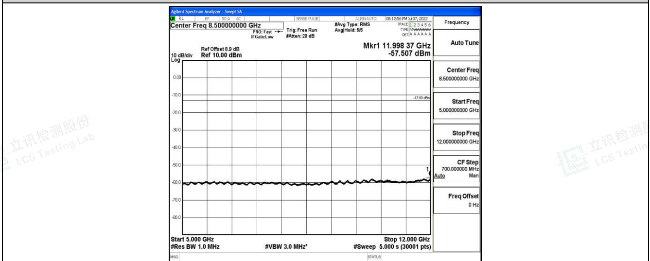
Band2-20MHz-16QAM-18900-1-0-Low-5000-12000--57.51-PASS
