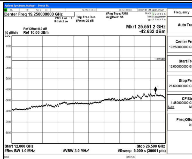
Band2-20MHz-QPSK-18700-1-0-Low-12000-26500--42.63-PASS
