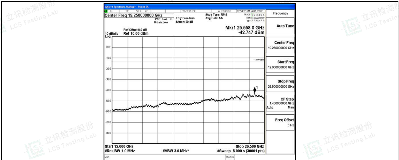
Band2-15MHz-16QAM-19125-1-0-High-12000-26500--42.75-PASS
