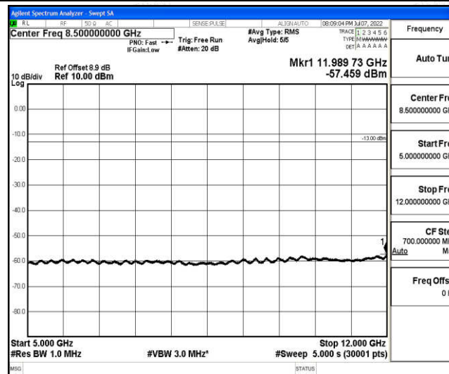
Band2-20MHz-16QAM-18700-1-0-Low-5000-12000--57.46-PASS
