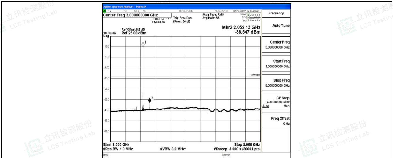
Band2-15MHz-16QAM-18900-1-0-Low-1000-5000--38.55-PASS
