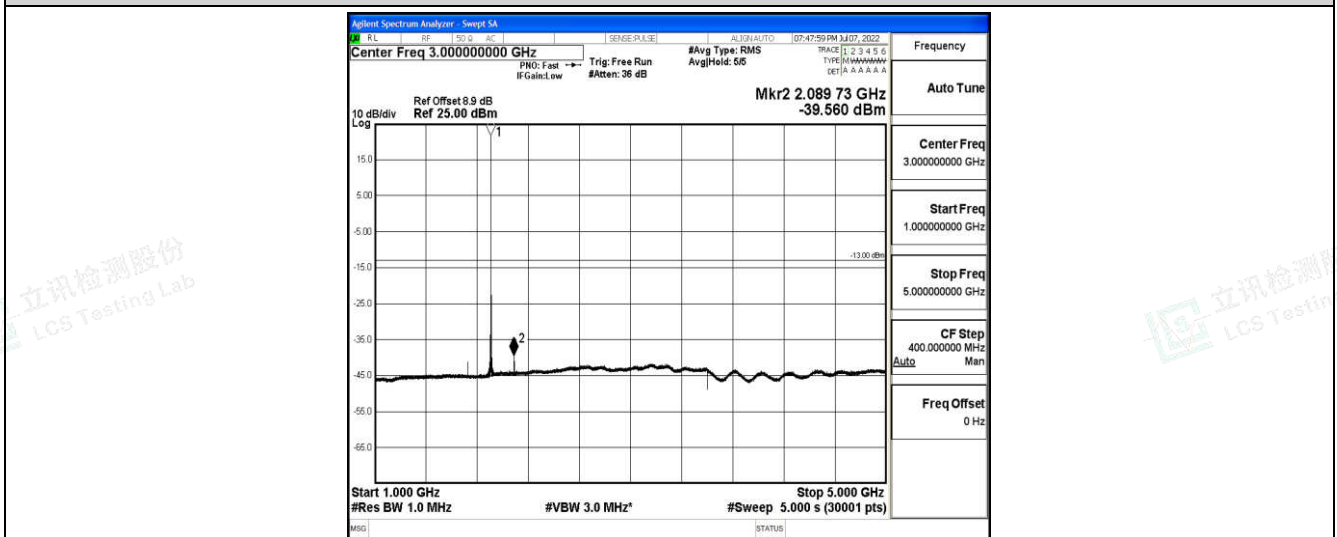
Band2-15MHz-QPSK-19125-1-0-High-1000-5000--39.56-PASS
