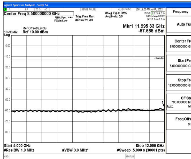
Band2-20MHz-QPSK-18900-1-0-Low-5000-12000--57.59-PASS
