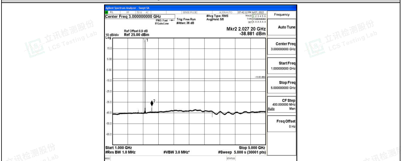
Band2-15MHz-16QAM-18675-1-0-Low-1000-5000--38.88-PASS
