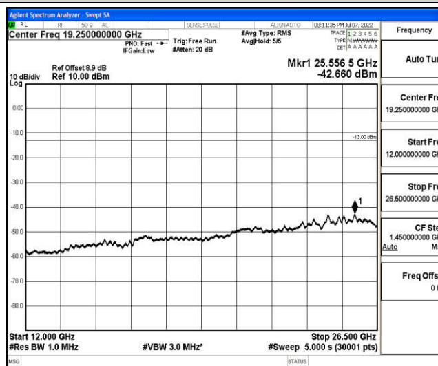
Band2-20MHz-QPSK-18900-1-0-Low-12000-26500--42.66-PASS
