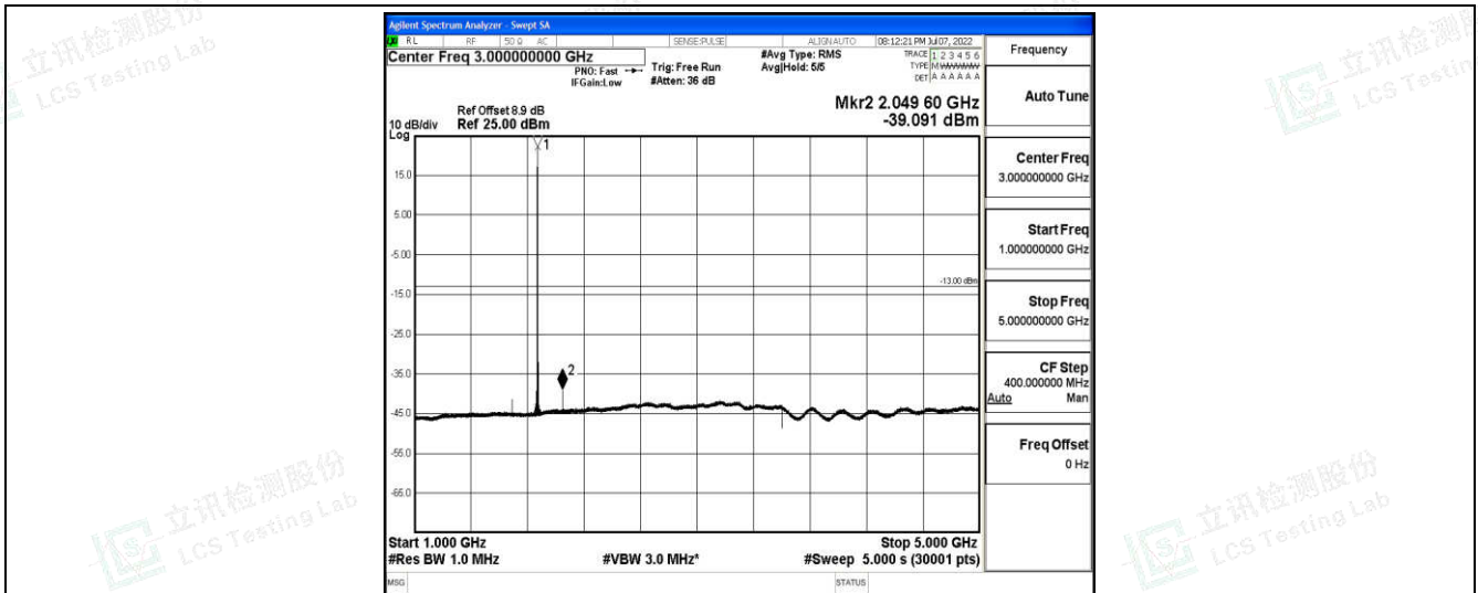
Band2-20MHz-16QAM-18900-1-0-Low-1000-5000--39.09-PASS
