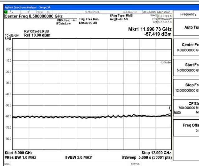
Band2-20MHz-QPSK-19100-1-0-High-5000-12000--57.42-PASS
