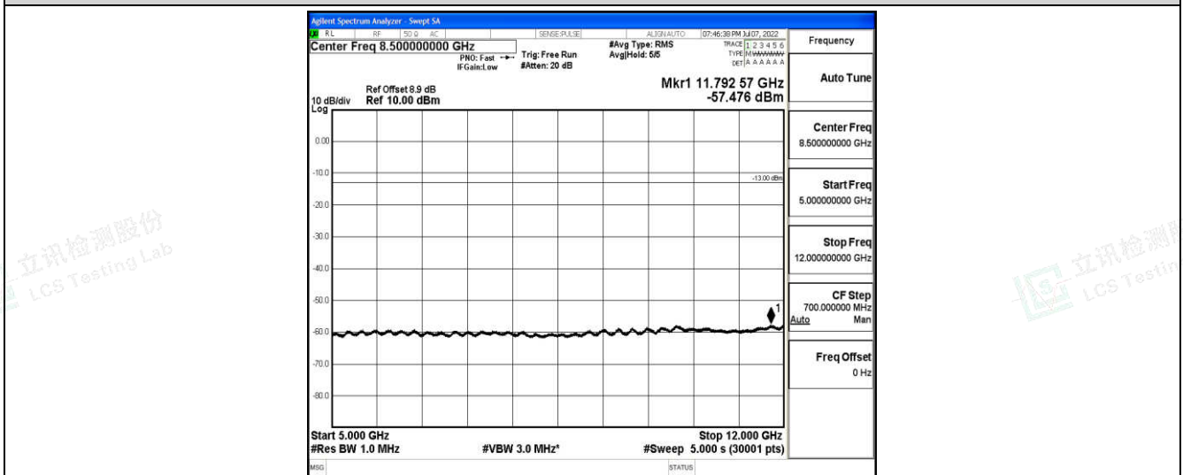
Band2-15MHz-16QAM-18900-1-0-Low-5000-12000--57.48-PASS
