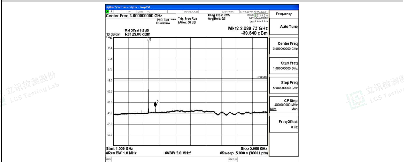
Band2-15MHz-16QAM-19125-1-0-High-1000-5000--39.54-PASS
