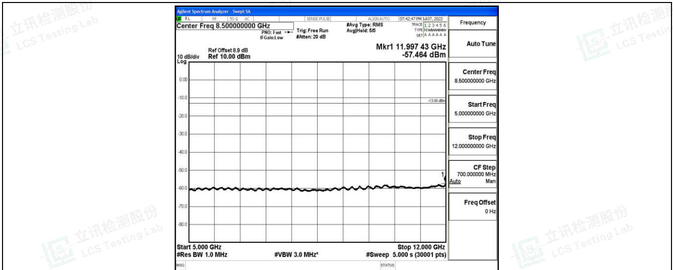
Band2-15MHz-16QAM-18675-1-0-Low-5000-12000--57.46-PASS
