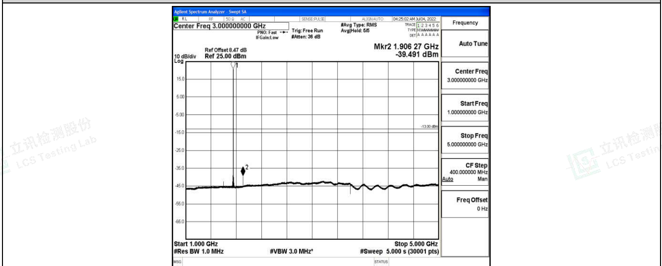
Band4-3MHz-QPSK-20385-1-0-High-1000-5000--39.49-PASS
