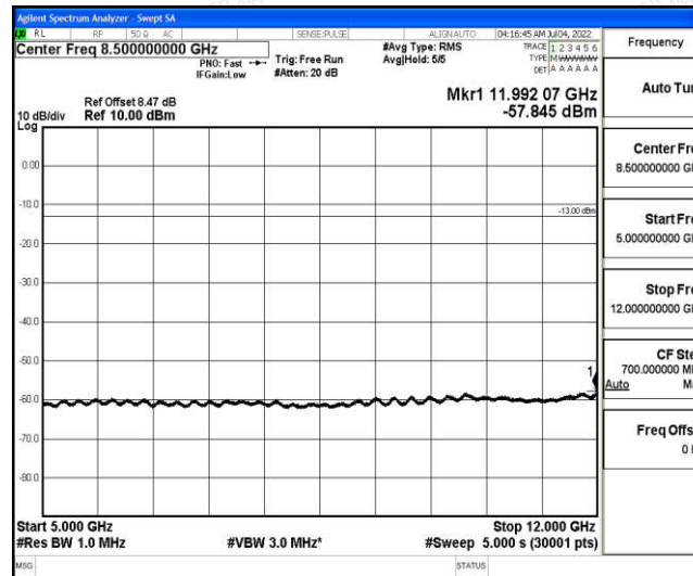
Band4-3MHz-QPSK-19965-1-0-Low-5000-12000--57.85-PASS
