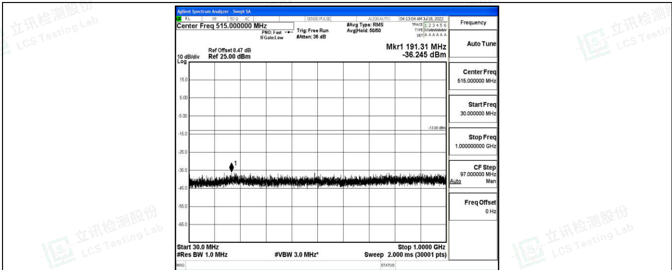
Band4-3MHz-16QAM-20385-1-0-High-30-1000--36.25-PASS
