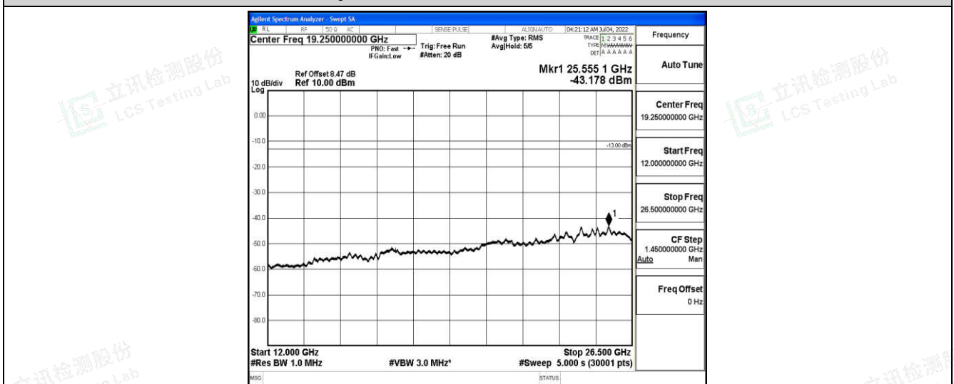
Band4-3MHz-QPSK-20175-1-0-Low-12000-26500--43.18-PASS
