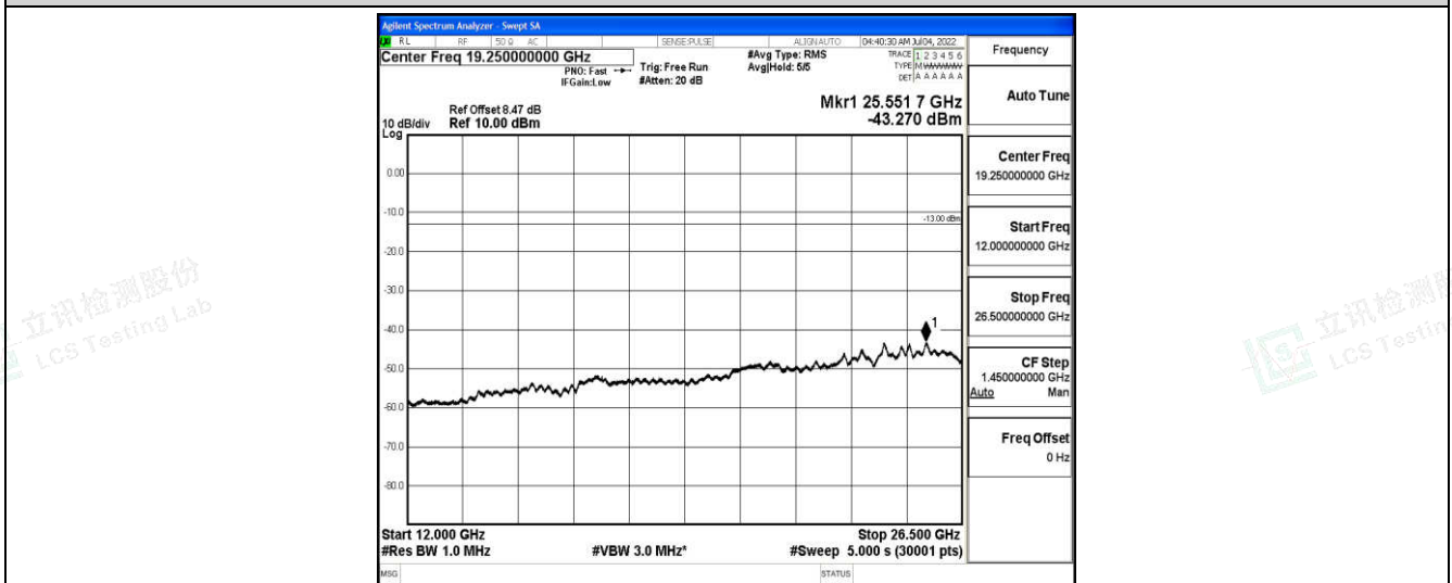
Band4-5MHz-16QAM-19975-1-0-Low-12000-26500--43.27-PASS
