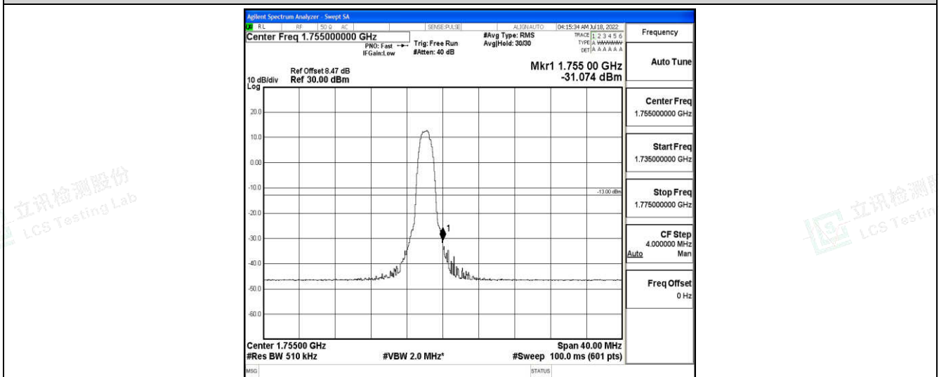
Band4-20MHz-QPSK-20300-6-0-High--31.07-PASS
