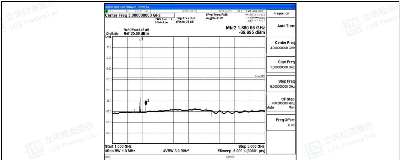
Band4-5MHz-QPSK-20175-1-0-Low-1000-5000--39.7-PASS
