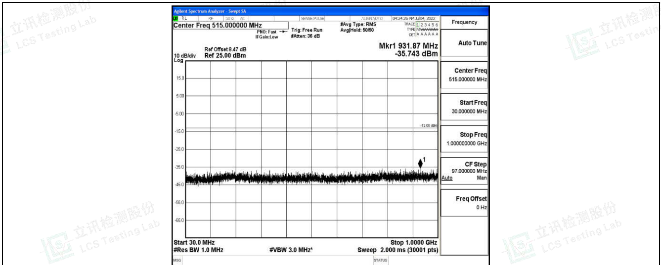
Band4-3MHz-QPSK-20385-1-0-High-30-1000--35.74-PASS
