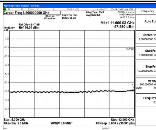
Band4-1.4MHz-QPSK-20393-1-0-High-5000-12000--57.98-PASS
