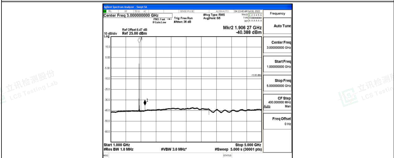
Band4-3MHz-16QAM-20385-1-0-High-1000-5000--40.39-PASS
