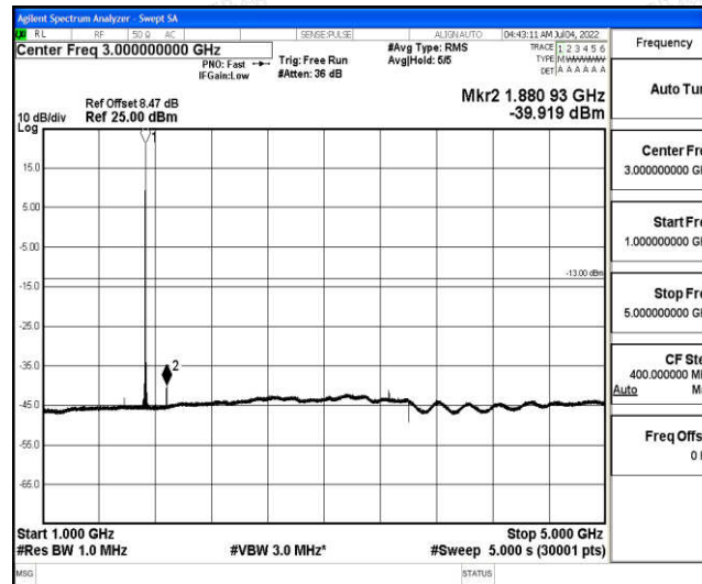
Band4-5MHz-16QAM-20175-1-0-Low-1000-5000--39.92-PASS
