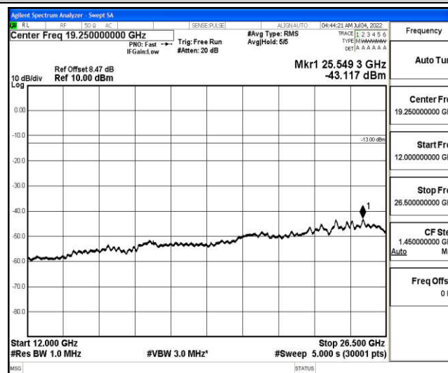
Band4-5MHz-16QAM-20175-1-0-Low-12000-26500--43.12-PASS
