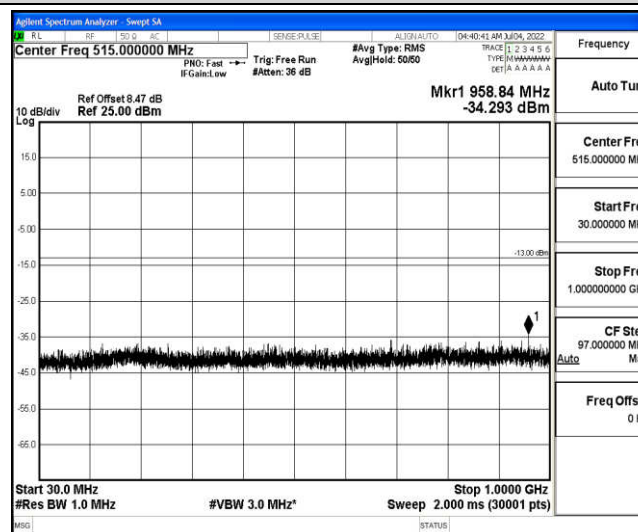
Band4-5MHz-QPSK-20175-1-0-Low-30-1000--34.29-PASS
