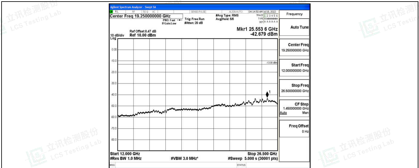
Band4-3MHz-16QAM-20385-1-0-High-12000-26500--42.68-PASS
