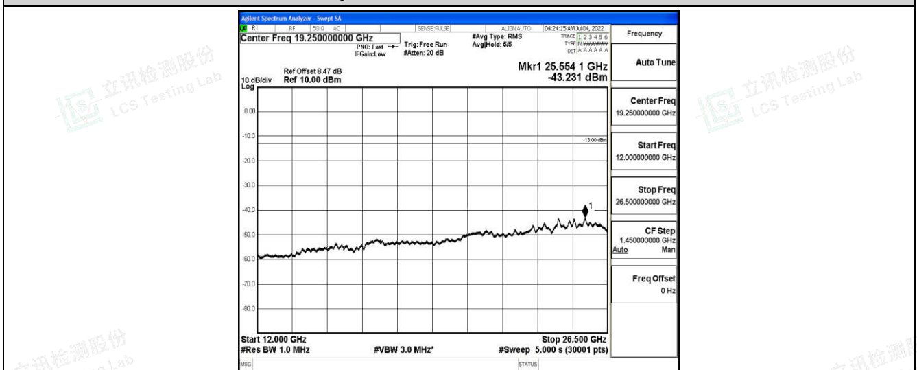
Band4-3MHz-16QAM-20175-1-0-Low-12000-26500--43.23-PASS
