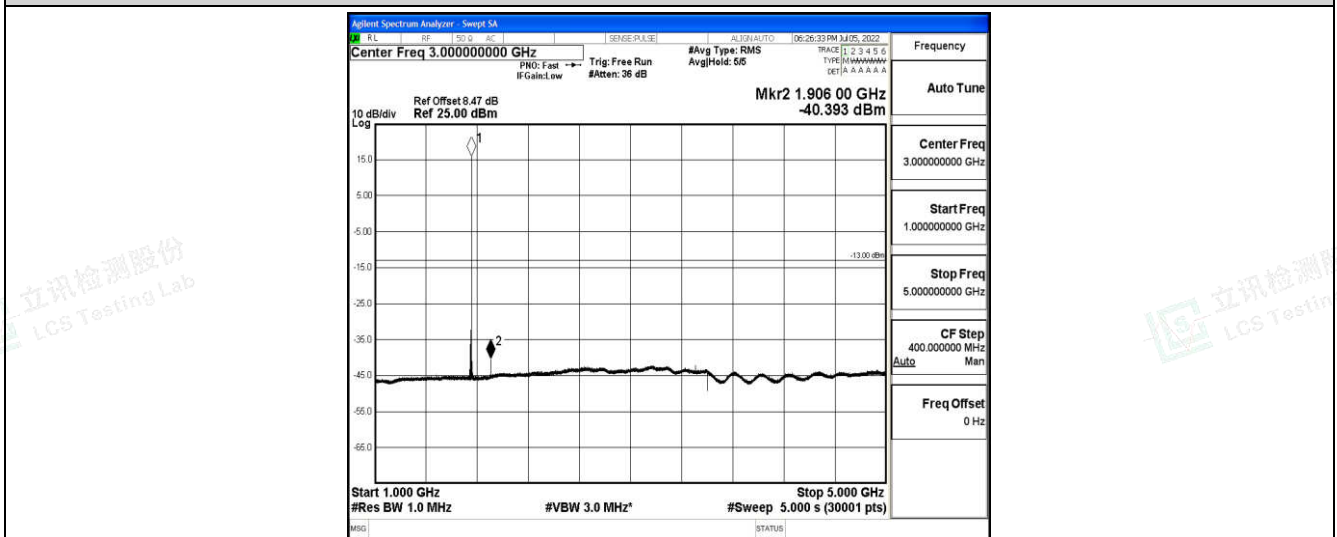
Band4-10MHz-QPSK-20350-1-0-High-1000-5000--40.39-PASS
