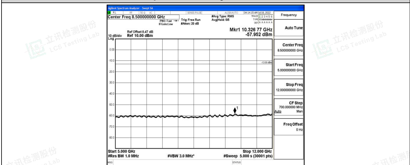
Band4-3MHz-16QAM-20385-1-0-High-5000-12000--57.95-PASS
