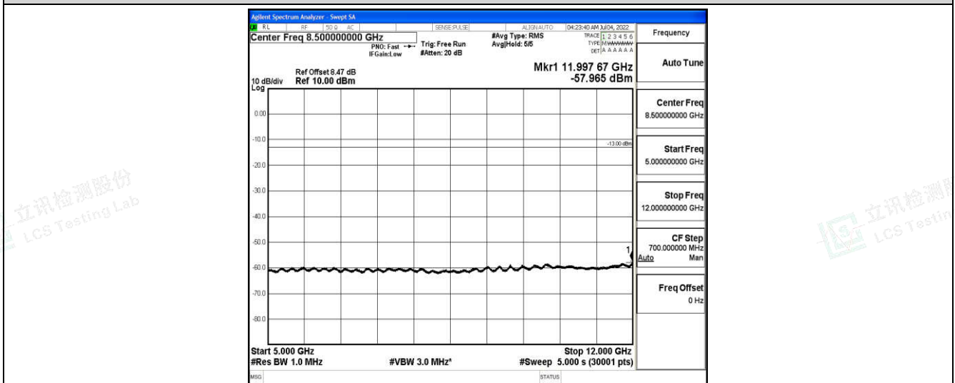
Band4-3MHz-16QAM-20175-1-0-Low-5000-12000--57.97-PASS
