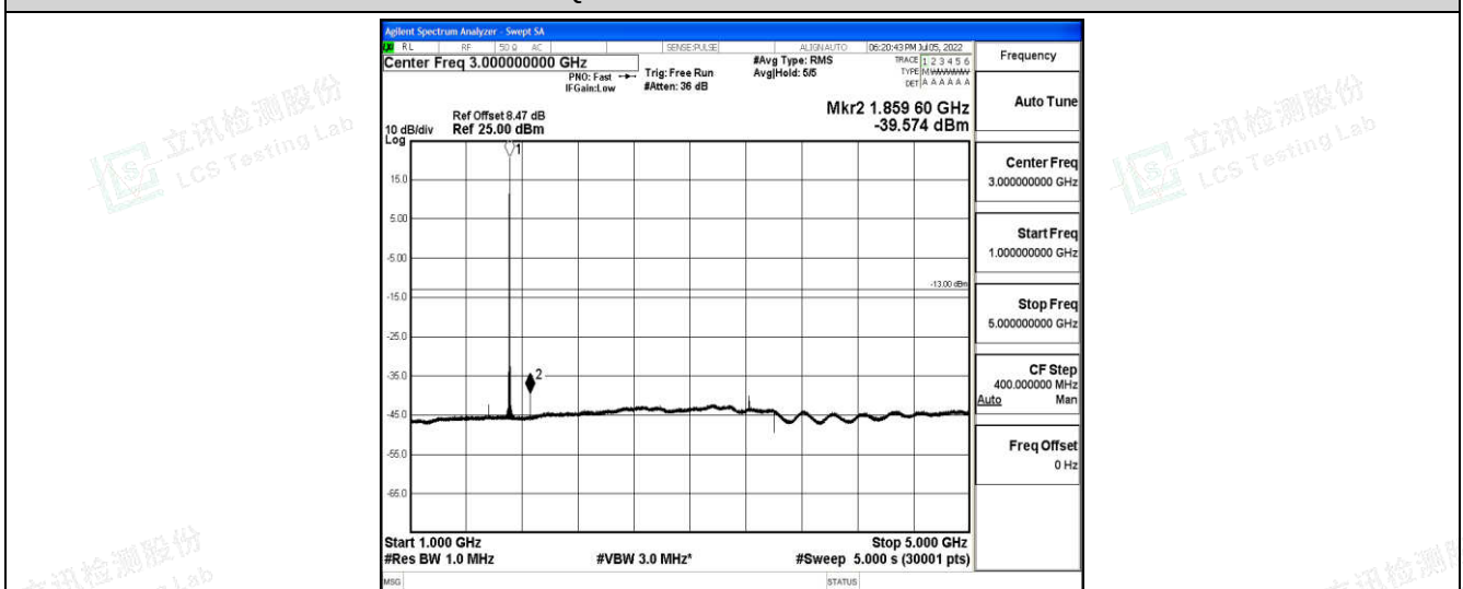
Band4-10MHz-16QAM-20000-1-0-Low-1000-5000--39.57-PASS
