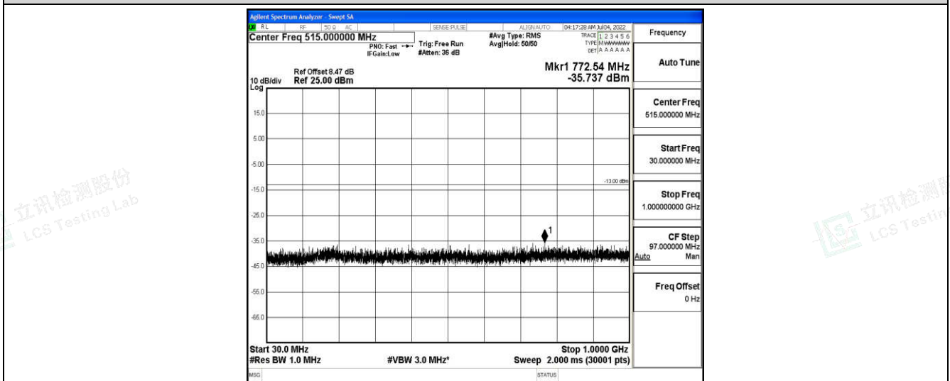
Band4-3MHz-16QAM-19965-1-0-Low-30-1000--35.74-PASS
