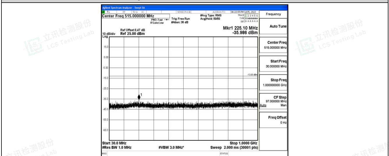
Band4-10MHz-QPSK-20175-1-0-Low-30-1000--35.99-PASS
