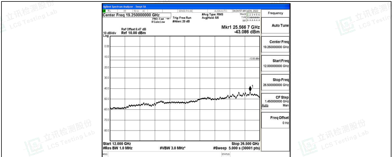
Band4-1.4MHz-QPSK-20393-1-0-High-12000-26500--43.09-PASS
