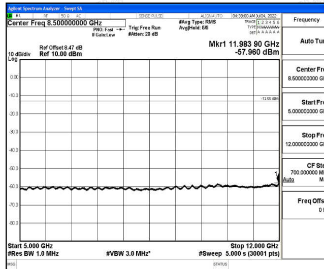
Band4-5MHz-QPSK-19975-1-0-Low-5000-12000--57.96-PASS
