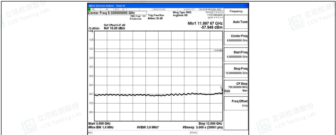
Band4-3MHz-16QAM-19965-1-0-Low-5000-12000--57.95-PASS
