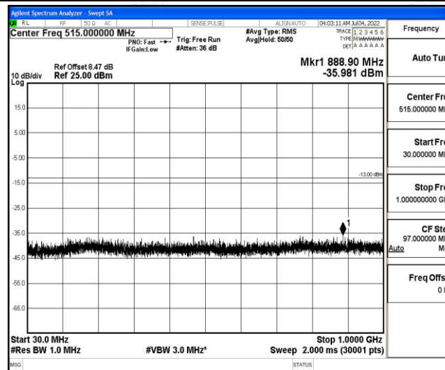
Band4-1.4MHz-QPSK-20393-1-0-High-30-1000--35.98-PASS
