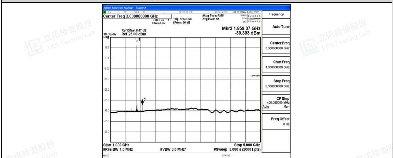
Band4-5MHz-16QAM-19975-1-0-Low-1000-5000--39.39-PASS
