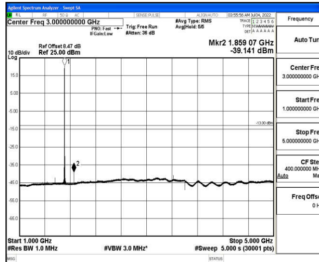
Band4-1.4MHz-QPSK-19957-1-0-Low-1000-5000--39.14-PASS
