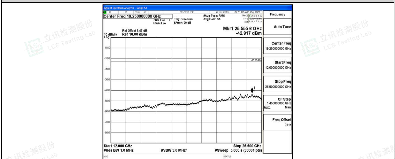
Band4-1.4MHz-QPSK-20175-1-0-Low-12000-26500--42.92-PASS
