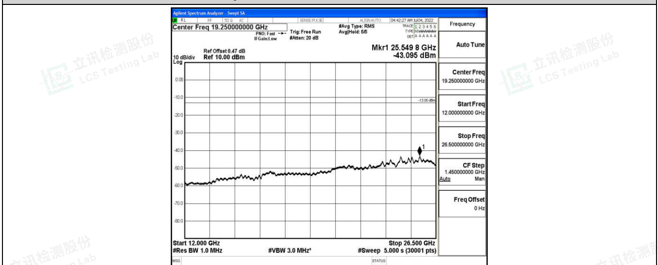
Band4-5MHz-QPSK-20175-1-0-Low-12000-26500--43.1-PASS
