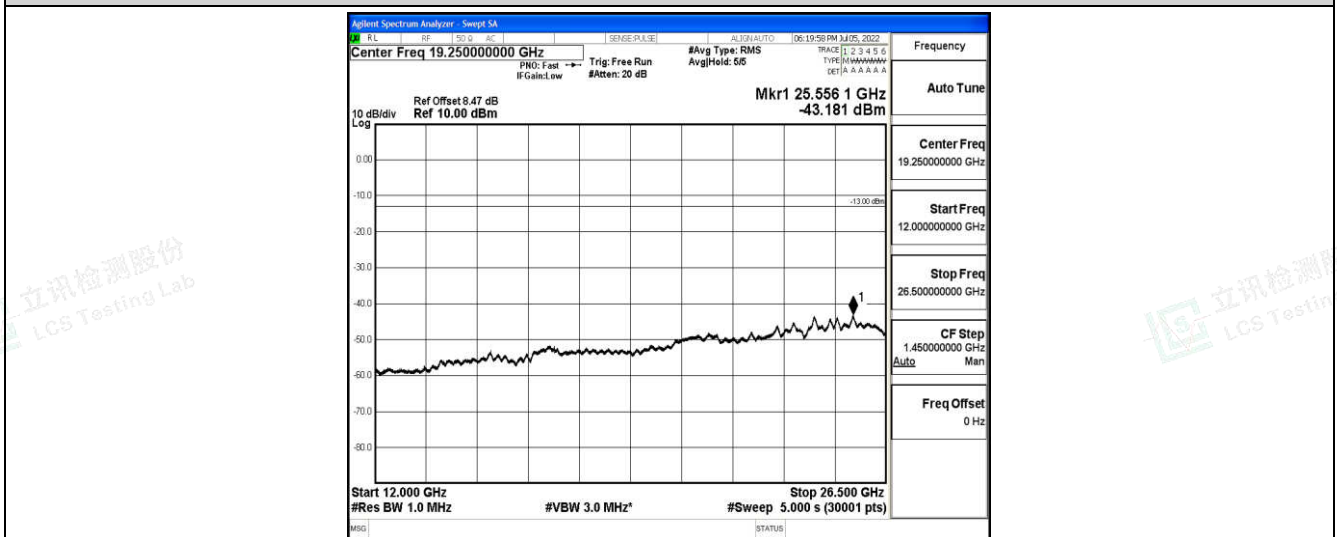
Band4-10MHz-QPSK-20000-1-0-Low-12000-26500--43.18-PASS
