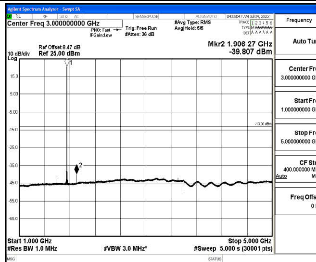
Band4-1.4MHz-QPSK-20393-1-0-High-1000-5000--39.81-PASS
