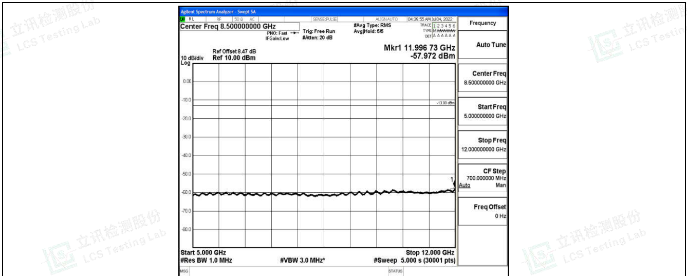
Band4-5MHz-16QAM-19975-1-0-Low-5000-12000--57.97-PASS
