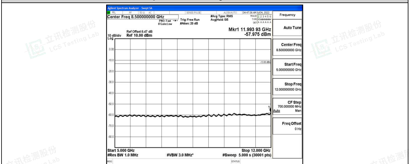
Band4-5MHz-16QAM-20375-1-0-High-5000-12000--57.98-PASS
