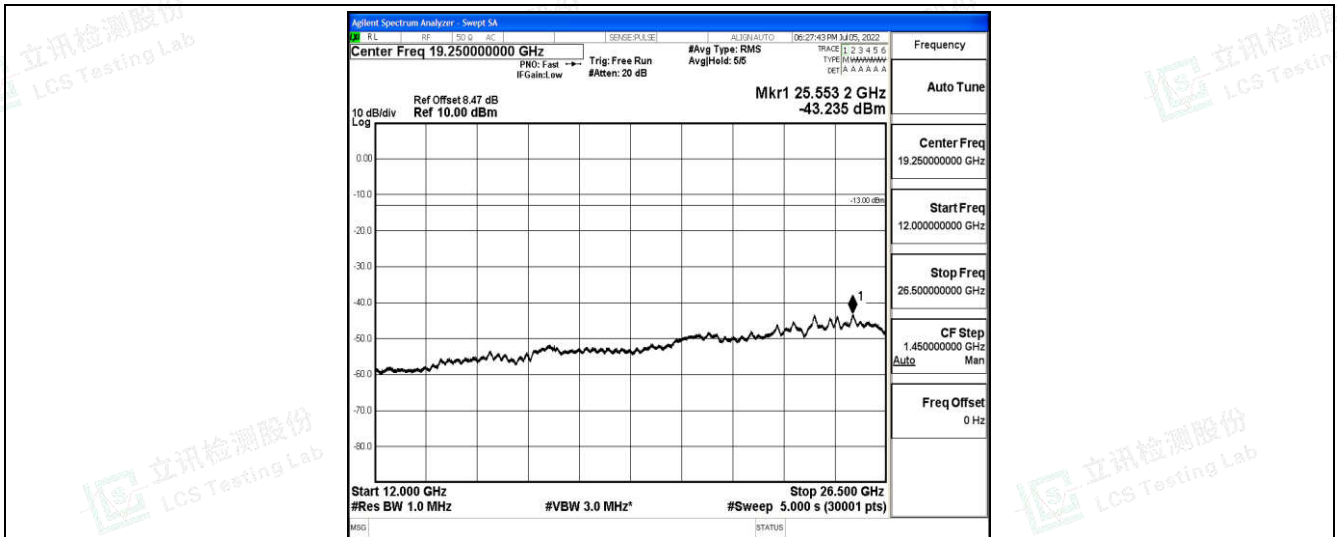
Band4-10MHz-QPSK-20350-1-0-High-12000-26500--43.24-PASS
