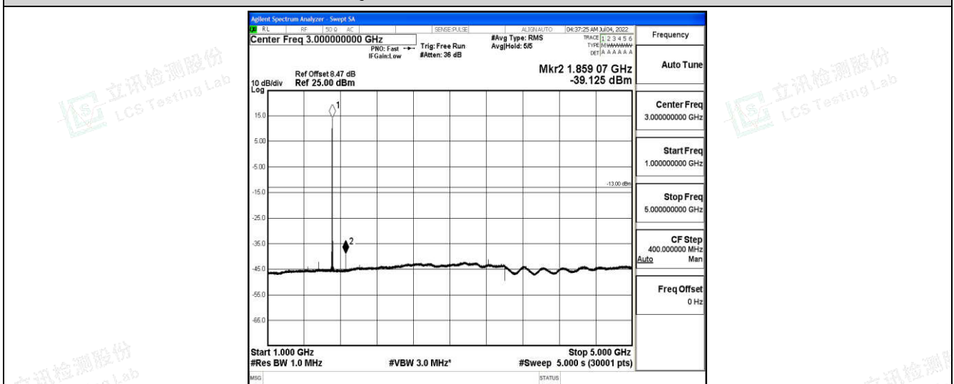
Band4-5MHz-QPSK-19975-1-0-Low-1000-5000--39.13-PASS
