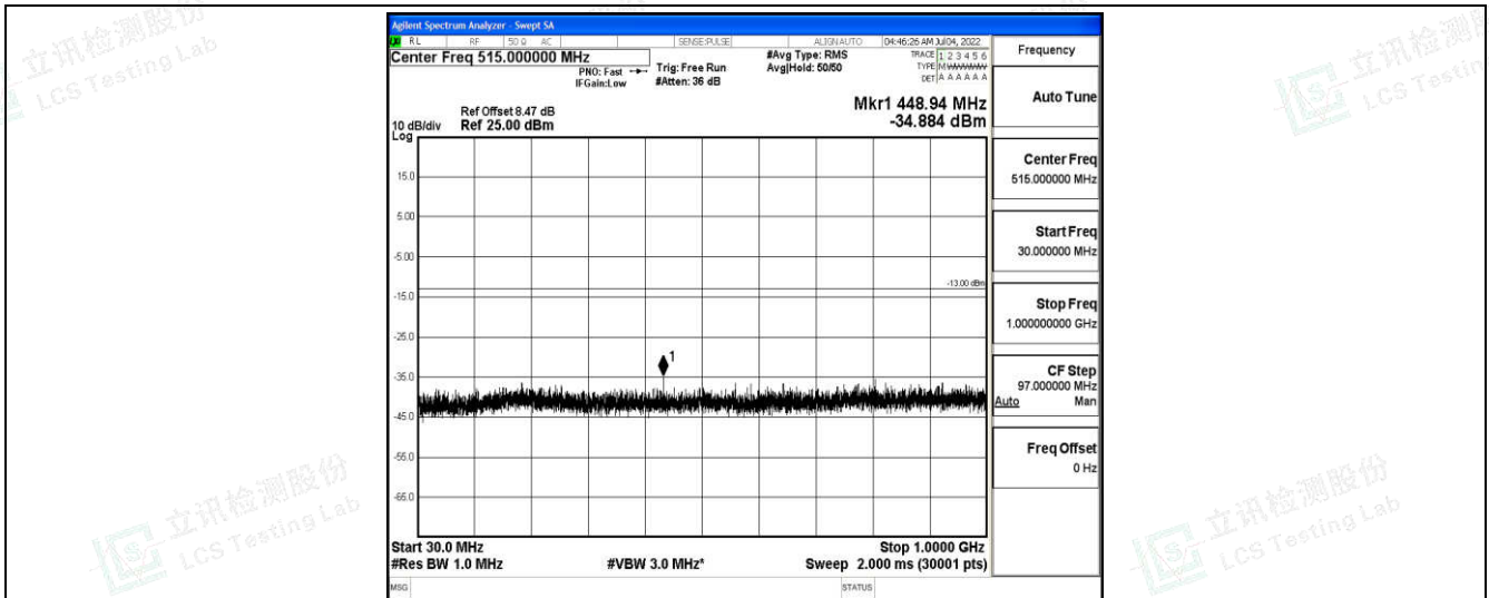
Band4-5MHz-16QAM-20375-1-0-High-30-1000--34.88-PASS
