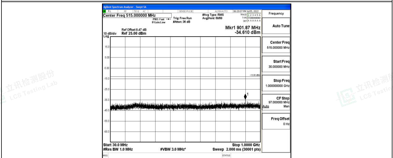
Band4-10MHz-16QAM-20000-1-0-Low-30-1000--34.61-PASS
