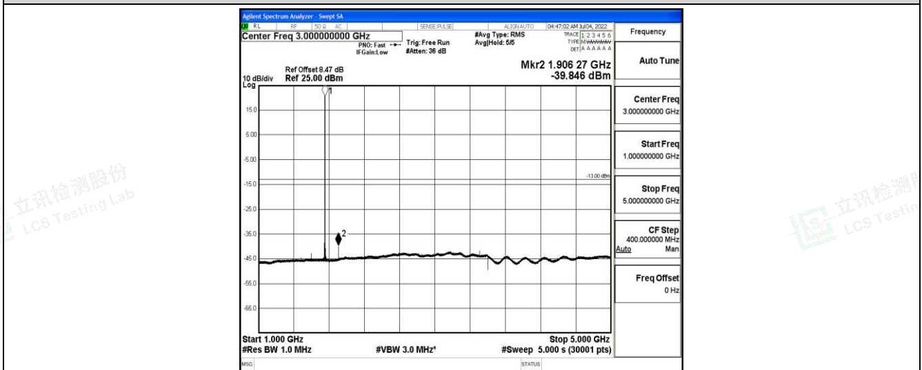
Band4-5MHz-16QAM-20375-1-0-High-1000-5000--39.85-PASS
