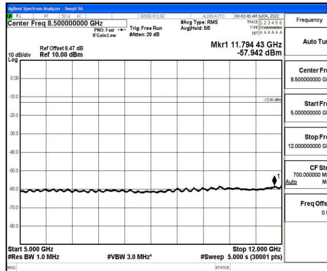
Band4-5MHz-16QAM-20175-1-0-Low-5000-12000--57.94-PASS
