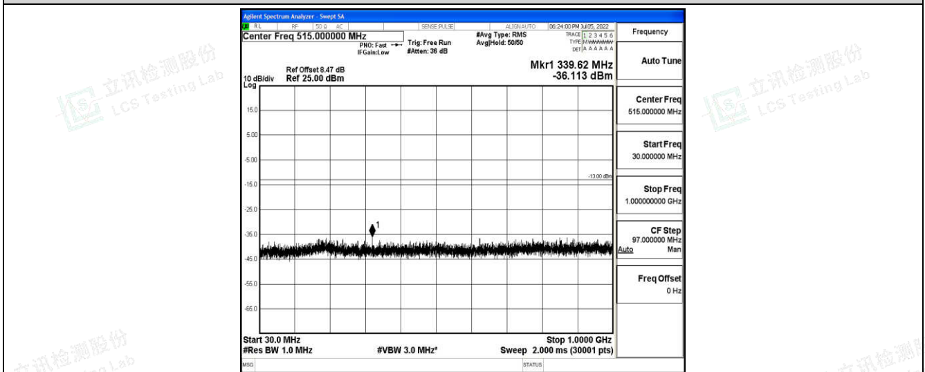
Band4-10MHz-16QAM-20175-1-0-Low-30-1000--36.11-PASS
