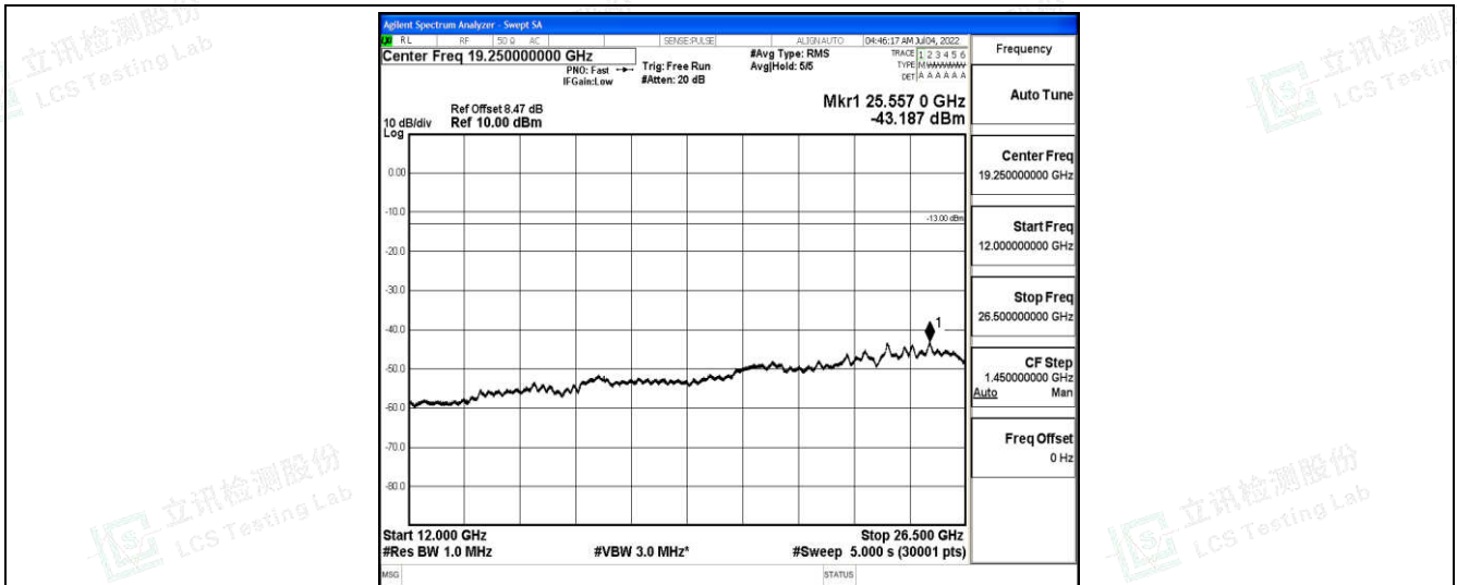
Band4-5MHz-QPSK-20375-1-0-High-12000-26500--43.19-PASS
