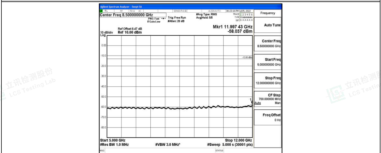
Band4-10MHz-QPSK-20175-1-0-Low-5000-12000--58.04-PASS
