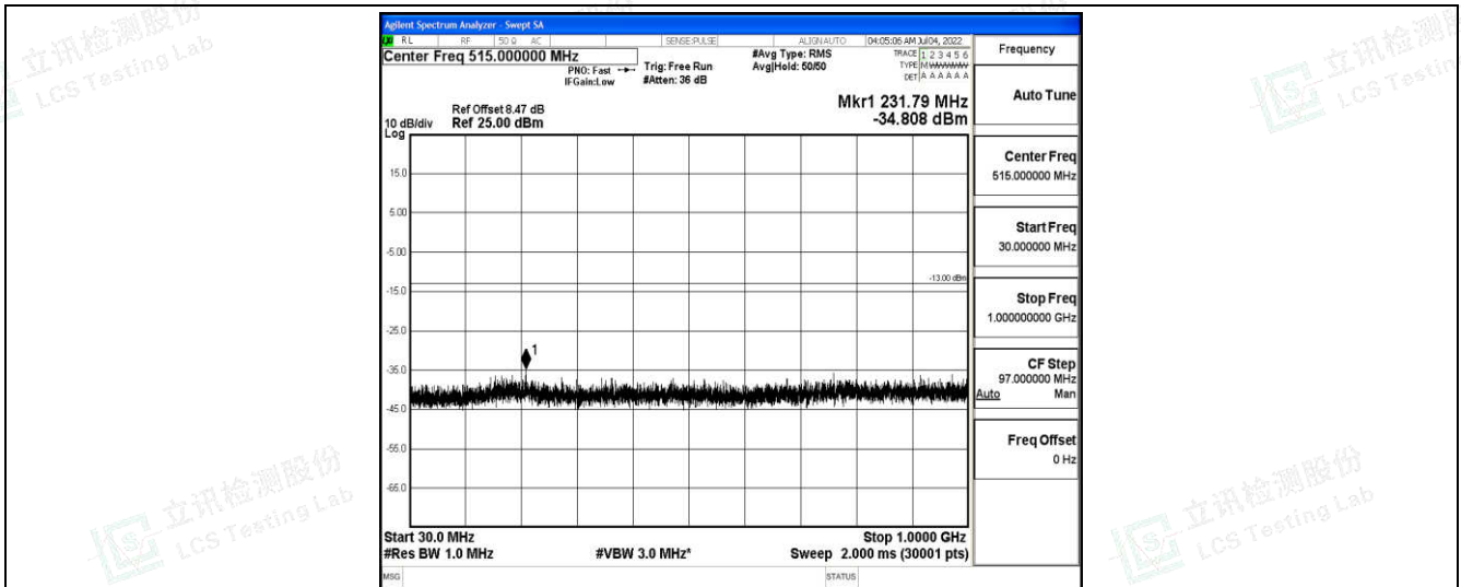
Band4-1.4MHz-16QAM-20393-1-0-High-30-1000--34.81-PASS
