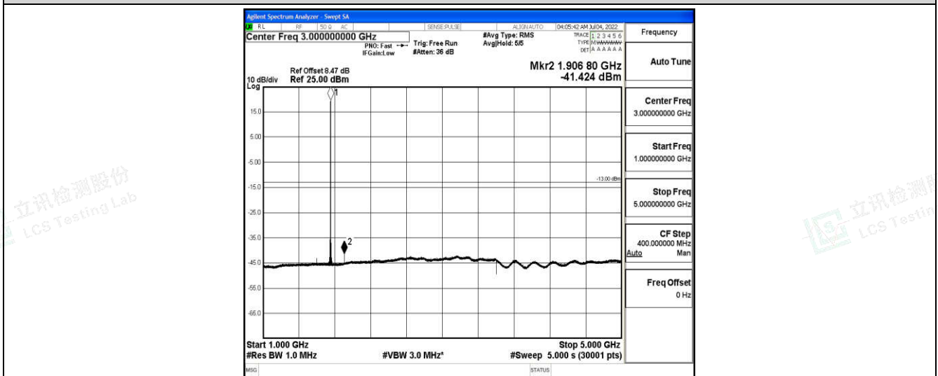
Band4-1.4MHz-16QAM-20393-1-0-High-1000-5000--41.42-PASS
