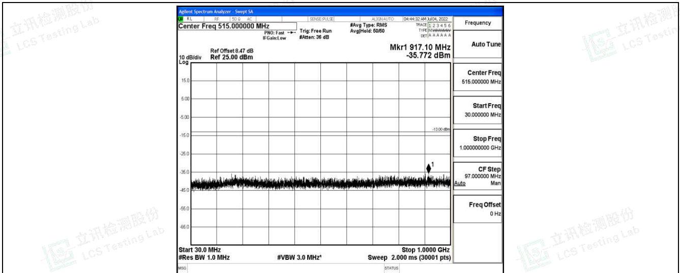
Band4-5MHz-QPSK-20375-1-0-High-30-1000--35.77-PASS
