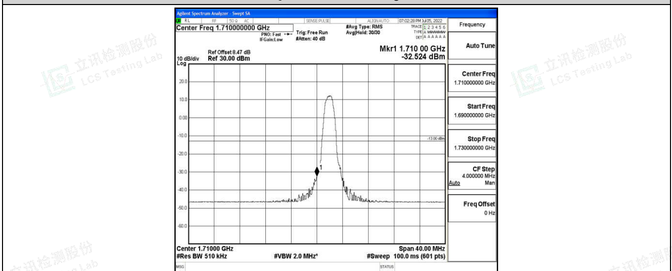
Band4-20MHz-16QAM-20050-6-0-Low--32.52-PASS
