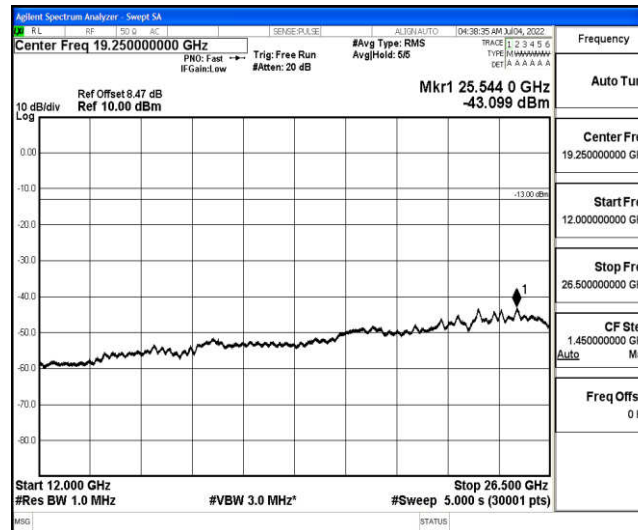
Band4-5MHz-QPSK-19975-1-0-Low-12000-26500--43.1-PASS
