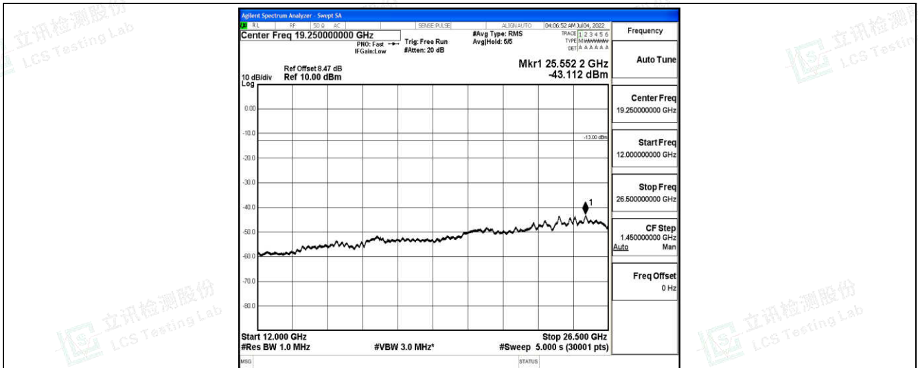
Band4-1.4MHz-16QAM-20393-1-0-High-12000-26500--43.11-PASS
