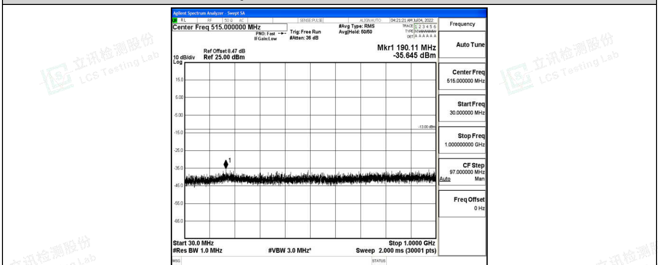
Band4-3MHz-16QAM-20175-1-0-Low-30-1000--35.65-PASS
