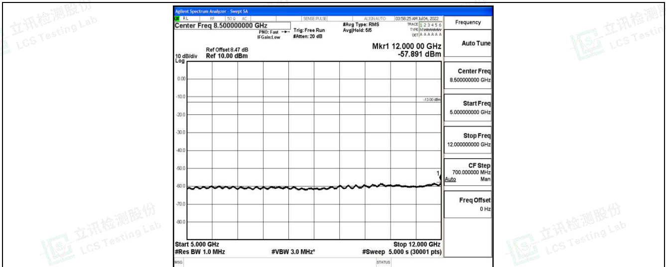
Band4-1.4MHz-16QAM-19957-1-0-Low-5000-12000--57.89-PASS
