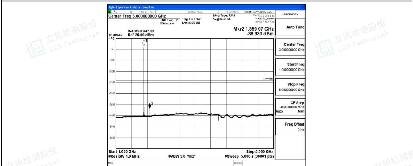
Band4-3MHz-QPSK-19965-1-0-Low-1000-5000--38.93-PASS
