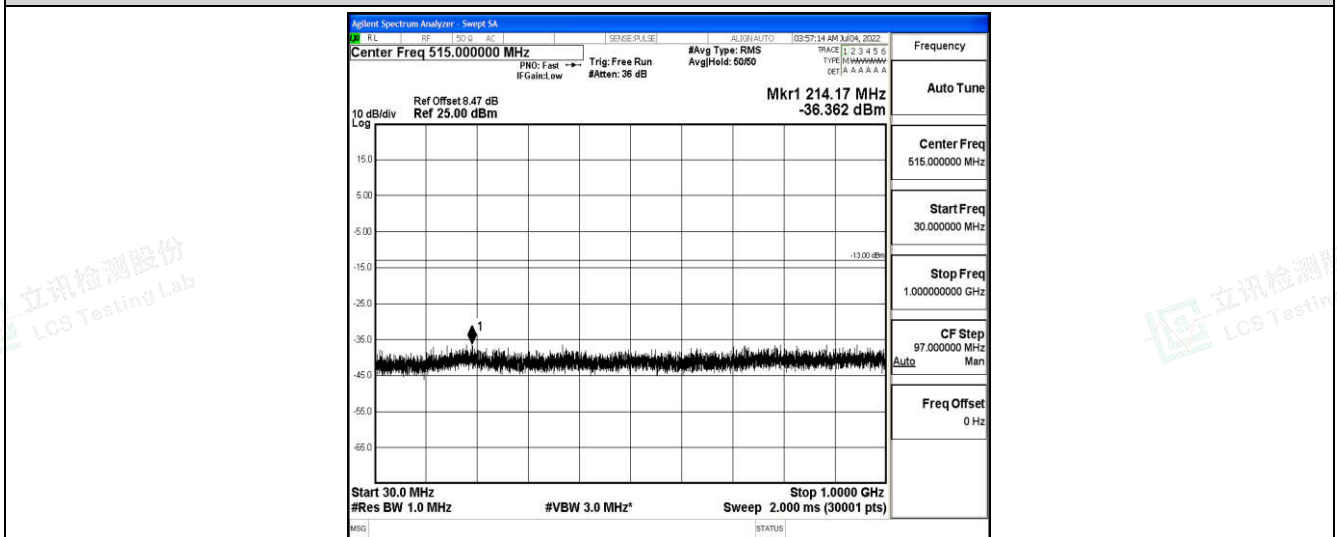
Band4-1.4MHz-16QAM-19957-1-0-Low-30-1000--36.36-PASS
