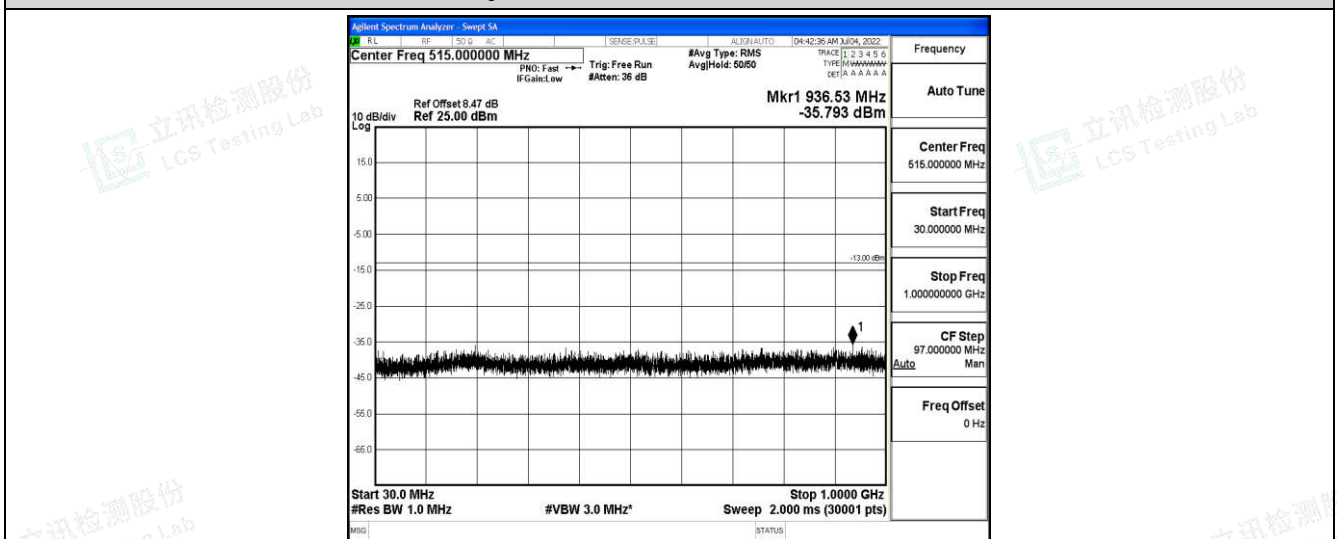
Band4-5MHz-16QAM-20175-1-0-Low-30-1000--35.79-PASS
