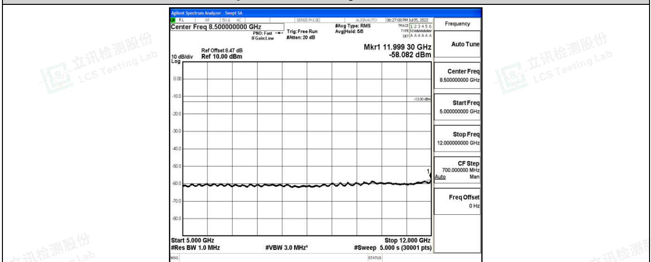
Band4-10MHz-QPSK-20350-1-0-High-5000-12000--58.08-PASS
