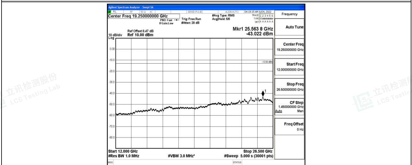
Band4-3MHz-16QAM-19965-1-0-Low-12000-26500--43.02-PASS
