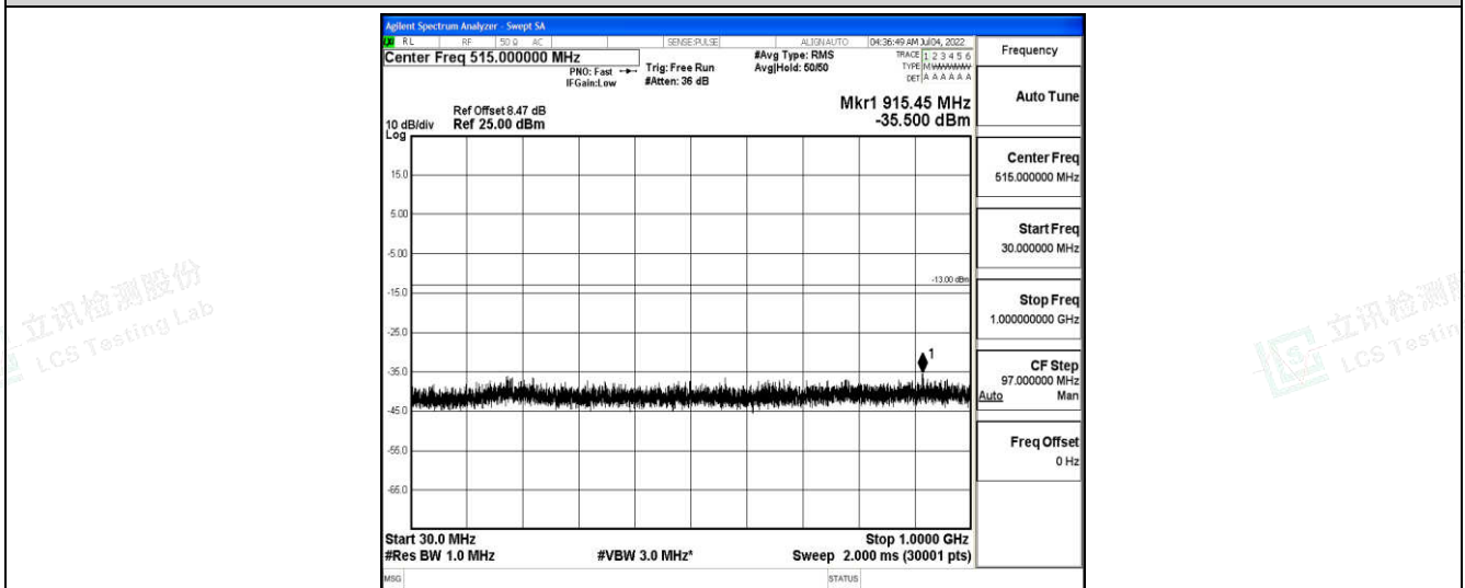
Band4-5MHz-QPSK-19975-1-0-Low-30-1000--35.5-PASS
