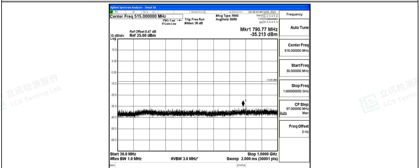
Band4-5MHz-16QAM-19975-1-0-Low-30-1000--35.21-PASS
