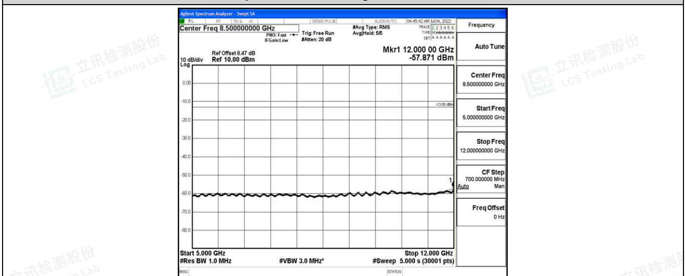
Band4-5MHz-QPSK-20375-1-0-High-5000-12000--57.87-PASS
