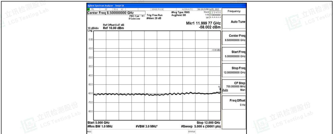
Band4-10MHz-QPSK-20000-1-0-Low-5000-12000--58-PASS
