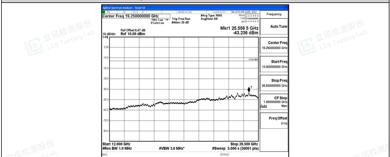
Band4-10MHz-QPSK-20175-1-0-Low-12000-26500--43.24-PASS
