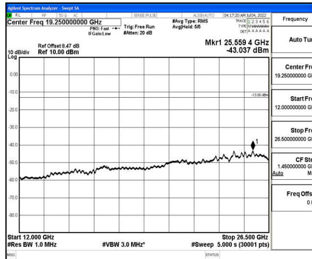
Band4-3MHz-QPSK-19965-1-0-Low-12000-26500--43.04-PASS
