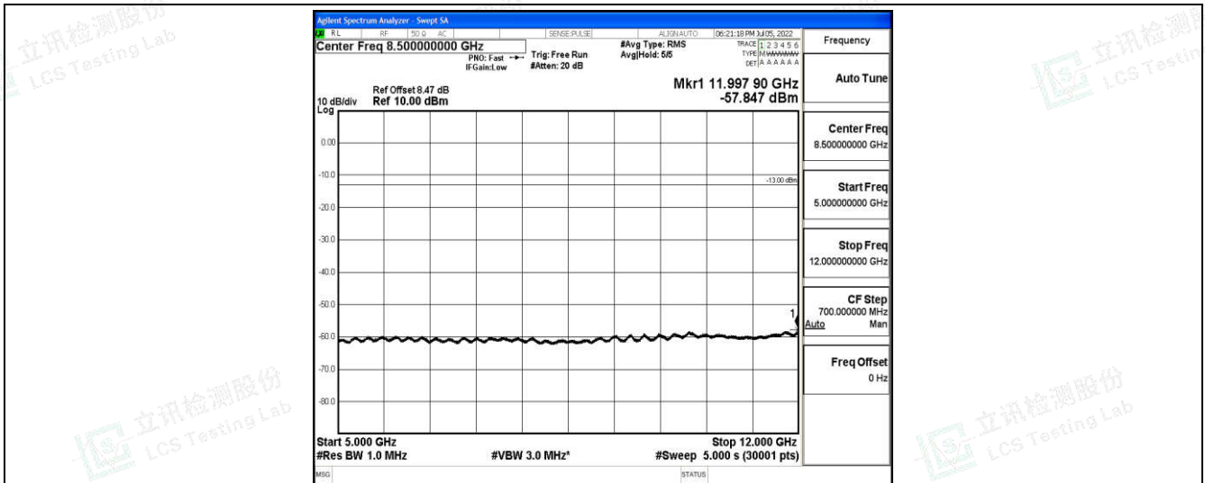
Band4-10MHz-16QAM-20000-1-0-Low-5000-12000--57.85-PASS
