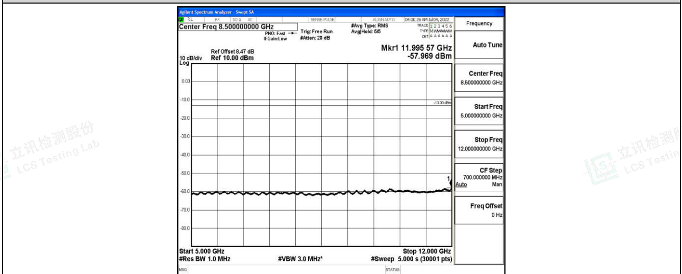
Band4-1.4MHz-QPSK-20175-1-0-Low-5000-12000--57.97-PASS
