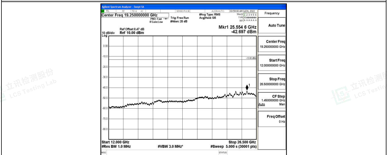
Band4-1.4MHz-16QAM-19957-1-0-Low-12000-26500--42.7-PASS
