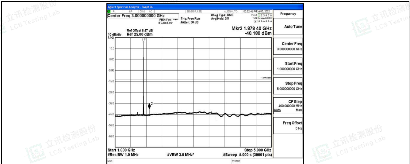
Band4-10MHz-QPSK-20175-1-0-Low-1000-5000--40.18-PASS
