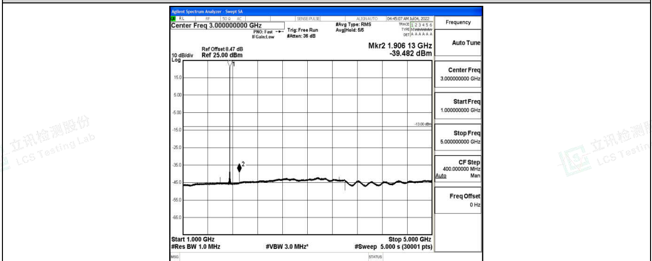
Band4-5MHz-QPSK-20375-1-0-High-1000-5000--39.48-PASS
