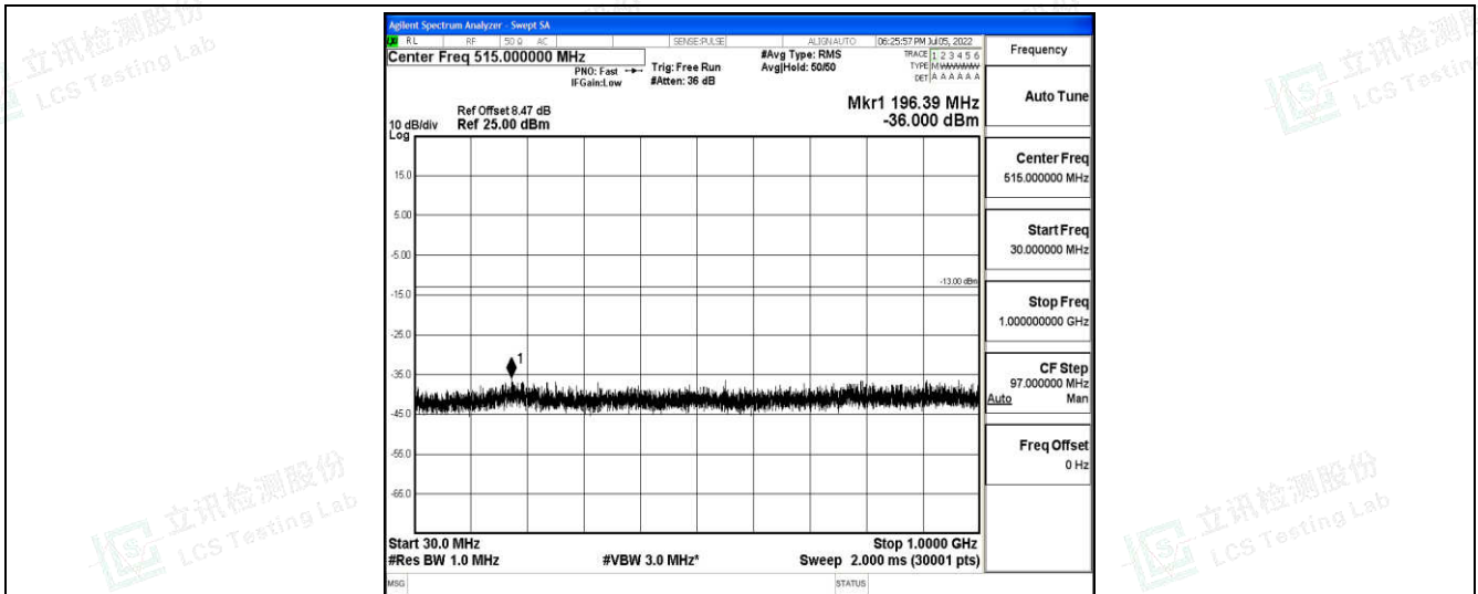
Band4-10MHz-QPSK-20350-1-0-High-30-1000--36-PASS
