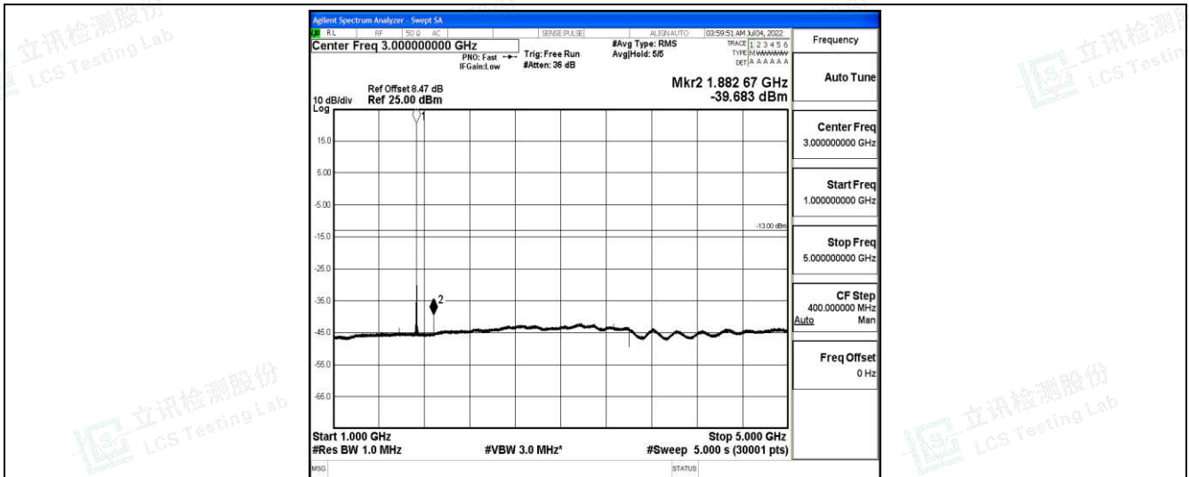
Band4-1.4MHz-QPSK-20175-1-0-Low-1000-5000--39.68-PASS
