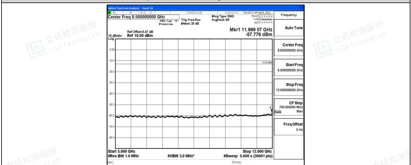
Band4-3MHz-QPSK-20385-1-0-High-5000-12000--57.78-PASS
