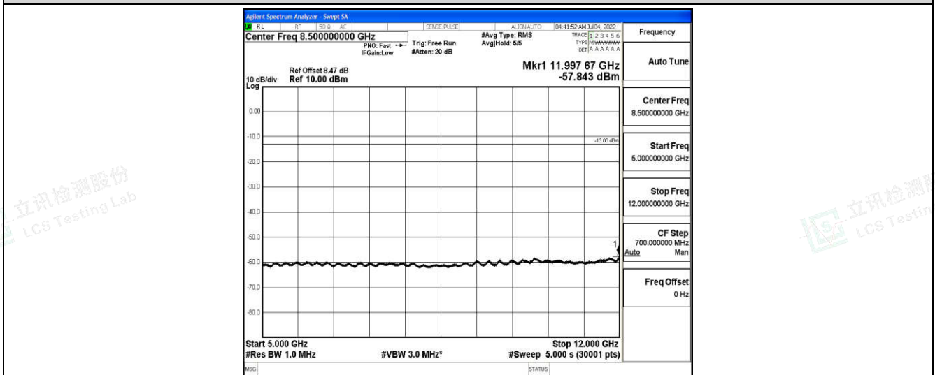
Band4-5MHz-QPSK-20175-1-0-Low-5000-12000--57.84-PASS
