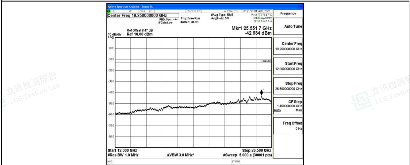
Band4-10MHz-16QAM-20000-1-0-Low-12000-26500--42.93-PASS
