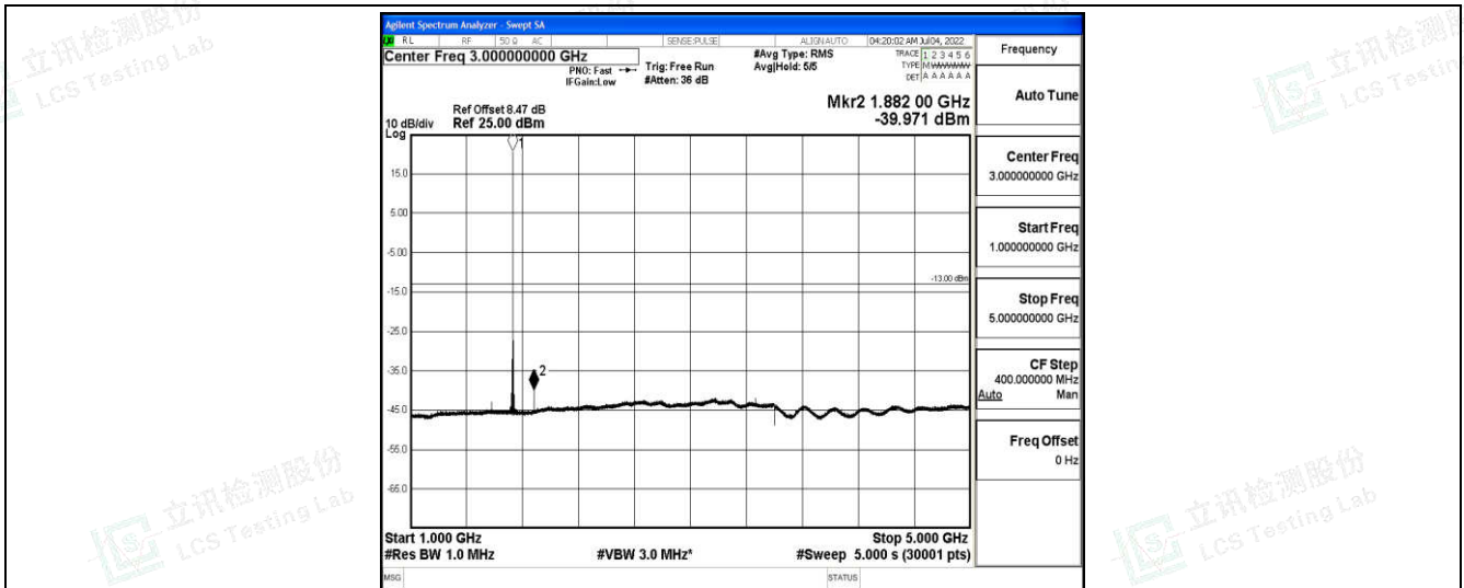
Band4-3MHz-QPSK-20175-1-0-Low-1000-5000--39.97-PASS
