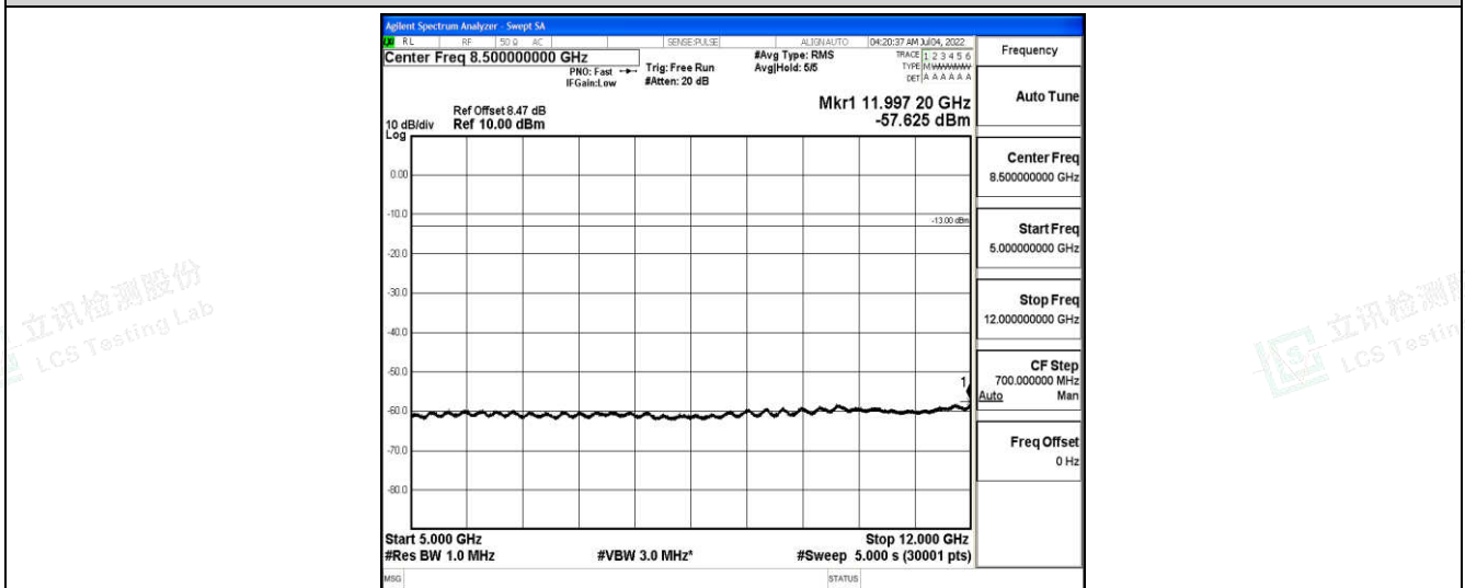
Band4-3MHz-QPSK-20175-1-0-Low-5000-12000--57.63-PASS
