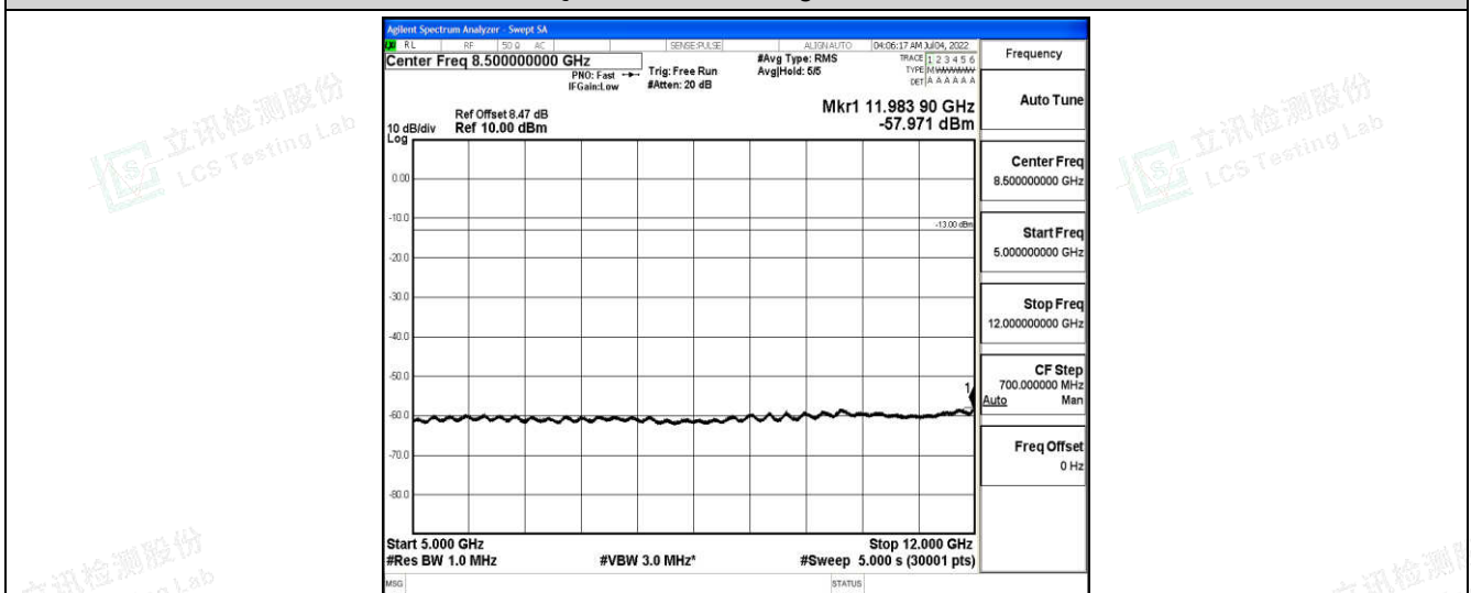
Band4-1.4MHz-16QAM-20393-1-0-High-5000-12000--57.97-PASS
