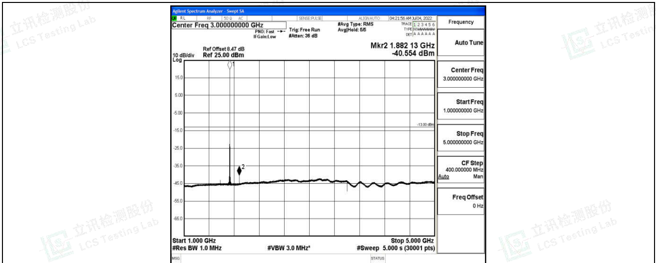
Band4-3MHz-16QAM-20175-1-0-Low-1000-5000--40.55-PASS
