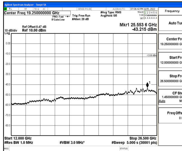
Band4-20MHz-16QAM-20050-1-0-Low-12000-26500--43.22-PASS
