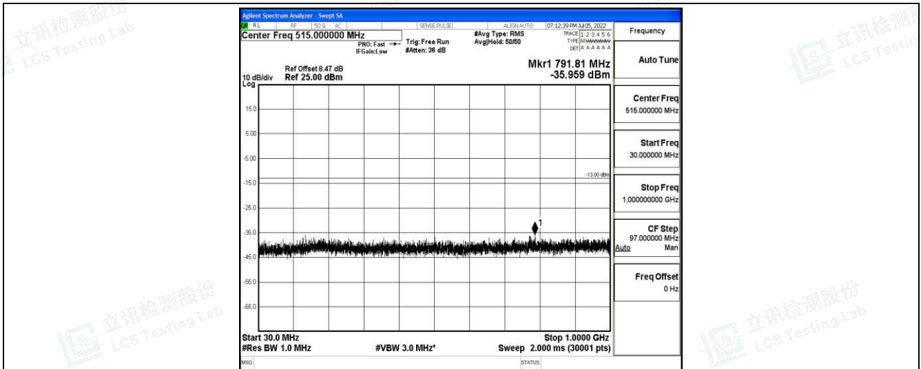
Band4-20MHz-16QAM-20300-1-0-High-30-1000--35.96-PASS
