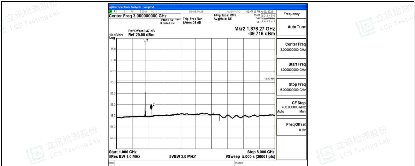
Band4-15MHz-QPSK-20175-1-0-Low-1000-5000--39.72-PASS
