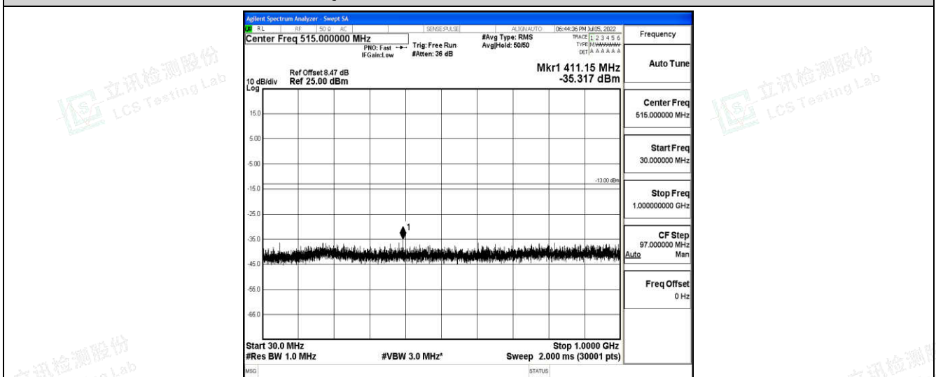
Band4-15MHz-QPSK-20175-1-0-Low-30-1000--35.32-PASS
