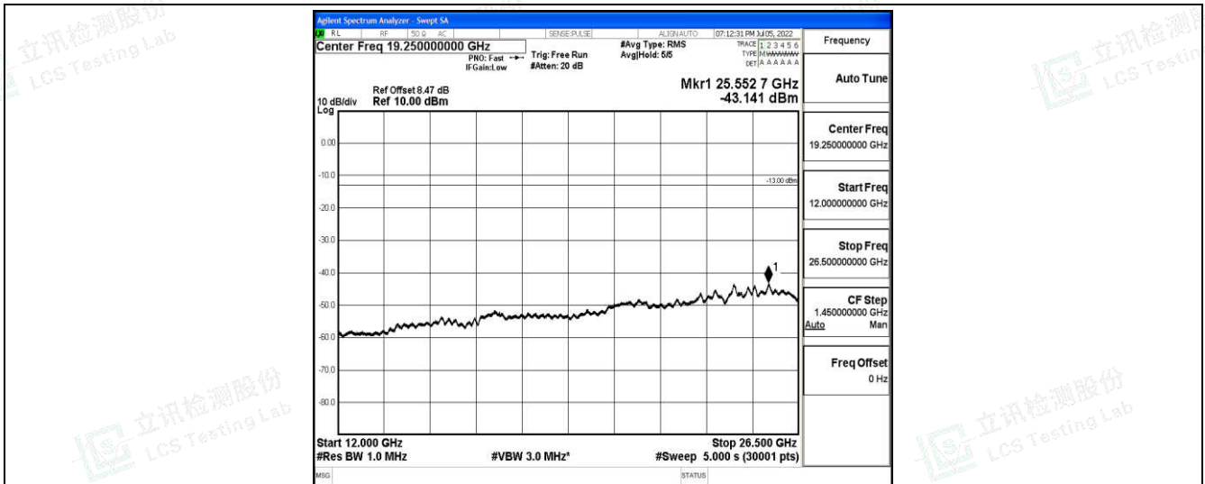
Band4-20MHz-QPSK-20300-1-0-High-12000-26500--43.14-PASS
