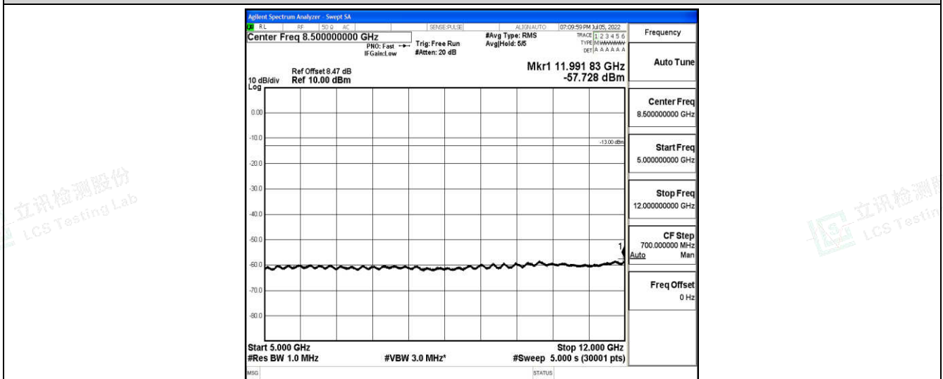
Band4-20MHz-16QAM-20175-1-0-Low-5000-12000--57.73-PASS
