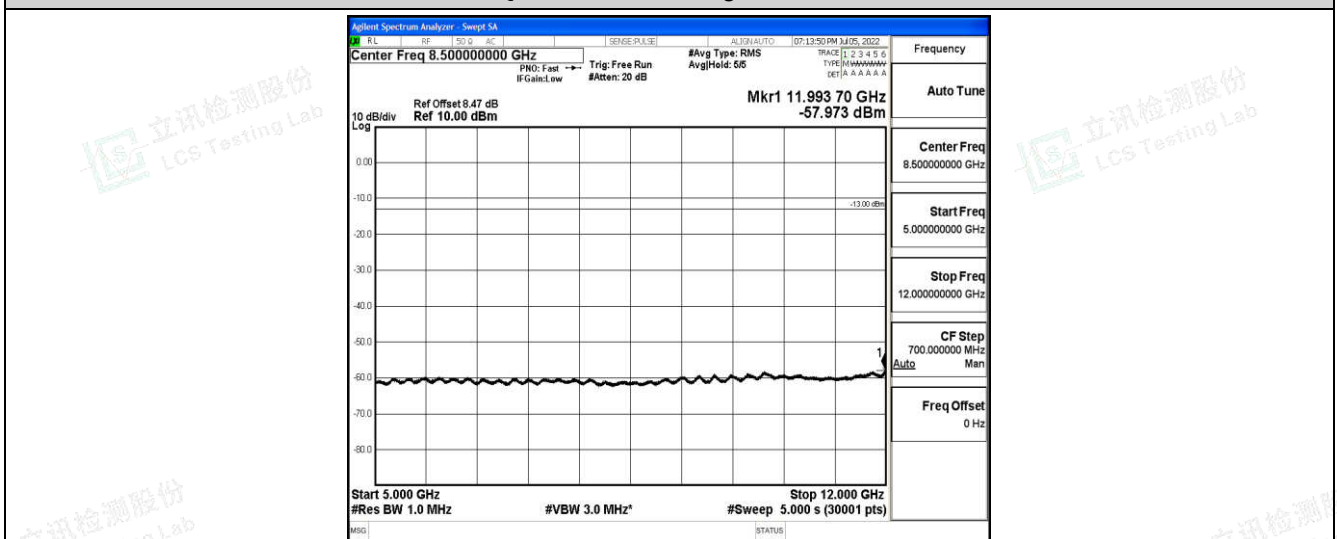
Band4-20MHz-16QAM-20300-1-0-High-5000-12000--57.97-PASS
