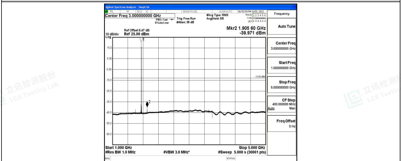
Band4-15MHz-16QAM-20325-1-0-High-1000-5000--39.97-PASS
