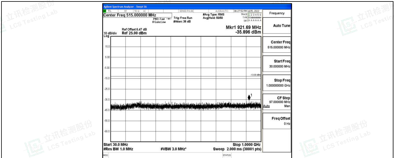
Band4-10MHz-16QAM-20350-1-0-High-30-1000--35.9-PASS
