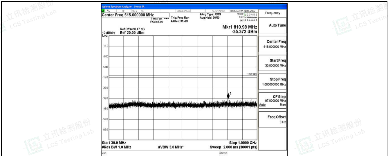
Band4-15MHz-16QAM-20325-1-0-High-30-1000--35.37-PASS
