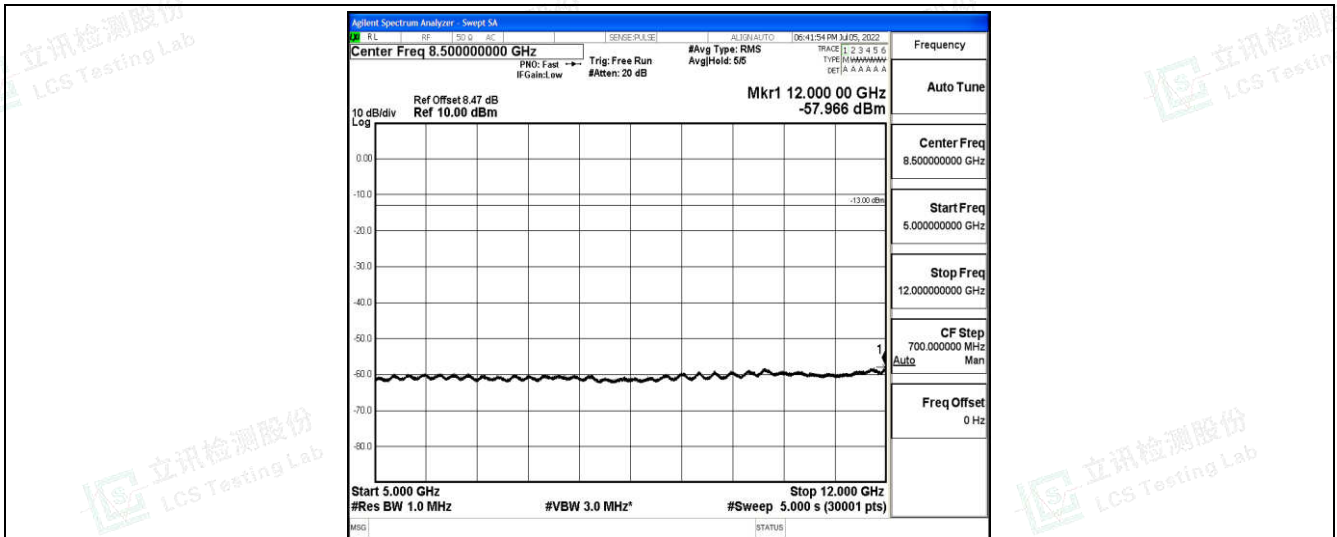
Band4-15MHz-QPSK-20025-1-0-Low-5000-12000--57.97-PASS
