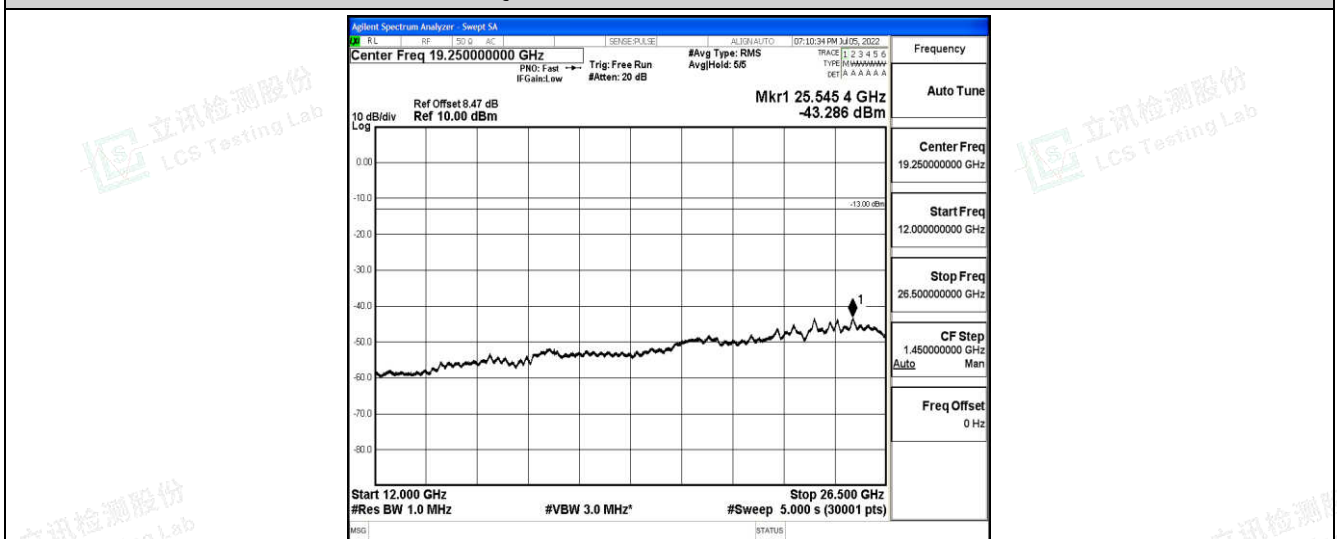
Band4-20MHz-16QAM-20175-1-0-Low-12000-26500--43.29-PASS
