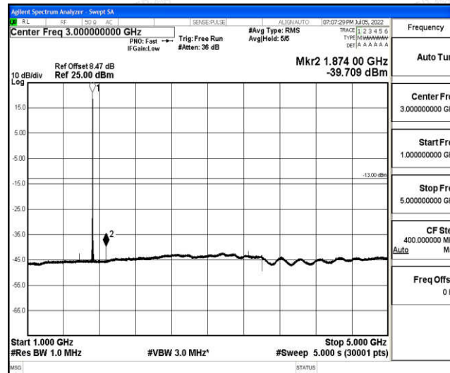
Band4-20MHz-QPSK-20175-1-0-Low-1000-5000--39.71-PASS
