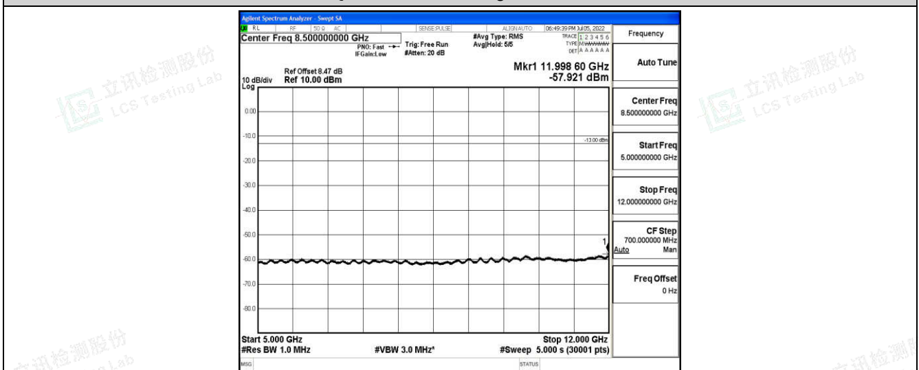
Band4-15MHz-QPSK-20325-1-0-High-5000-12000--57.92-PASS
