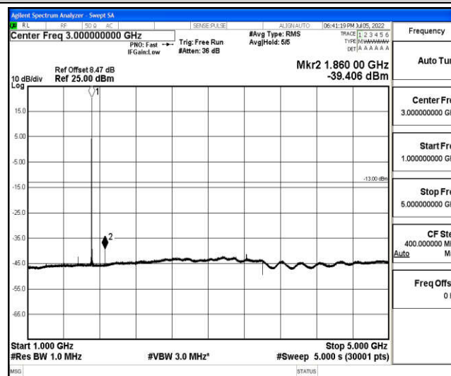
Band4-15MHz-QPSK-20025-1-0-Low-1000-5000--39.41-PASS
