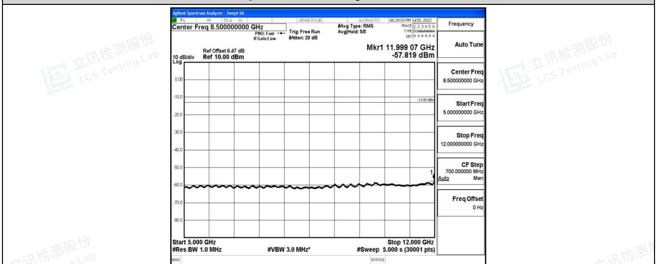
Band4-10MHz-16QAM-20350-1-0-High-5000-12000--57.82-PASS
