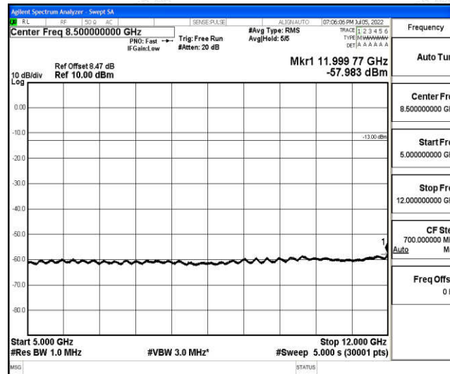
Band4-20MHz-16QAM-20050-1-0-Low-5000-12000--57.98-PASS
