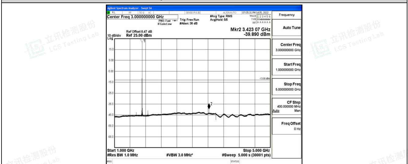
Band4-20MHz-16QAM-20050-1-0-Low-1000-5000--39.89-PASS
