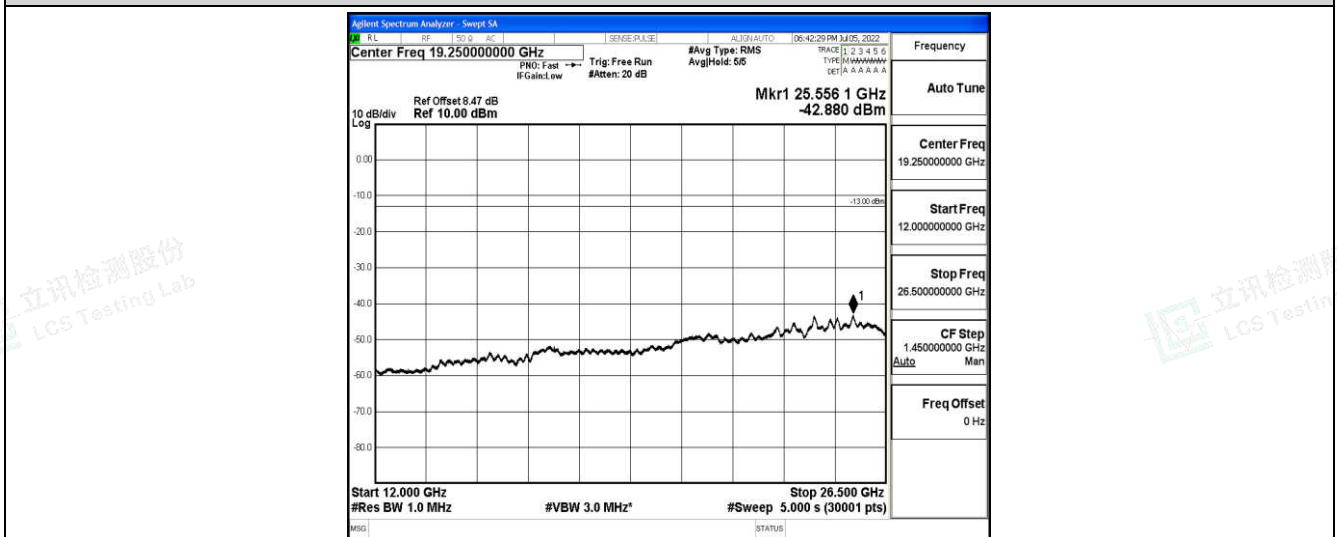
Band4-15MHz-QPSK-20025-1-0-Low-12000-26500--42.88-PASS
