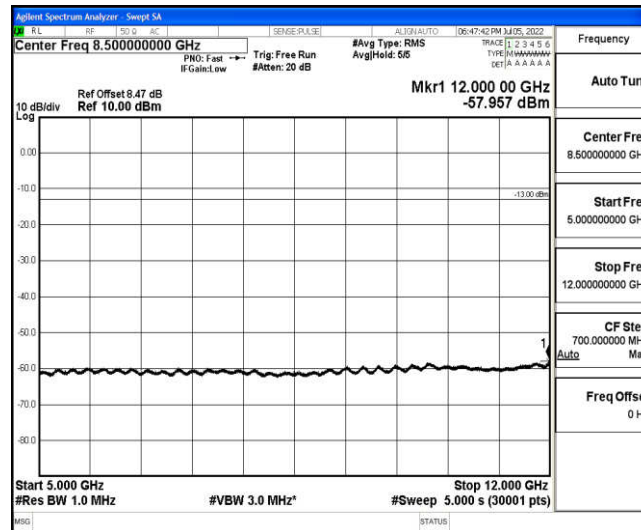
Band4-15MHz-16QAM-20175-1-0-Low-5000-12000--57.96-PASS
