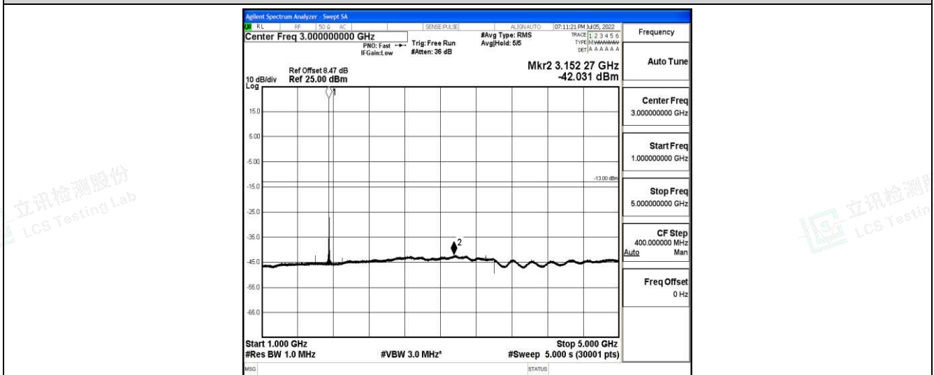
Band4-20MHz-QPSK-20300-1-0-High-1000-5000--42.03-PASS
