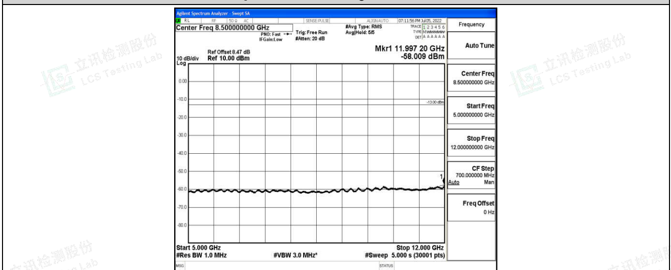
Band4-20MHz-QPSK-20300-1-0-High-5000-12000--58.01-PASS
