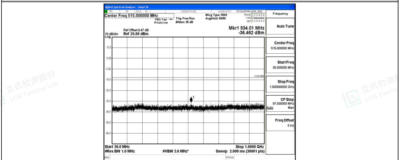
Band4-20MHz-16QAM-20050-1-0-Low-30-1000--36.46-PASS
