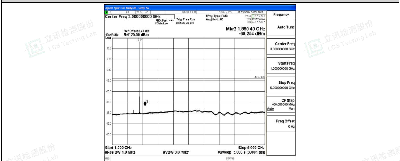
Band4-20MHz-QPSK-20050-1-0-Low-1000-5000--39.25-PASS
