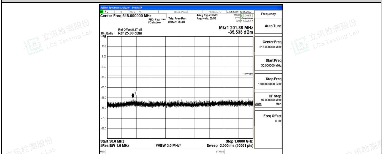
Band4-20MHz-QPSK-20175-1-0-Low-30-1000--35.53-PASS
