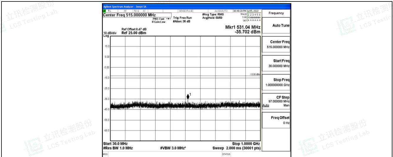
Band4-15MHz-QPSK-20325-1-0-High-30-1000--35.7-PASS
