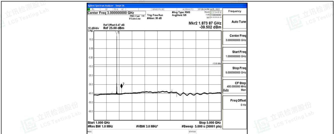
Band4-20MHz-16QAM-20175-1-0-Low-1000-5000--39.5-PASS
