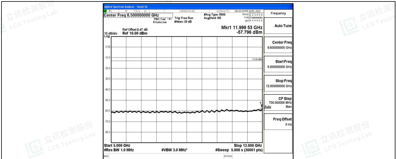
Band4-15MHz-16QAM-20025-1-0-Low-5000-12000--57.8-PASS
