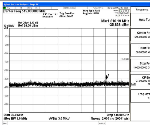
Band4-15MHz-16QAM-20025-1-0-Low-30-1000--35.84-PASS
