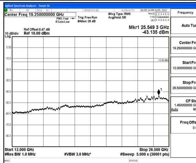
Band4-15MHz-QPSK-20325-1-0-High-12000-26500--43.14-PASS
