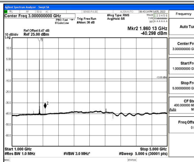
Band4-15MHz-16QAM-20025-1-0-Low-1000-5000--40.3-PASS
