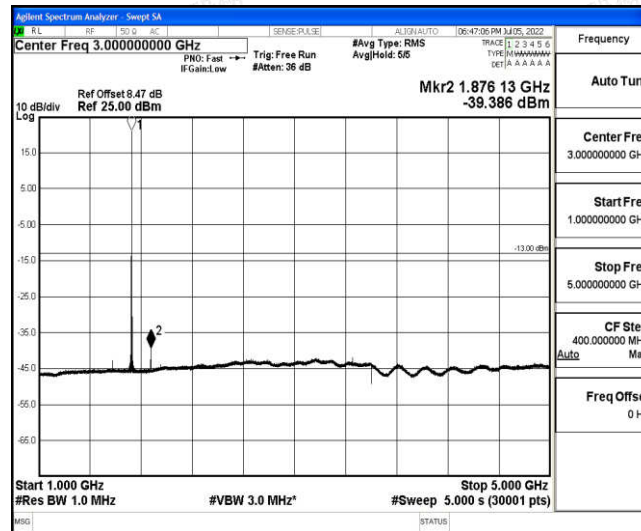
Band4-15MHz-16QAM-20175-1-0-Low-1000-5000--39.39-PASS
