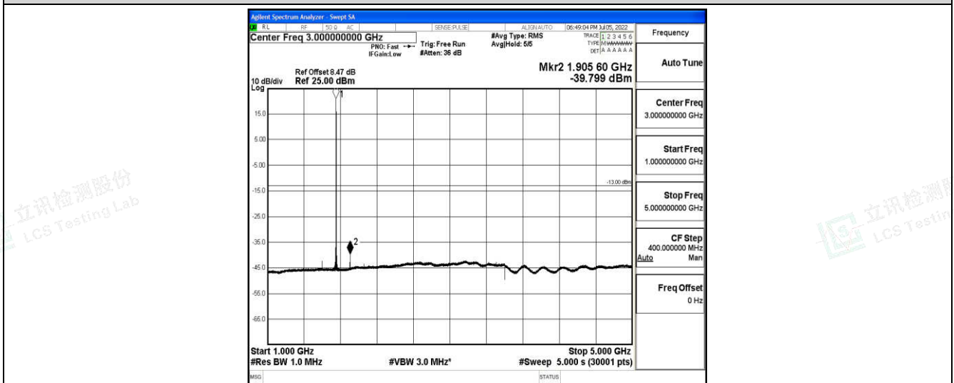
Band4-15MHz-QPSK-20325-1-0-High-1000-5000--39.8-PASS
