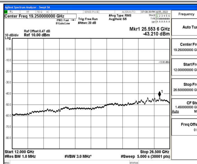
Band4-20MHz-QPSK-20175-1-0-Low-12000-26500--43.21-PASS
