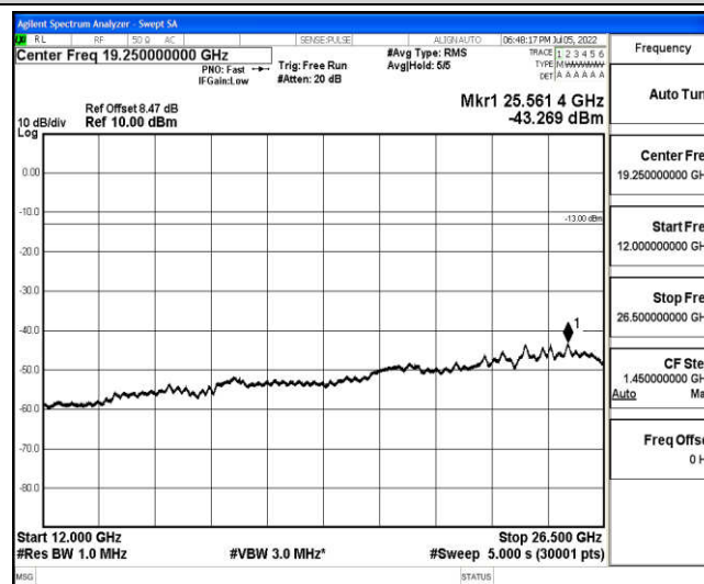
Band4-15MHz-16QAM-20175-1-0-Low-12000-26500--43.27-PASS
