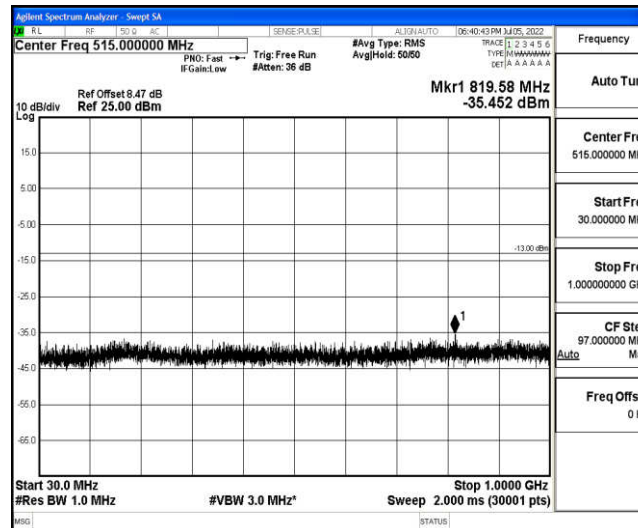
Band4-15MHz-QPSK-20025-1-0-Low-30-1000--35.45-PASS
