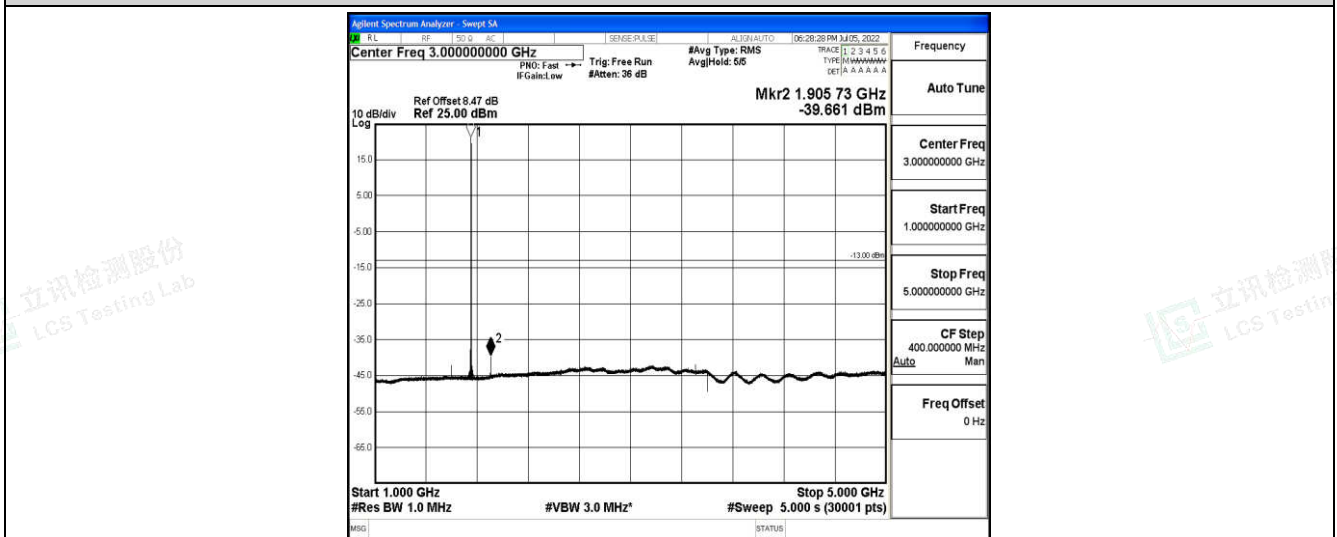
Band4-10MHz-16QAM-20350-1-0-High-1000-5000--39.66-PASS
