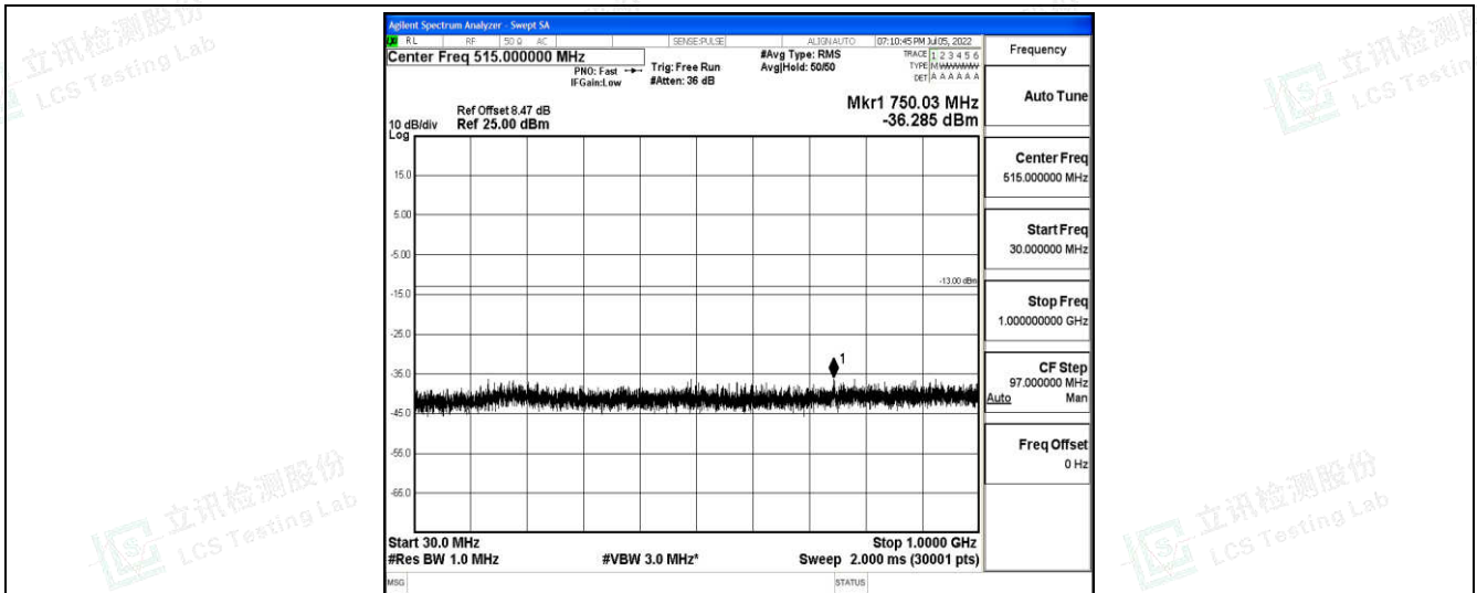
Band4-20MHz-QPSK-20300-1-0-High-30-1000--36.29-PASS
