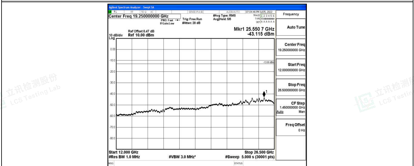
Band4-20MHz-QPSK-20050-1-0-Low-12000-26500--43.12-PASS
