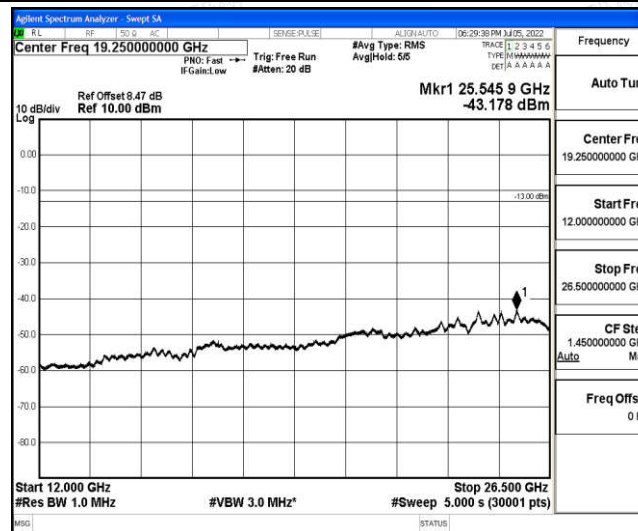
Band4-10MHz-16QAM-20350-1-0-High-12000-26500--43.18-PASS
