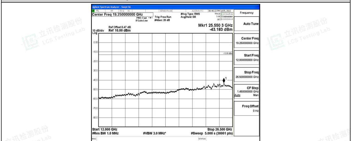
Band4-15MHz-QPSK-20175-1-0-Low-12000-26500--43.18-PASS
