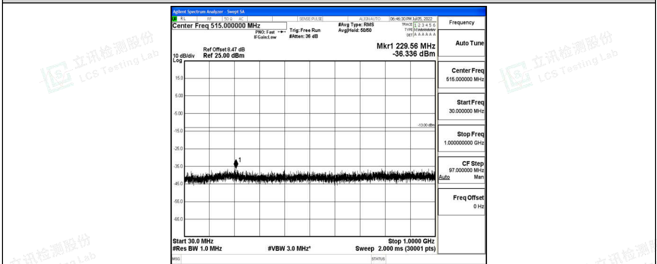
Band4-15MHz-16QAM-20175-1-0-Low-30-1000--36.34-PASS
