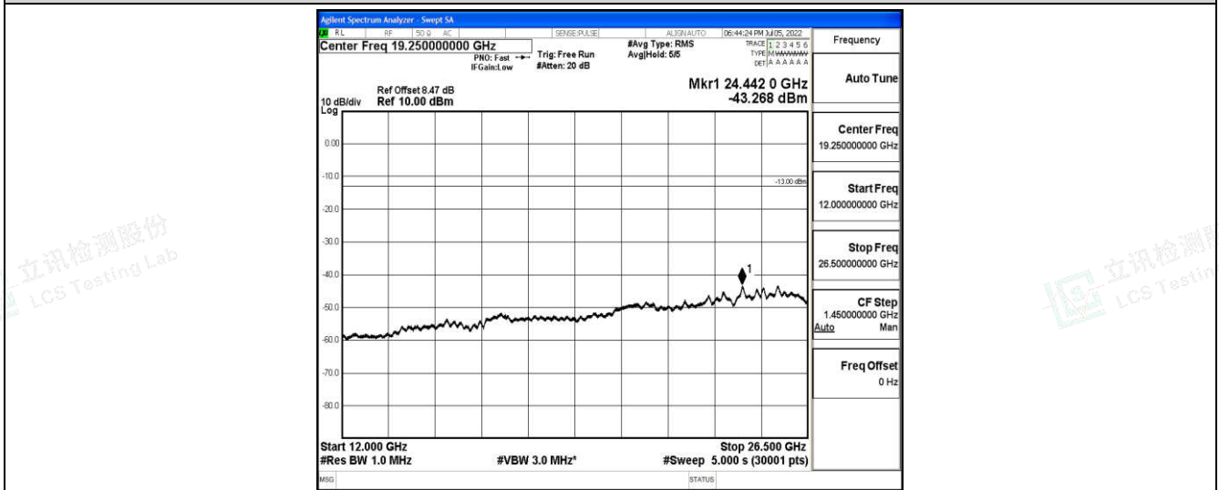
Band4-15MHz-16QAM-20025-1-0-Low-12000-26500--43.27-PASS
