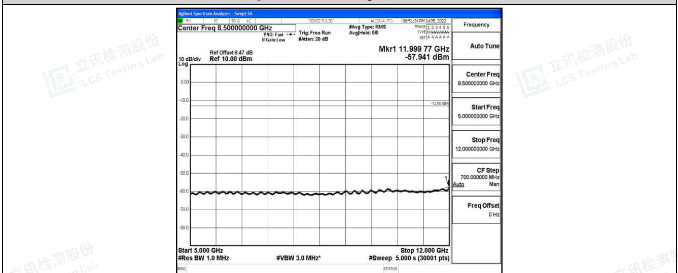
Band4-15MHz-16QAM-20325-1-0-High-5000-12000--57.94-PASS
