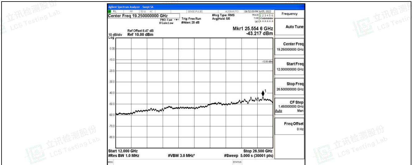
Band4-15MHz-16QAM-20325-1-0-High-12000-26500--43.22-PASS
