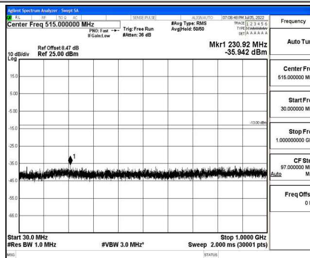
Band4-20MHz-16QAM-20175-1-0-Low-30-1000--35.94-PASS
