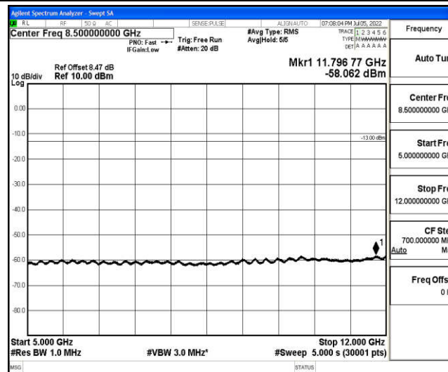
Band4-20MHz-QPSK-20175-1-0-Low-5000-12000--58.06-PASS
