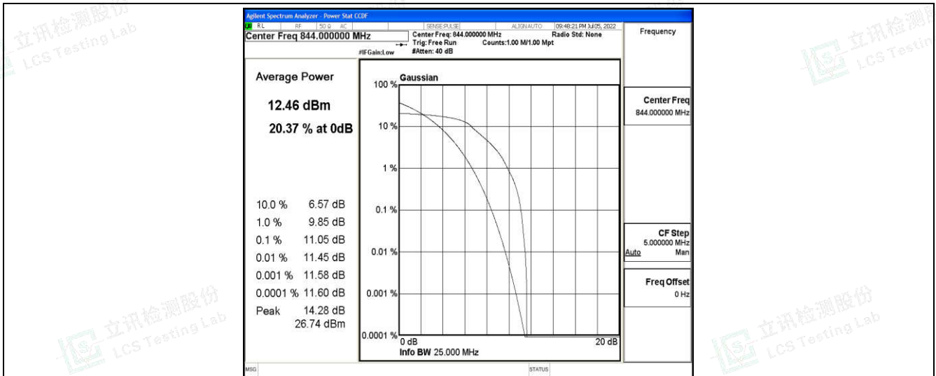
Band5-10MHz-QPSK-20600-6-0-High-11.05-&lt;=13-PASS
