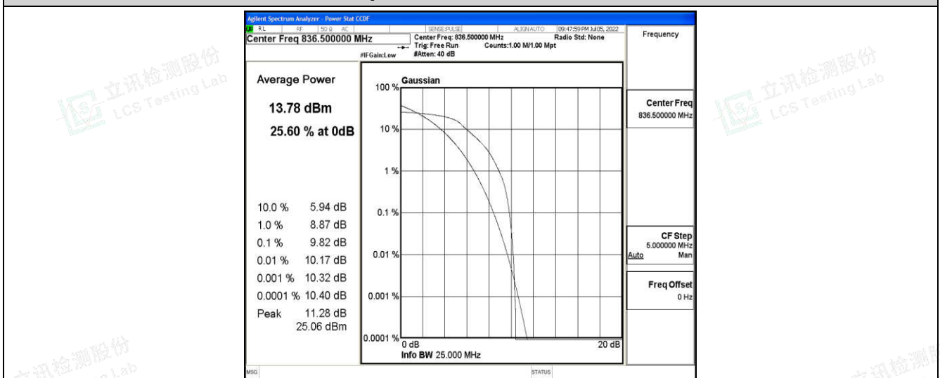
Band5-10MHz-QPSK-20525-6-0-Low-9.82-&lt;=13-PASS
