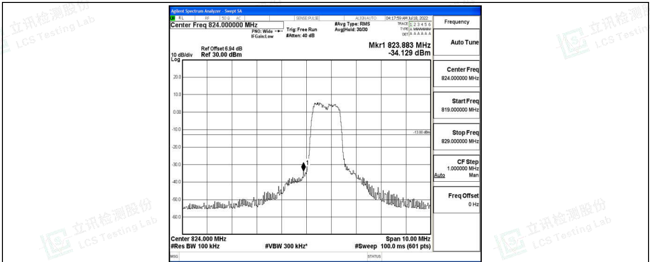
Band5-5MHz-16QAM-20425-6-0-Low--34.13-PASS
