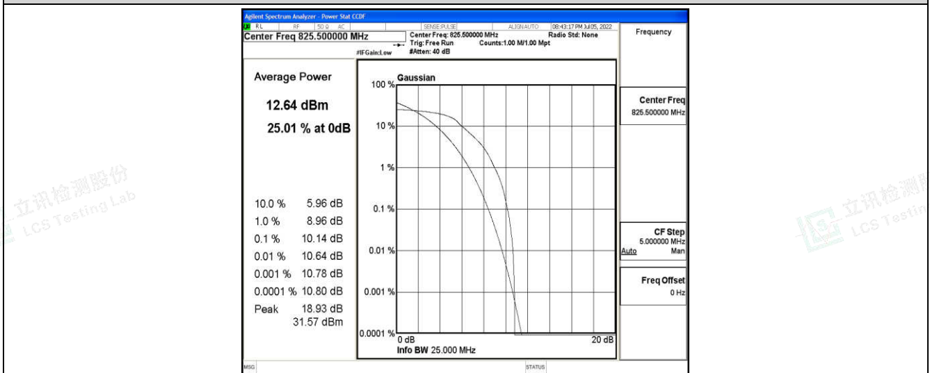
Band5-3MHz-QPSK-20415-6-0-Low-10.14-&lt;=13-PASS
