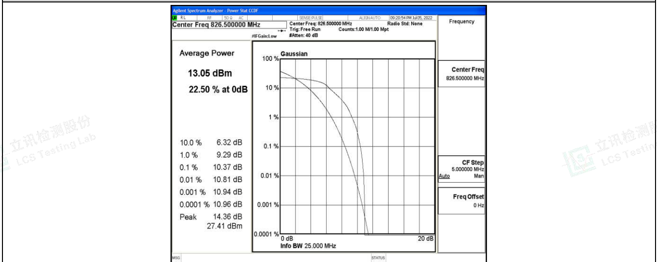
Band5-5MHz-QPSK-20425-6-0-Low-10.37-&lt;=13-PASS
