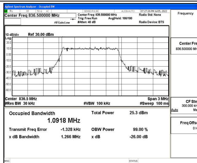
Band5-1.4MHz-16QAM-20525-6-0-Low-1.0918-1.266-PASS
