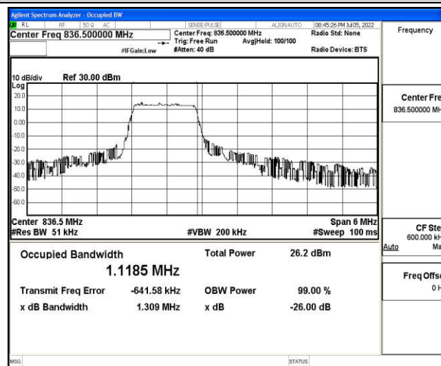
Band5-3MHz-16QAM-20525-6-0-Low-1.1185-1.309-PASS
