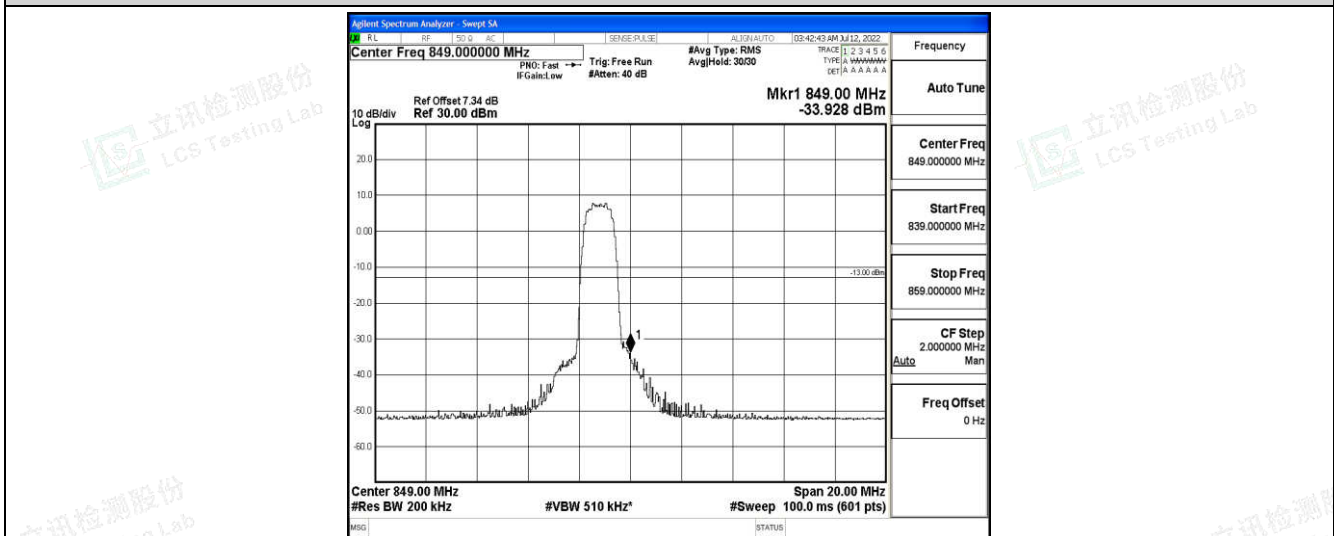
Band5-10MHz-16QAM-20600-6-0-High--33.93-PASS
