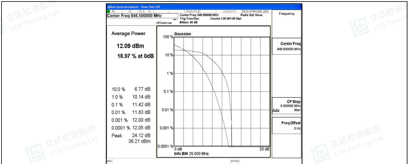
Band5-5MHz-16QAM-20625-6-0-High-11.42-&lt;=13-PASS
