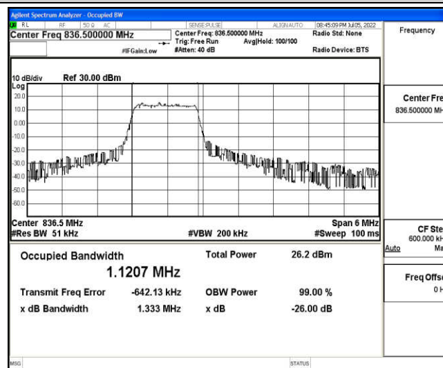
Band5-3MHz-QPSK-20525-6-0-Low-1.1207-1.333-PASS
