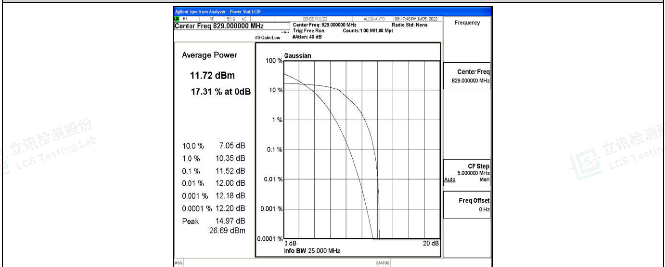
Band5-10MHz-16QAM-20450-6-0-Low-11.52-&lt;=13-PASS
