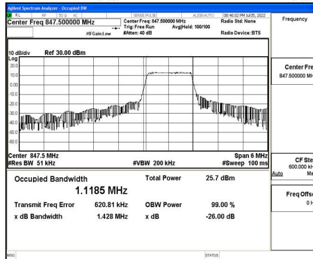
Band5-3MHz-16QAM-20635-6-0-High-1.1185-1.428-PASS
