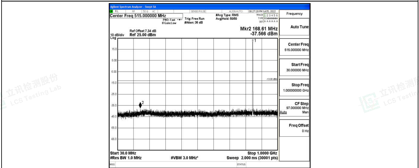
Band5-1.4MHz-16QAM-20643-1-0-High-30-1000--37.57-PASS
