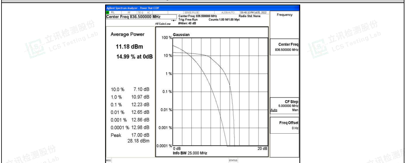
Band5-10MHz-16QAM-20525-6-0-Low-12.23-&lt;=13-PASS
