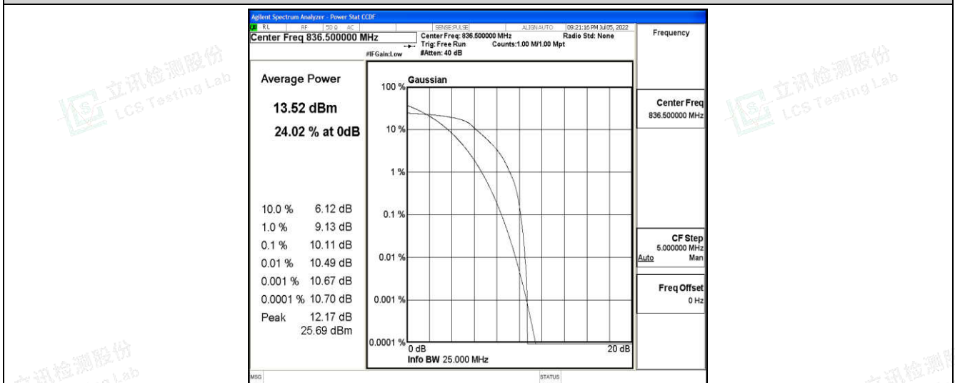
Band5-5MHz-QPSK-20525-6-0-Low-10.11-&lt;=13-PASS
