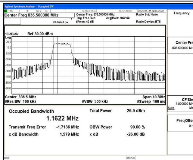
Band5-5MHz-QPSK-20525-6-0-Low-1.1622-1.579-PASS
