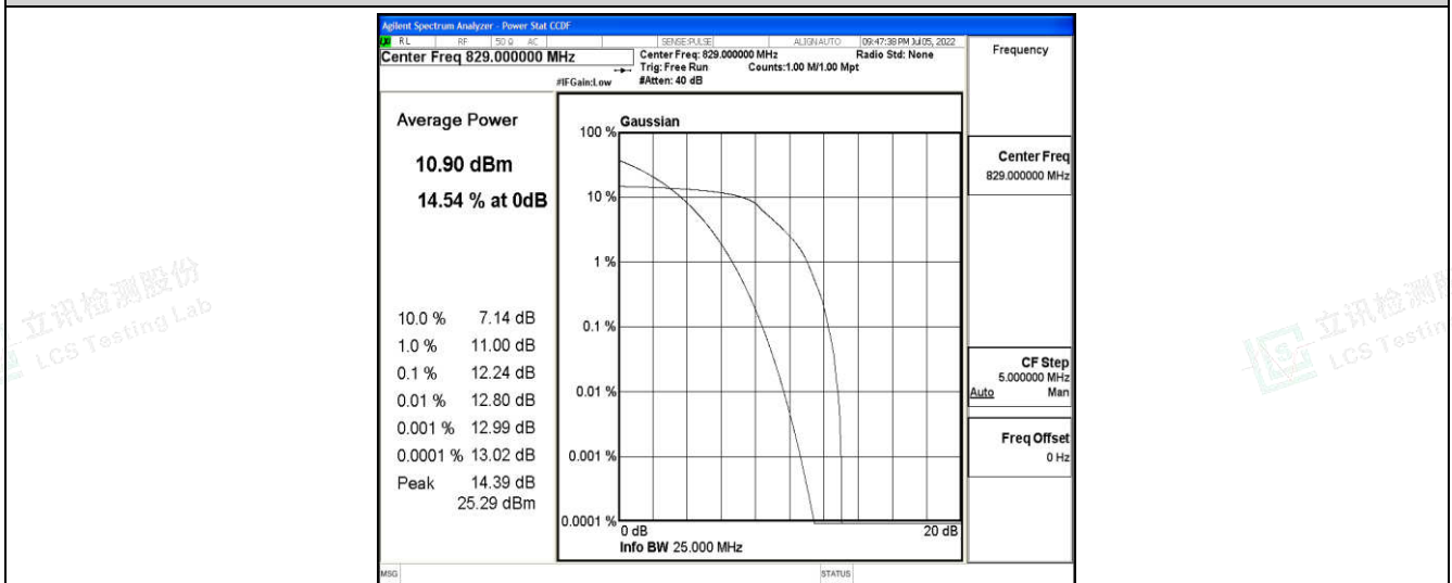
Band5-10MHz-QPSK-20450-6-0-Low-12.24-&lt;=13-PASS
