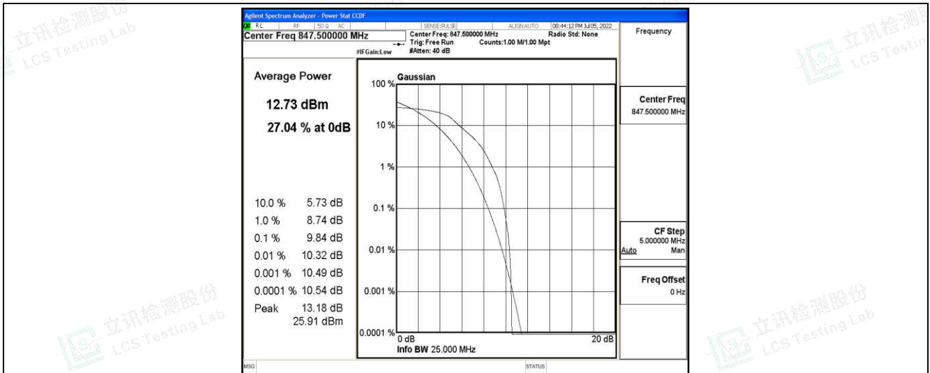
Band5-3MHz-16QAM-20635-6-0-High-9.84-&lt;=13-PASS
