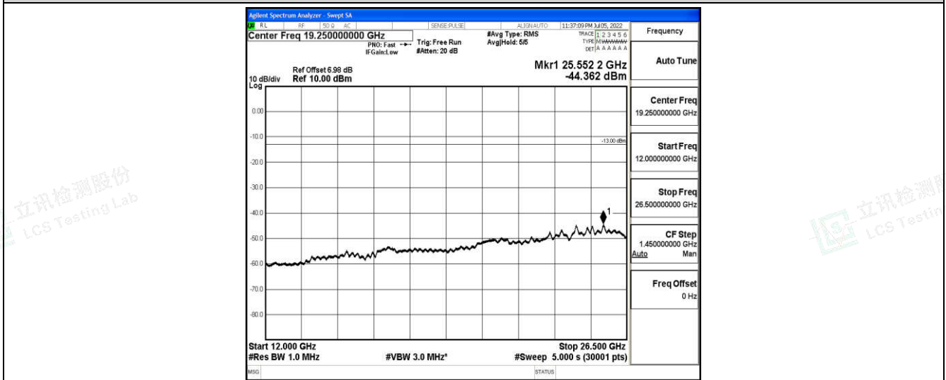
Band12-10MHz-16QAM-23060-1-0-Low-12000-26500--44.36-PASS
