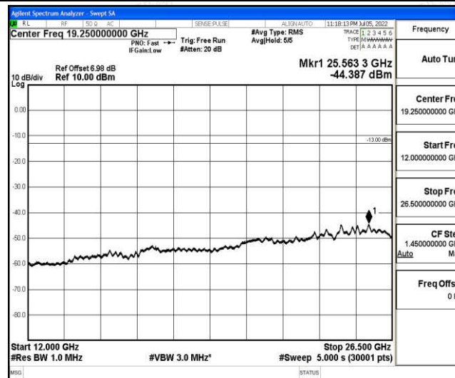
Band12-5MHz-16QAM-23155-1-0-High-12000-26500--44.39-PASS
