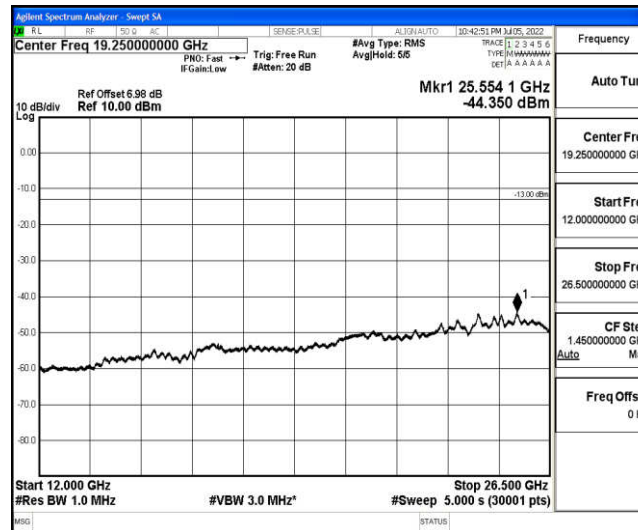
Band12-3MHz-QPSK-23025-1-0-Low-12000-26500--44.35-PASS
