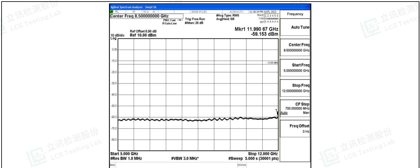
Band12-10MHz-16QAM-23060-1-0-Low-5000-12000--59.15-PASS
