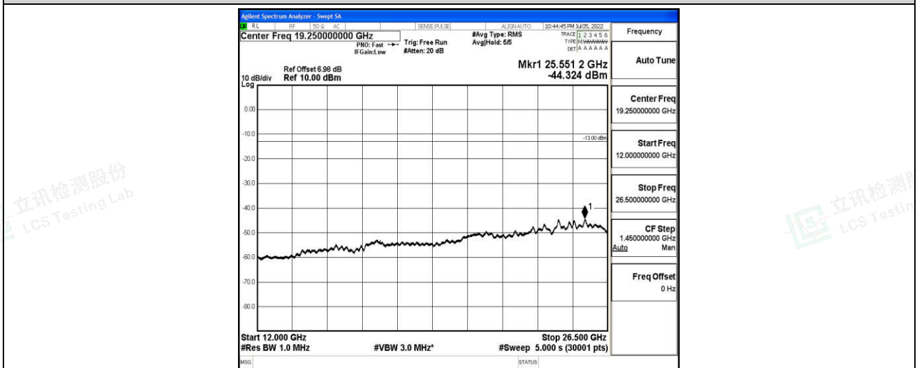
Band12-3MHz-16QAM-23025-1-0-Low-12000-26500--44.32-PASS
