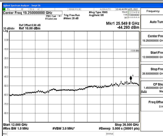
Band12-3MHz-QPSK-23095-1-0-Low-12000-26500--44.29-PASS
