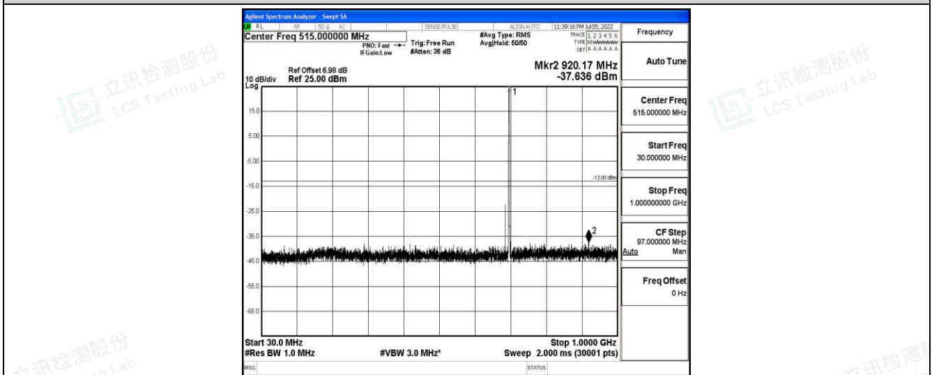
Band12-10MHz-16QAM-23095-1-0-Low-30-1000--37.64-PASS
