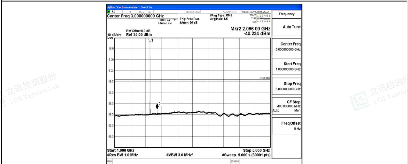
Band25-3MHz-16QAM-26675-1-0-High-1000-5000--40.23-PASS
