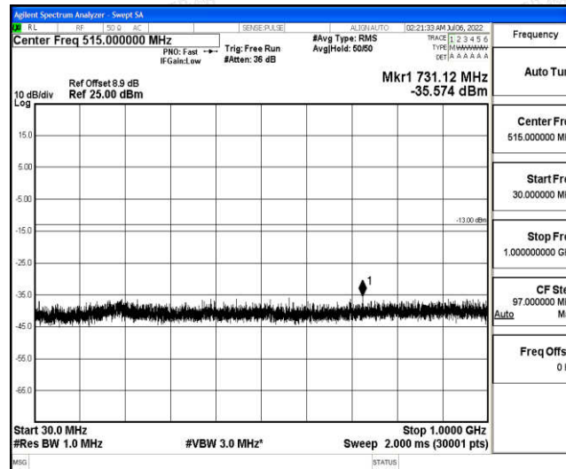
Band25-10MHz-QPSK-26640-1-0-High-30-1000--35.57-PASS
