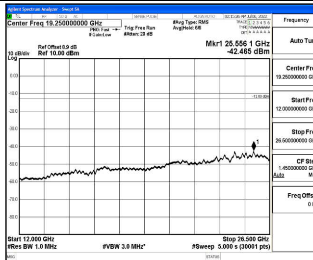
Band25-10MHz-QPSK-26090-1-0-Low-12000-26500--42.47-PASS
