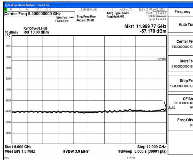
Band25-3MHz-16QAM-26055-1-0-Low-5000-12000--57.18-PASS
