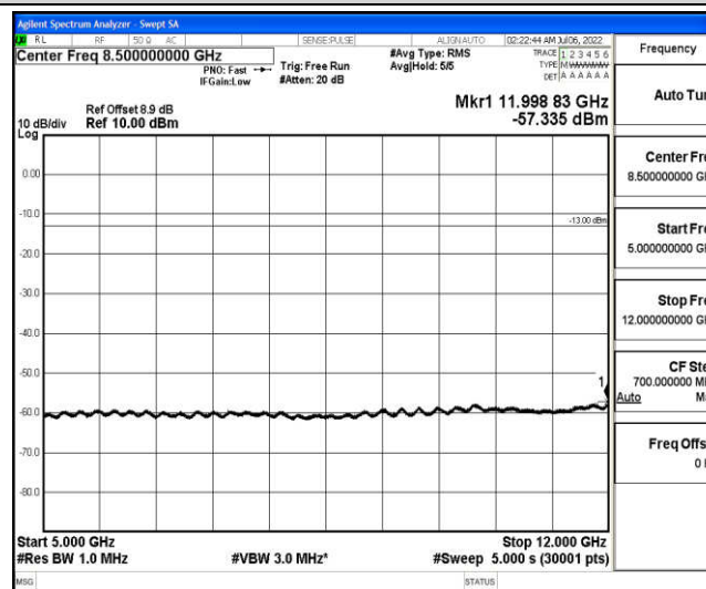
Band25-10MHz-QPSK-26640-1-0-High-5000-12000--57.34-PASS
