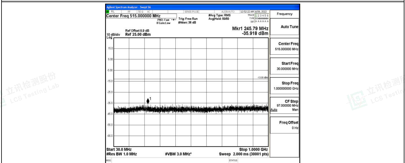
Band25-1.4MHz-16QAM-26047-1-0-Low-30-1000--35.92-PASS
