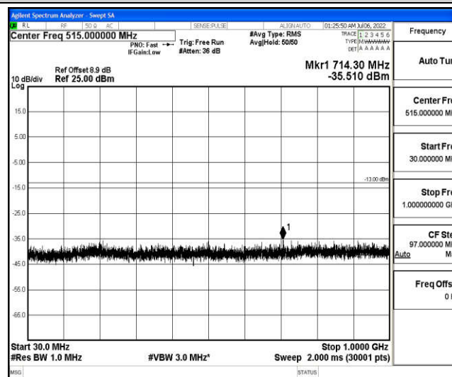
Band25-3MHz-16QAM-26365-1-0-Low-30-1000--35.51-PASS
