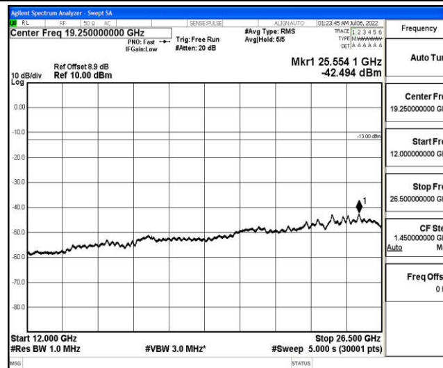
Band25-3MHz-16QAM-26055-1-0-Low-12000-26500--42.49-PASS
