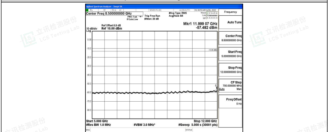
Band25-3MHz-16QAM-26675-1-0-High-5000-12000--57.48-PASS
