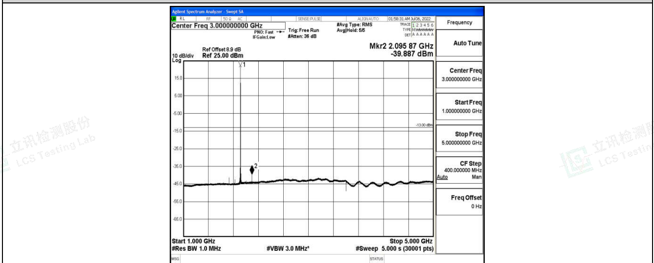
Band25-5MHz-16QAM-26665-1-0-High-1000-5000--39.89-PASS
