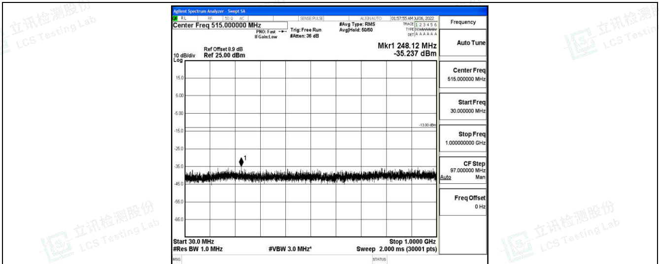
Band25-5MHz-16QAM-26665-1-0-High-30-1000--35.24-PASS
