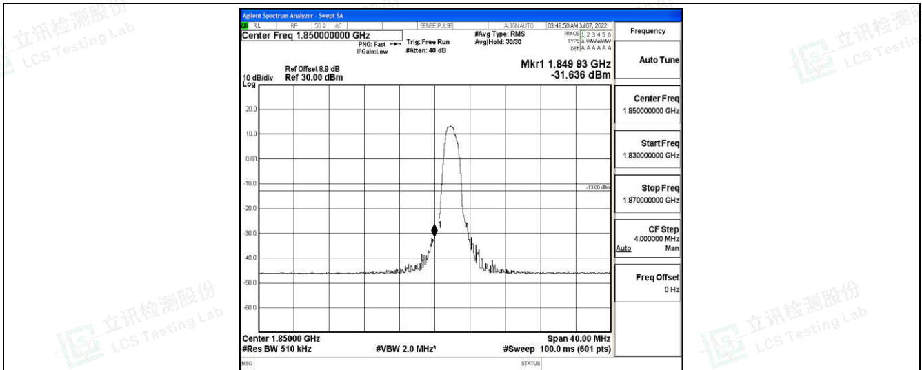
Band25-20MHz-QPSK-26140-6-0-Low--31.64-PASS
