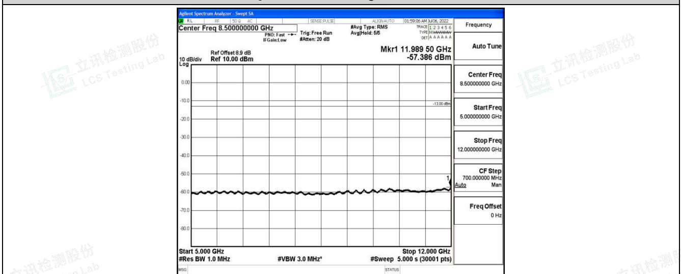
Band25-5MHz-16QAM-26665-1-0-High-5000-12000--57.39-PASS
