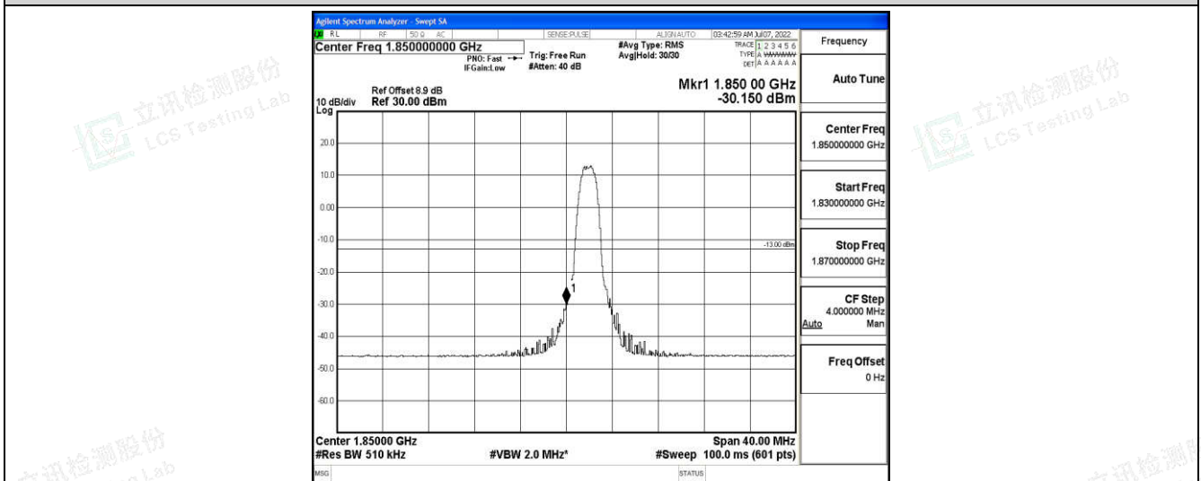
Band25-20MHz-16QAM-26140-6-0-Low--30.15-PASS
