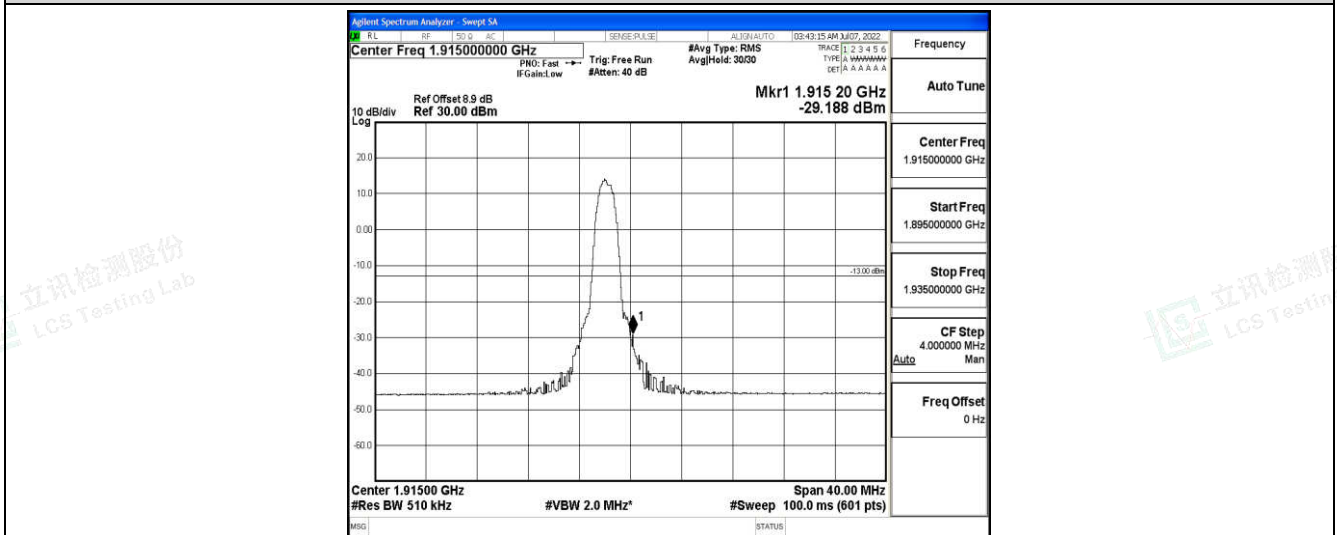
Band25-20MHz-QPSK-26590-6-0-High--29.19-PASS
