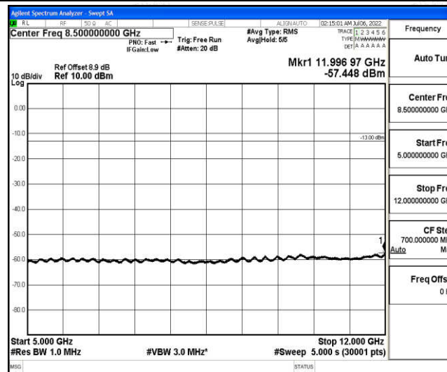
Band25-10MHz-QPSK-26090-1-0-Low-5000-12000--57.45-PASS
