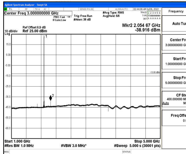
Band25-15MHz-16QAM-26365-1-0-Low-1000-5000--38.92-PASS
