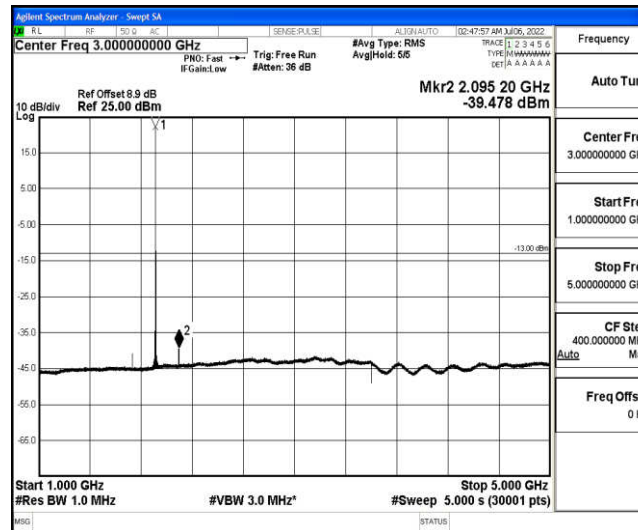
Band25-15MHz-16QAM-26615-1-0-High-1000-5000--39.48-PASS
