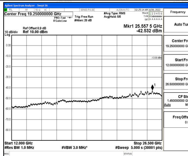
Band25-10MHz-16QAM-26640-1-0-High-12000-26500--42.53-PASS
