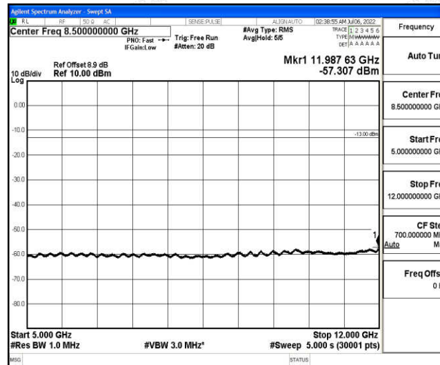
Band25-15MHz-QPSK-26115-1-0-Low-5000-12000--57.31-PASS
