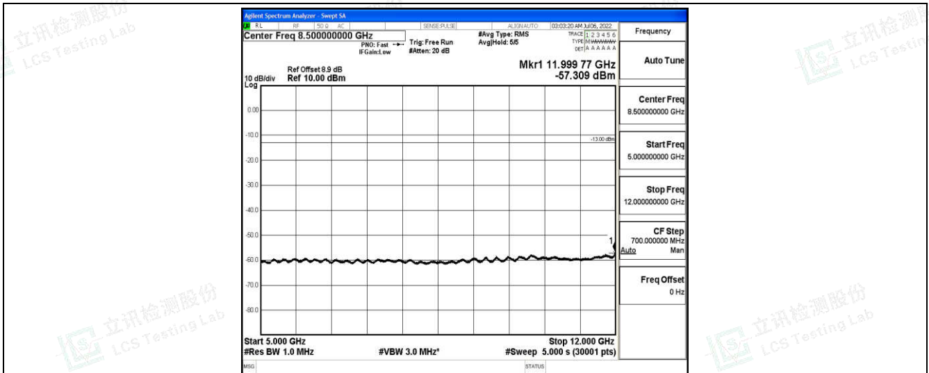
Band25-20MHz-QPSK-26140-1-0-Low-5000-12000--57.31-PASS
