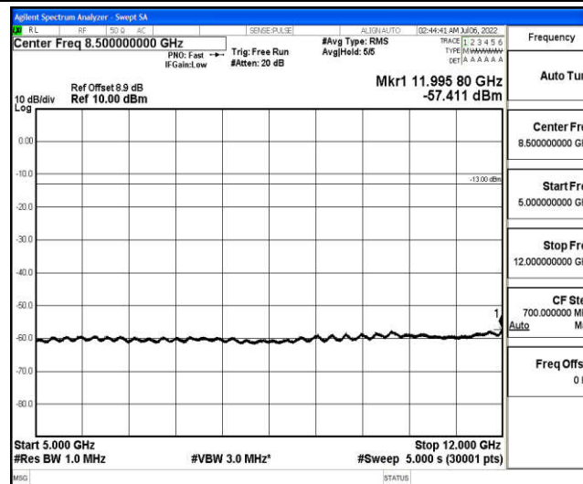
Band25-15MHz-16QAM-26365-1-0-Low-5000-12000--57.41-PASS
