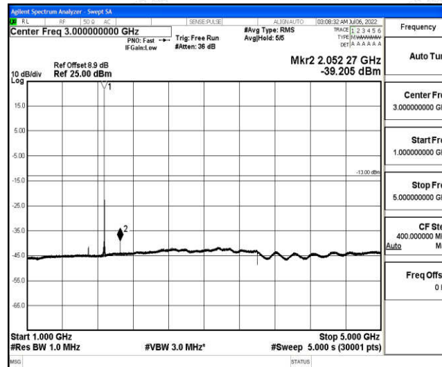
Band25-20MHz-16QAM-26365-1-0-Low-1000-5000--39.21-PASS
