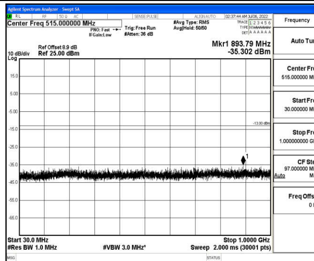
Band25-15MHz-QPSK-26115-1-0-Low-30-1000--35.3-PASS
