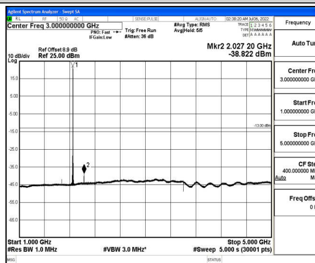
Band25-15MHz-QPSK-26115-1-0-Low-1000-5000--38.82-PASS
