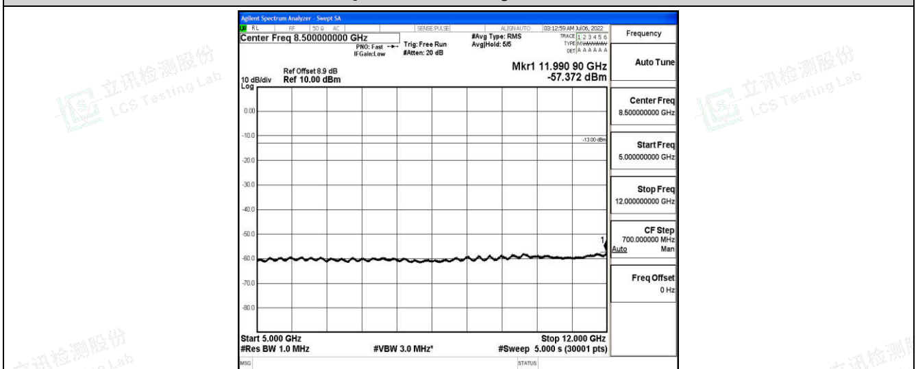
Band25-20MHz-16QAM-26590-1-0-High-5000-12000--57.37-PASS
