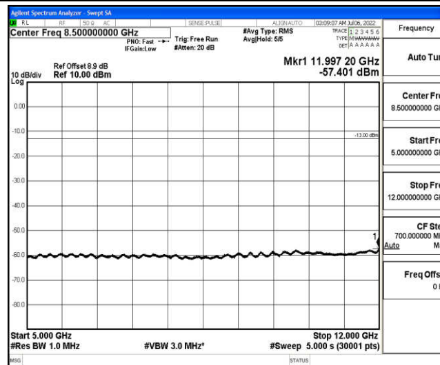
Band25-20MHz-16QAM-26365-1-0-Low-5000-12000--57.4-PASS
