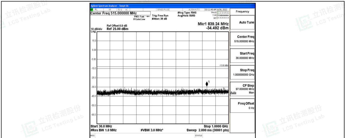
Band25-20MHz-16QAM-26590-1-0-High-30-1000--34.49-PASS
