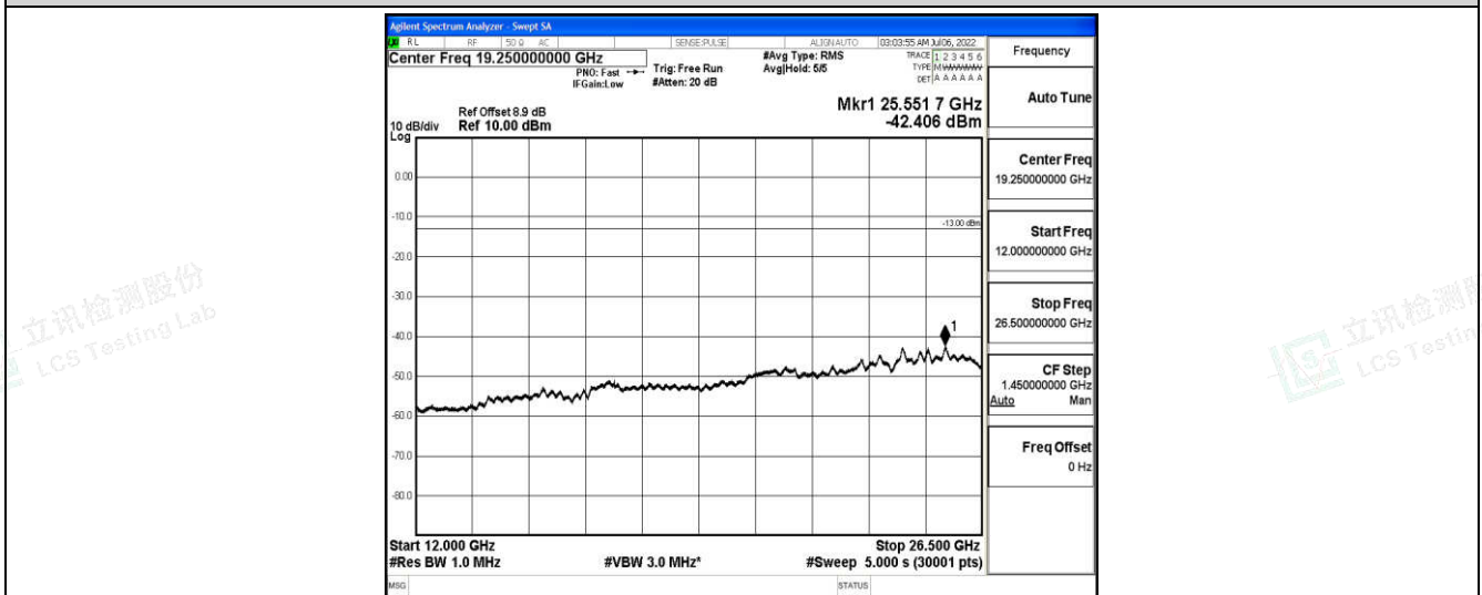
Band25-20MHz-QPSK-26140-1-0-Low-12000-26500--42.41-PASS
