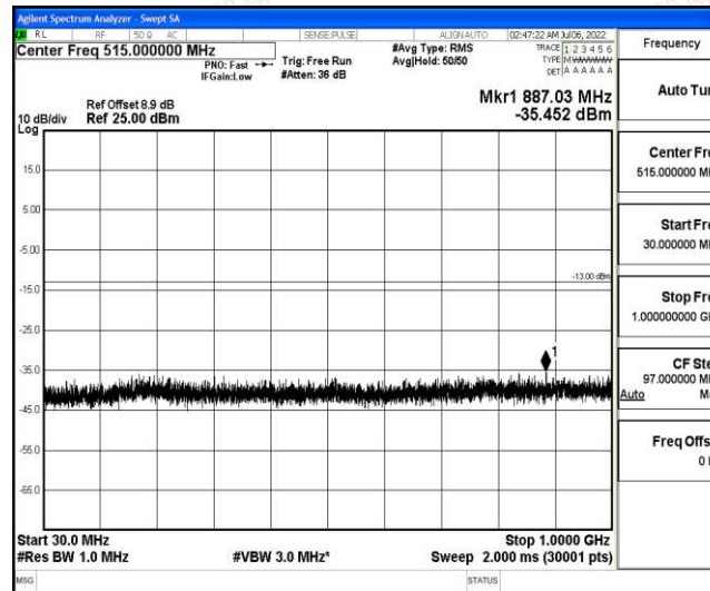
Band25-15MHz-16QAM-26615-1-0-High-30-1000--35.45-PASS
