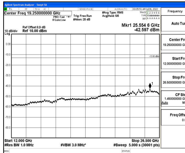
Band25-20MHz-16QAM-26140-1-0-Low-12000-26500--42.6-PASS
