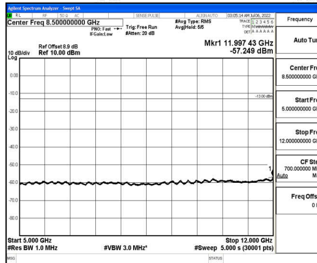
Band25-20MHz-16QAM-26140-1-0-Low-5000-12000--57.25-PASS
