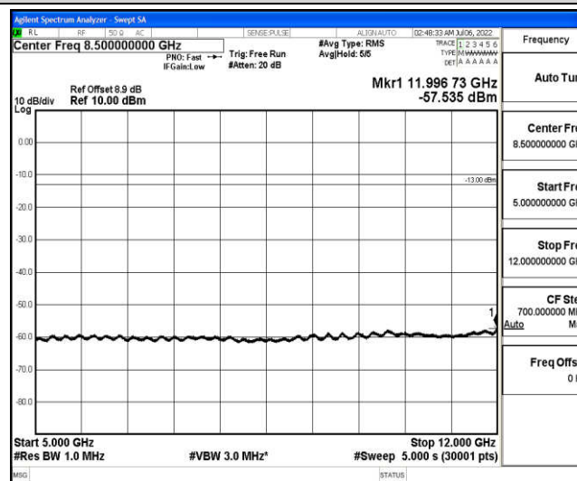
Band25-15MHz-16QAM-26615-1-0-High-5000-12000--57.54-PASS
