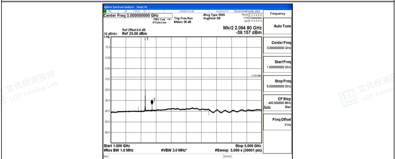
Band25-20MHz-16QAM-26590-1-0-High-1000-5000--39.16-PASS
