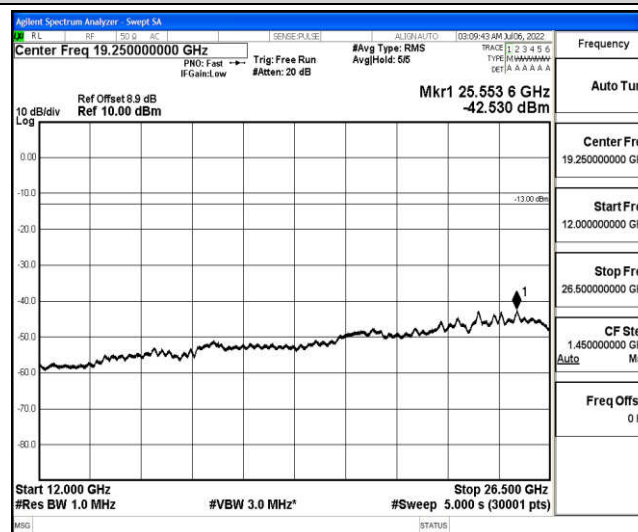
Band25-20MHz-16QAM-26365-1-0-Low-12000-26500--42.53-PASS
