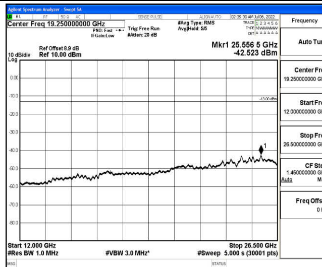
Band25-15MHz-QPSK-26115-1-0-Low-12000-26500--42.52-PASS
