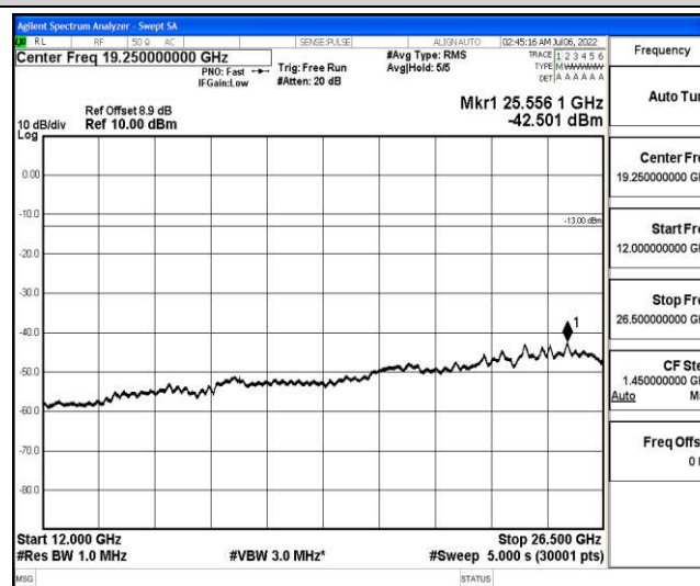
Band25-15MHz-16QAM-26365-1-0-Low-12000-26500--42.5-PASS
