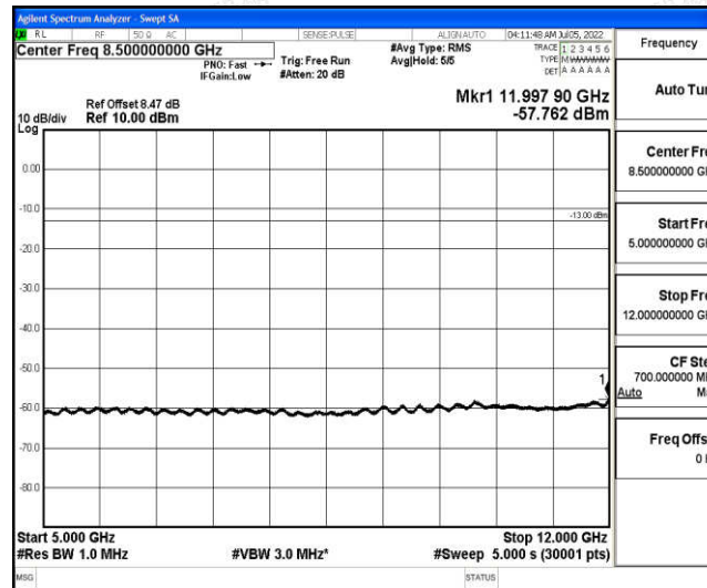
Band66-3MHz-16QAM-131987-1-0-Low-5000-12000--57.76-PASS
