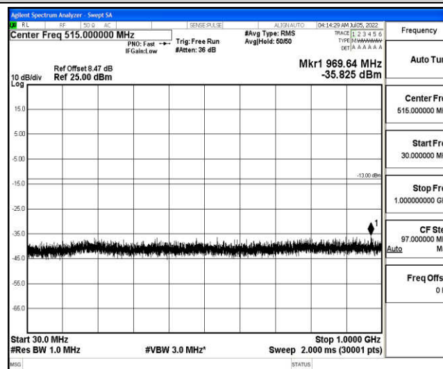
Band66-3MHz-16QAM-132322-1-0-Low-30-1000--35.83-PASS
