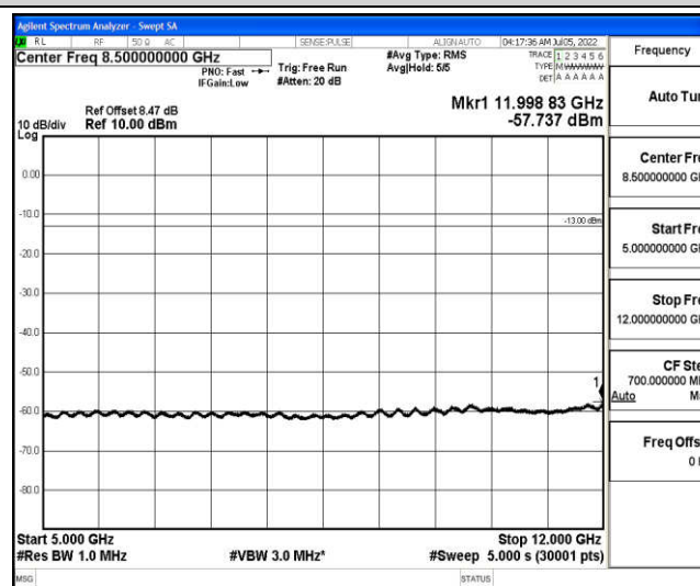
Band66-3MHz-QPSK-132657-1-0-High-5000-12000--57.74-PASS
