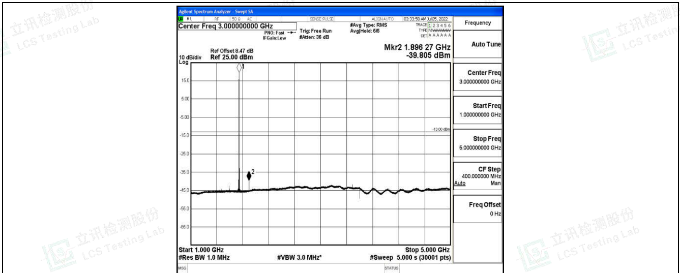
Band66-1.4MHz-QPSK-132322-1-0-Low-1000-5000--39.81-PASS
