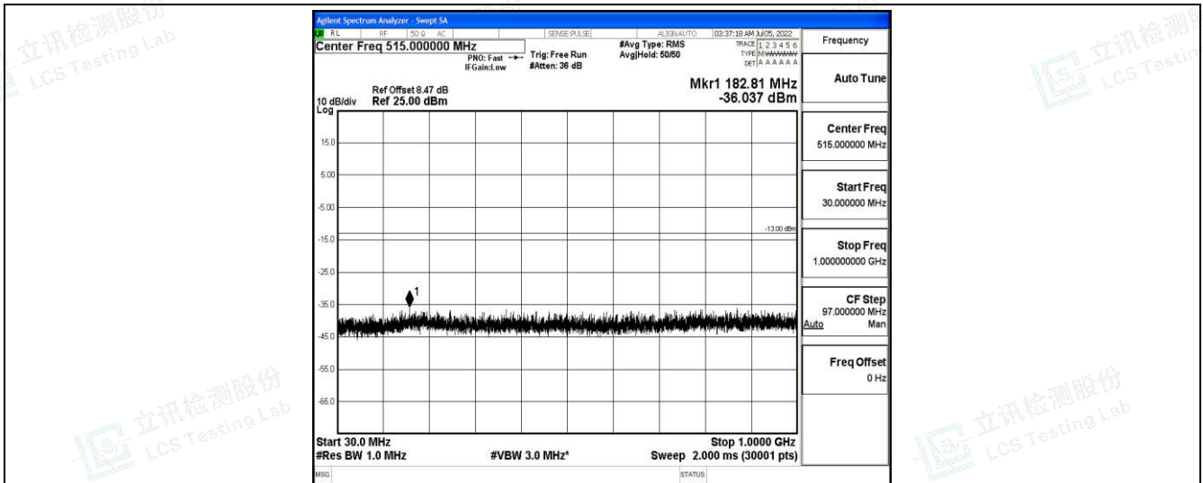
Band66-1.4MHz-QPSK-132665-1-0-High-30-1000--36.04-PASS
