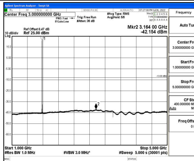
Band66-10MHz-16QAM-132622-1-0-High-1000-5000--42.15-PASS
