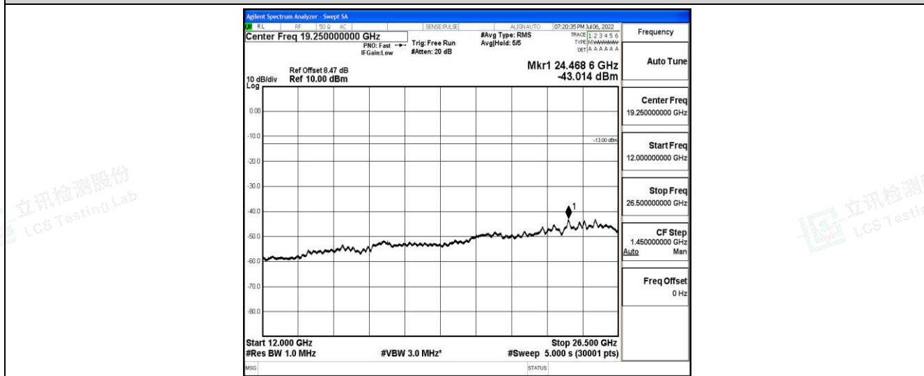
Band66-10MHz-16QAM-132022-1-0-Low-12000-26500--43.01-PASS
