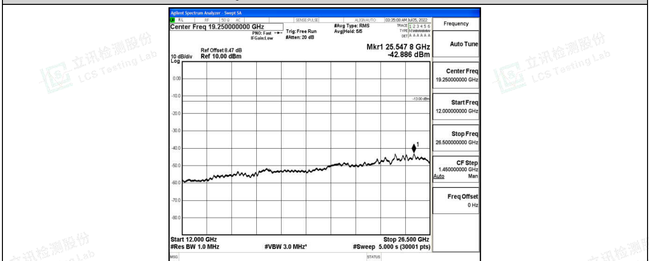
Band66-1.4MHz-QPSK-132322-1-0-Low-12000-26500--42.89-PASS
