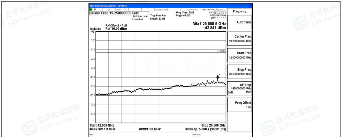
Band66-5MHz-16QAM-132647-1-0-High-12000-26500--42.84-PASS
