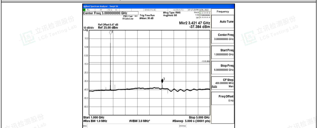
Band66-10MHz-QPSK-132022-1-0-Low-1000-5000--37.38-PASS
