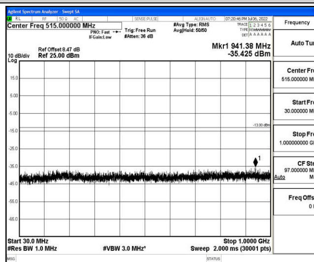
Band66-10MHz-QPSK-132322-1-0-Low-30-1000--35.43-PASS
