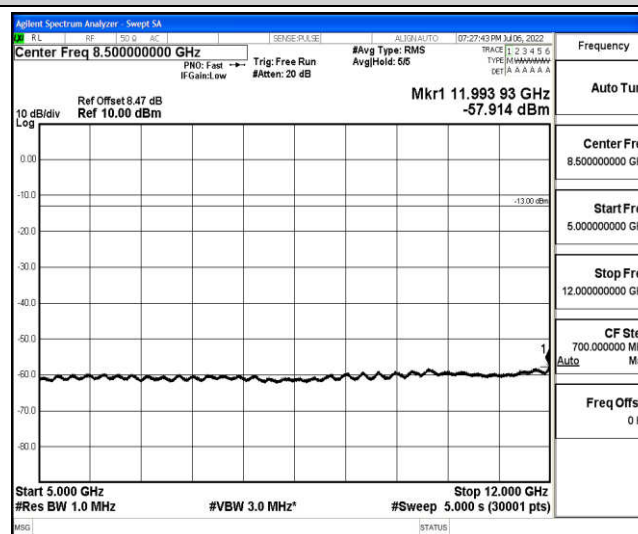
Band66-10MHz-16QAM-132622-1-0-High-5000-12000--57.91-PASS
