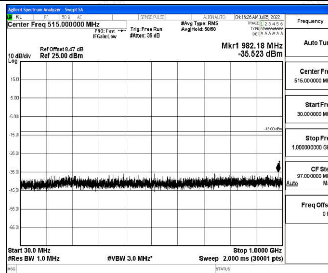
Band66-3MHz-QPSK-132657-1-0-High-30-1000--35.52-PASS
