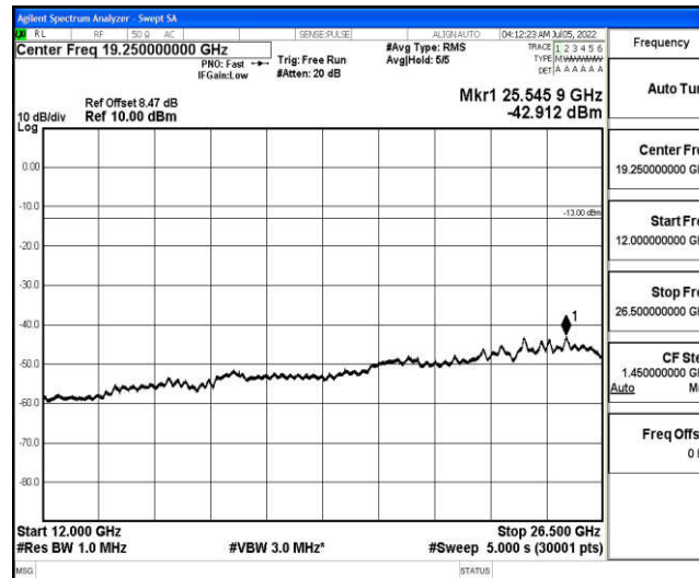
Band66-3MHz-16QAM-131987-1-0-Low-12000-26500--42.91-PASS
