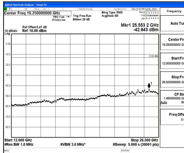
Band66-15MHz-QPSK-132047-1-0-Low-12000-26500--42.84-PASS
