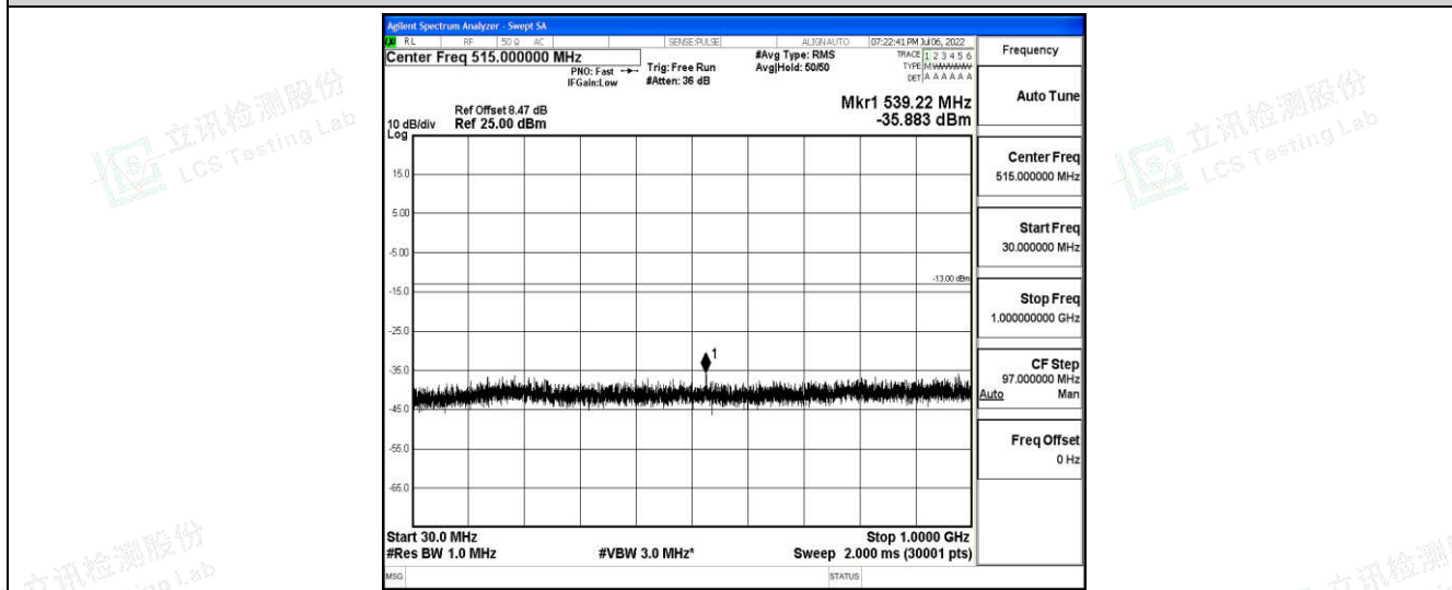
Band66-10MHz-16QAM-132322-1-0-Low-30-1000--35.88-PASS
