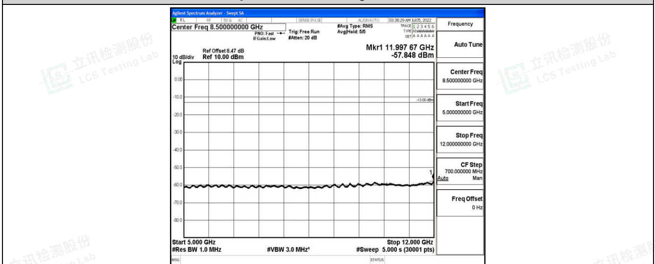
Band66-1.4MHz-QPSK-132665-1-0-High-5000-12000--57.85-PASS
