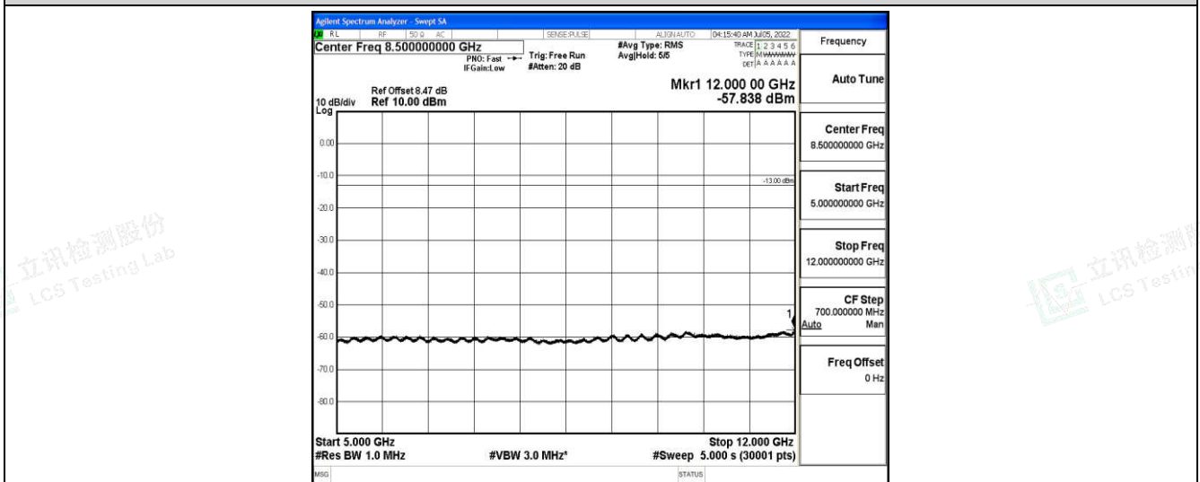
Band66-3MHz-16QAM-132322-1-0-Low-5000-12000--57.84-PASS
