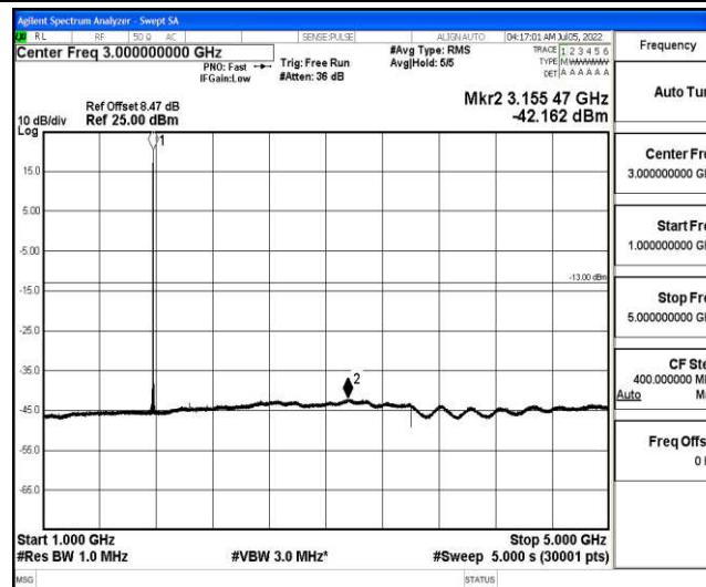
Band66-3MHz-QPSK-132657-1-0-High-1000-5000--42.16-PASS
