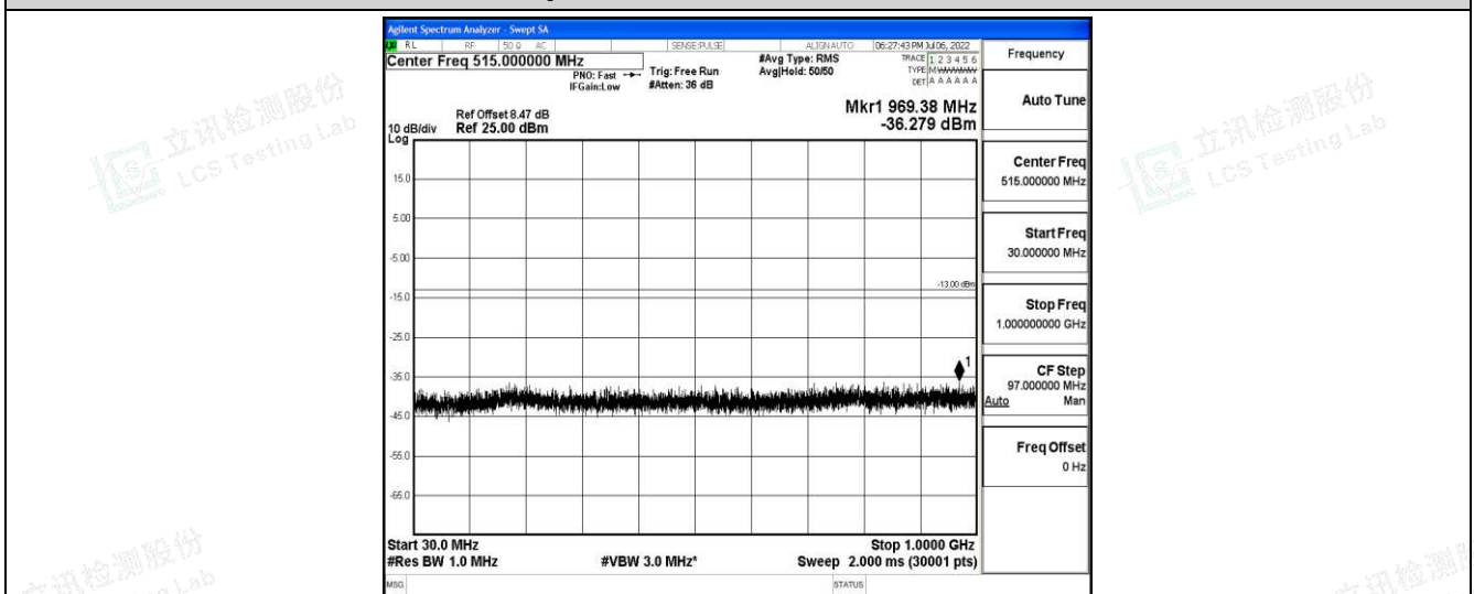
Band66-15MHz-16QAM-132322-1-0-Low-30-1000--36.28-PASS
