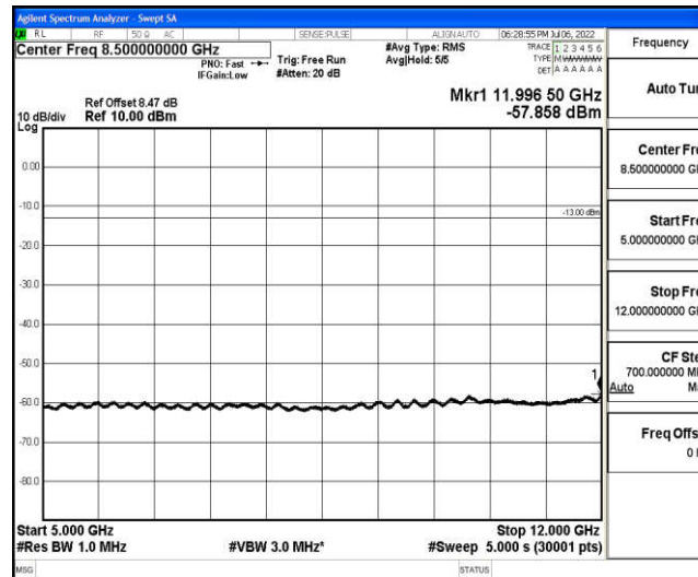
Band66-15MHz-16QAM-132322-1-0-Low-5000-12000--57.86-PASS
