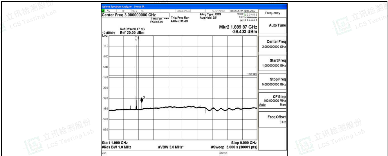
Band66-15MHz-QPSK-132322-1-0-Low-1000-5000--39.4-PASS
