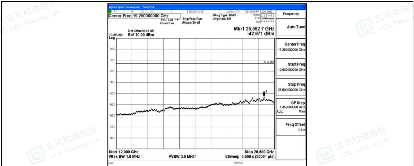
Band66-15MHz-16QAM-132597-1-0-High-12000-26500--42.97-PASS
