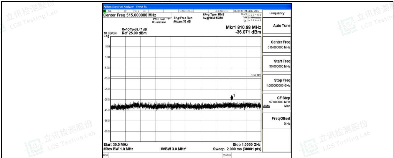
Band66-15MHz-QPSK-132597-1-0-High-30-1000--36.07-PASS
