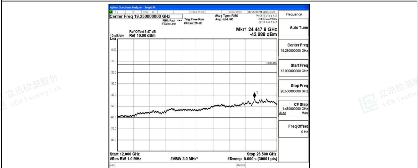
Band66-15MHz-16QAM-132047-1-0-Low-12000-26500--42.99-PASS
