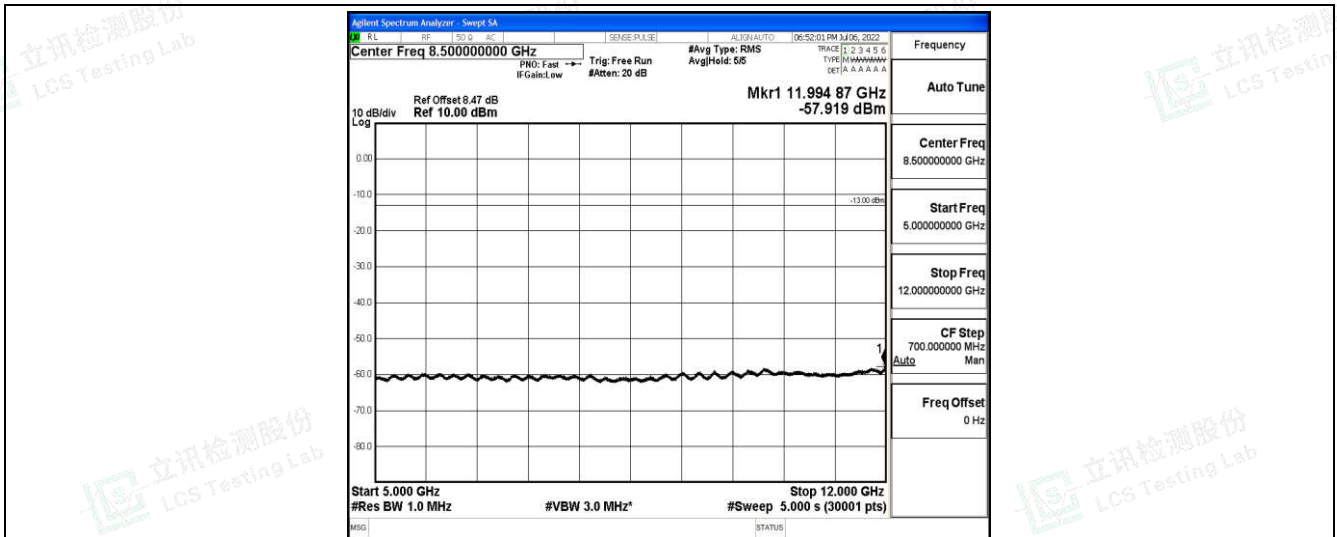
Band66-20MHz-QPSK-132072-1-0-Low-5000-12000--57.92-PASS
