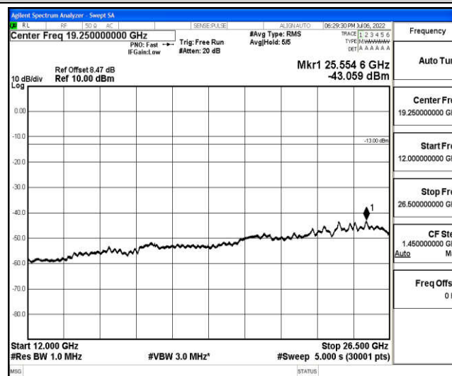
Band66-15MHz-16QAM-132322-1-0-Low-12000-26500--43.06-PASS
