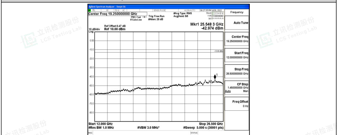
Band66-15MHz-QPSK-132322-1-0-Low-12000-26500--42.97-PASS
