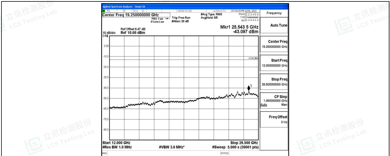
Band66-20MHz-QPSK-132572-1-0-High-12000-26500--43.1-PASS
