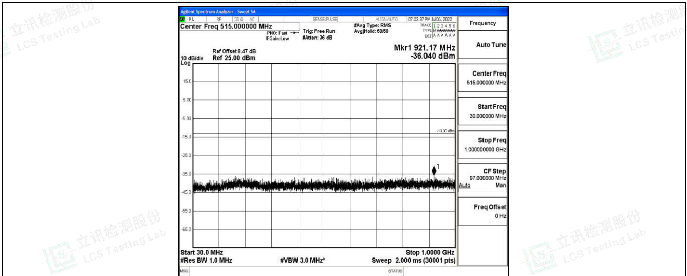
Band66-20MHz-16QAM-132572-1-0-High-30-1000--36.04-PASS
