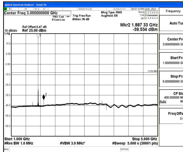
Band66-20MHz-16QAM-132322-1-0-Low-1000-5000--39.53-PASS
