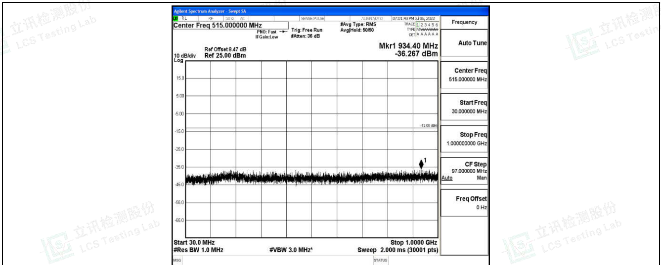
Band66-20MHz-QPSK-132572-1-0-High-30-1000--36.27-PASS
