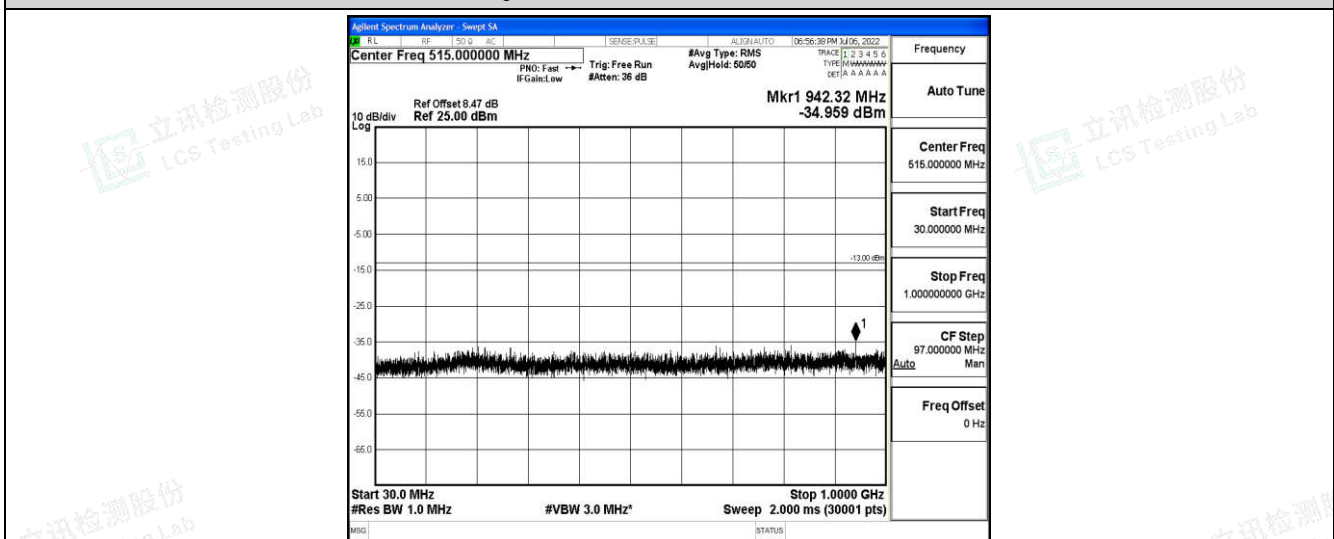
Band66-20MHz-16QAM-132322-1-0-Low-30-1000--34.96-PASS
