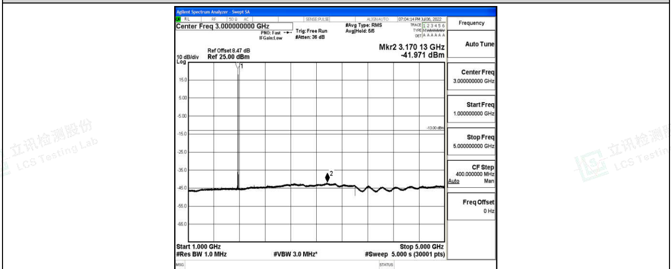
Band66-20MHz-16QAM-132572-1-0-High-1000-5000--41.97-PASS
