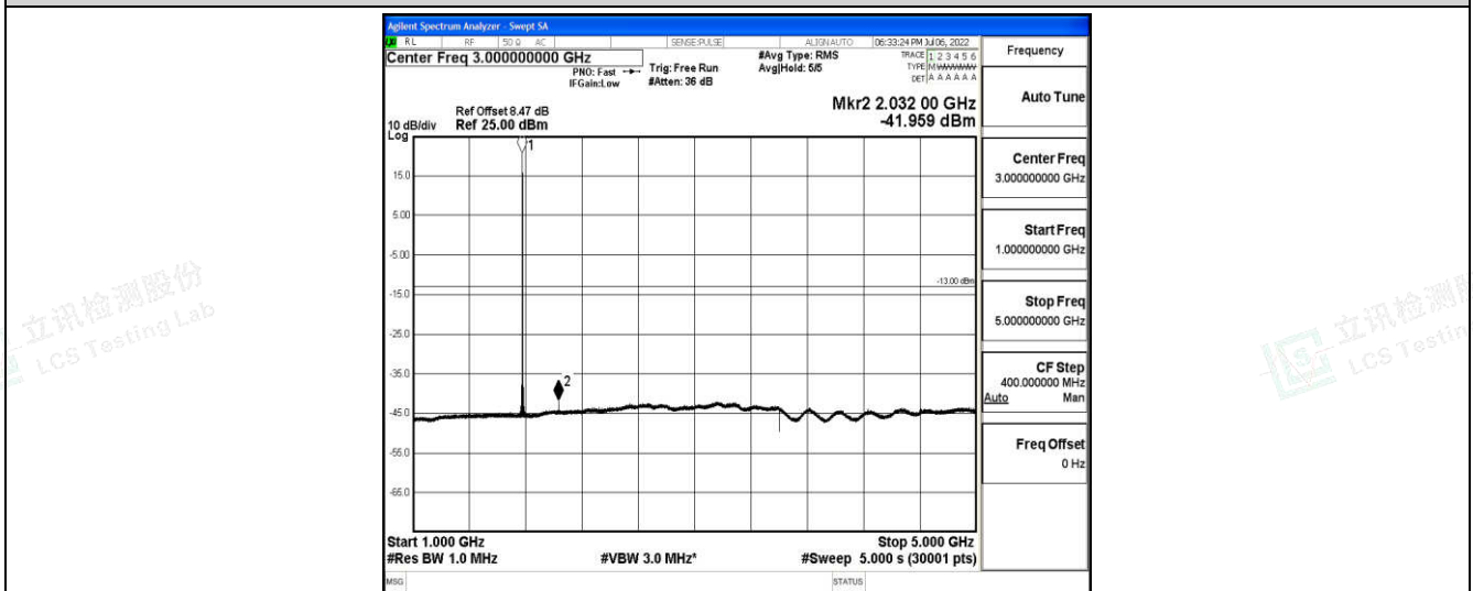
Band66-15MHz-QPSK-132597-1-0-High-1000-5000--41.96-PASS
