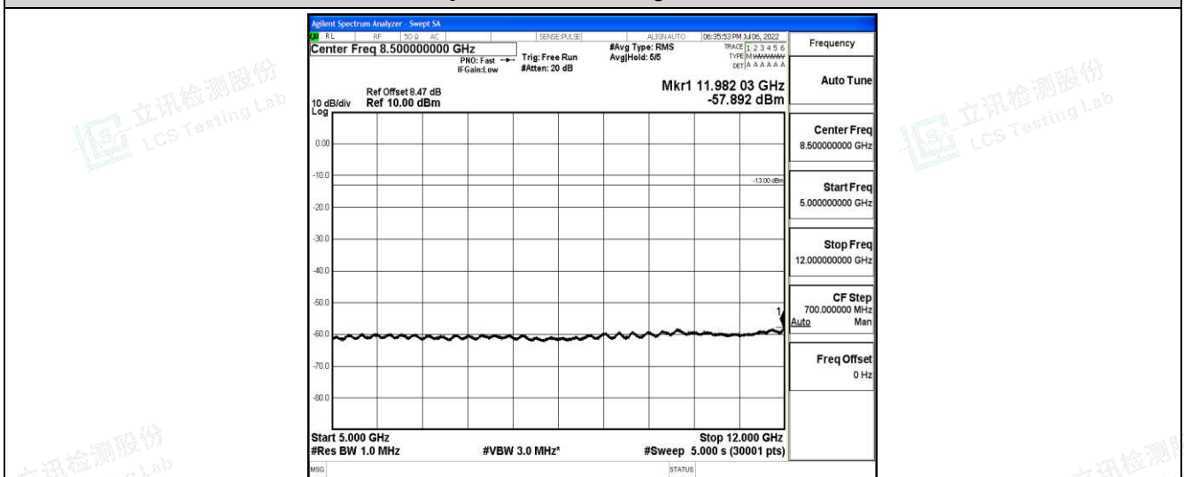
Band66-15MHz-16QAM-132597-1-0-High-5000-12000--57.89-PASS
