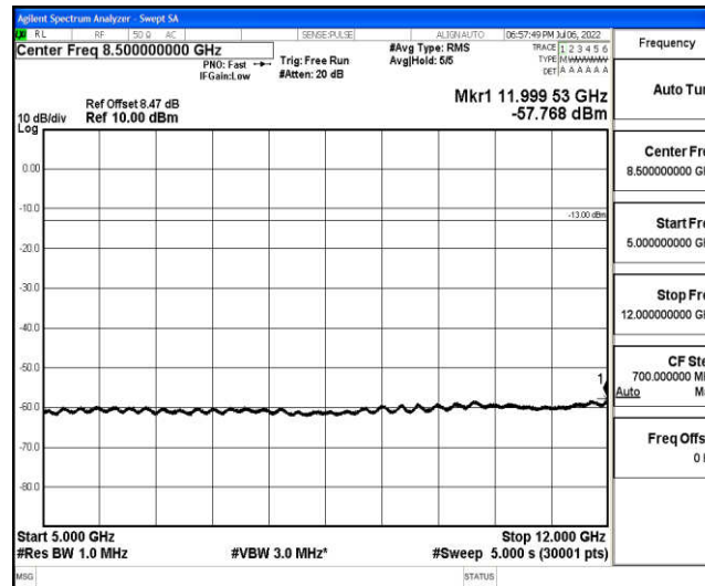
Band66-20MHz-16QAM-132322-1-0-Low-5000-12000--57.77-PASS
