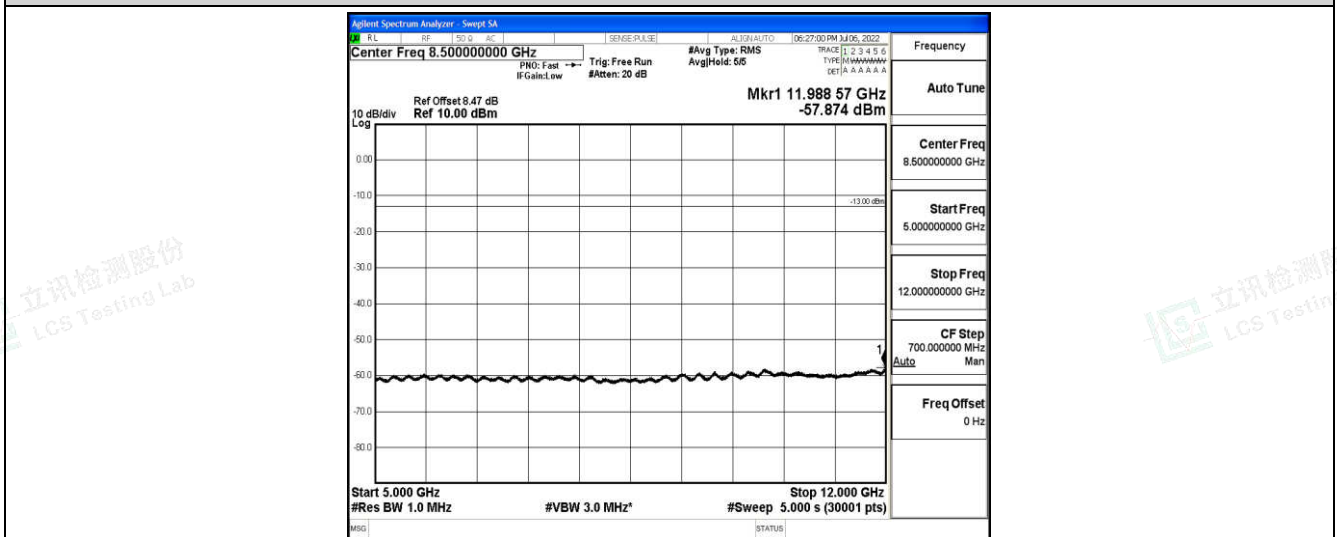
Band66-15MHz-QPSK-132322-1-0-Low-5000-12000--57.87-PASS
