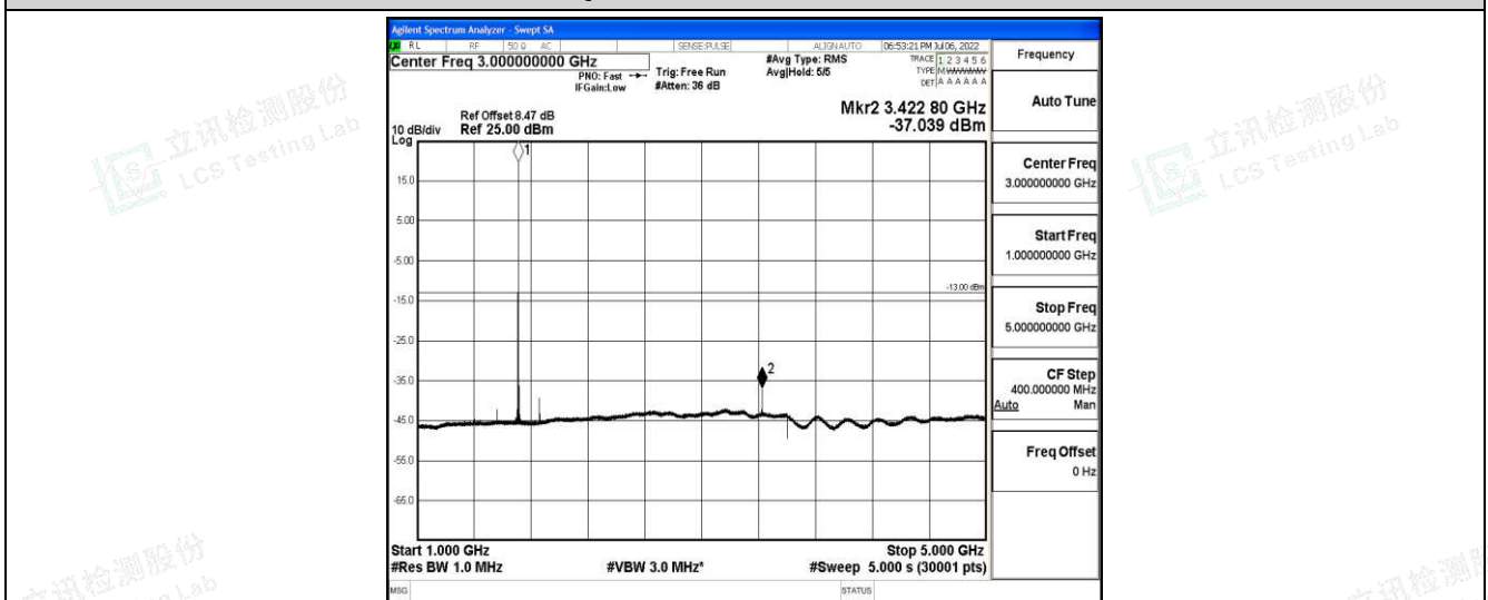
Band66-20MHz-16QAM-132072-1-0-Low-1000-5000--37.04-PASS
