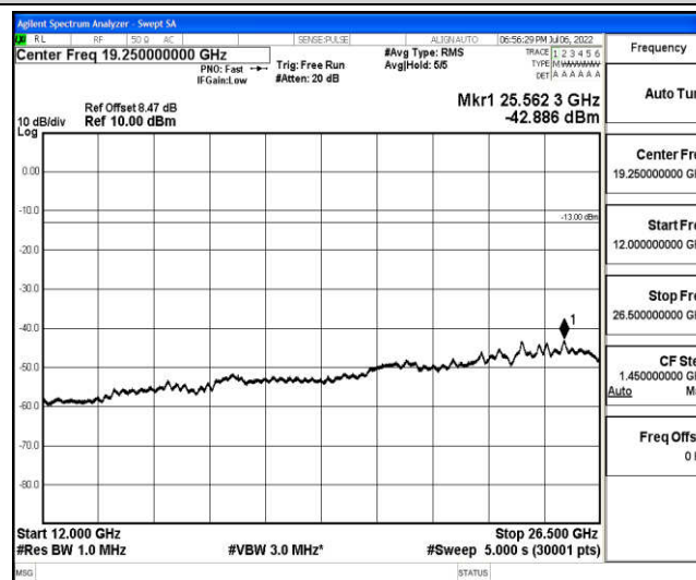
Band66-20MHz-QPSK-132322-1-0-Low-12000-26500--42.89-PASS
