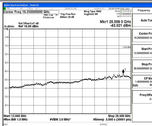
Band66-20MHz-16QAM-132322-1-0-Low-12000-26500--43.02-PASS
