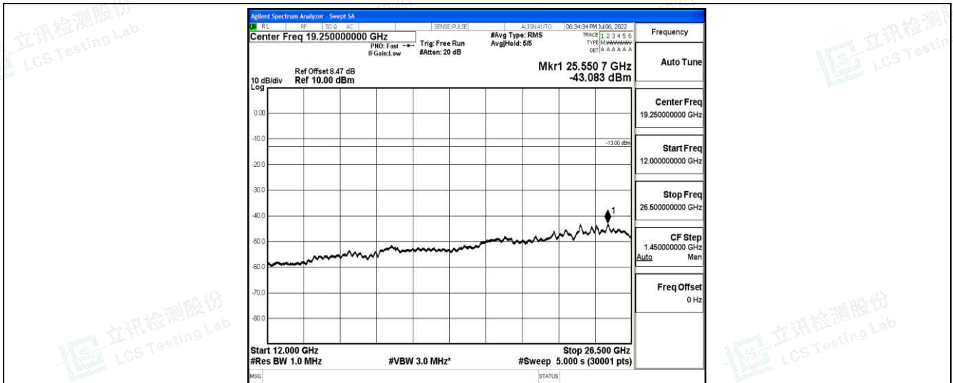
Band66-15MHz-QPSK-132597-1-0-High-12000-26500--43.08-PASS
