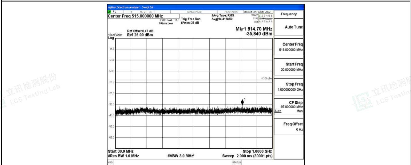
Band66-15MHz-16QAM-132047-1-0-Low-30-1000--35.84-PASS
