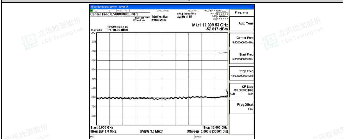
Band66-15MHz-QPSK-132597-1-0-High-5000-12000--57.82-PASS
