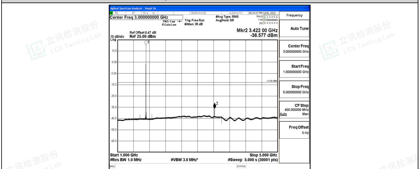
Band66-15MHz-16QAM-132047-1-0-Low-1000-5000--36.58-PASS
