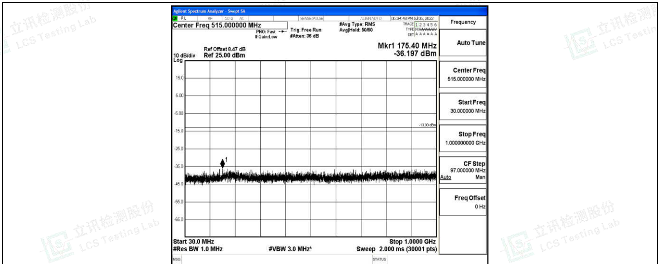
Band66-15MHz-16QAM-132597-1-0-High-30-1000--36.2-PASS
