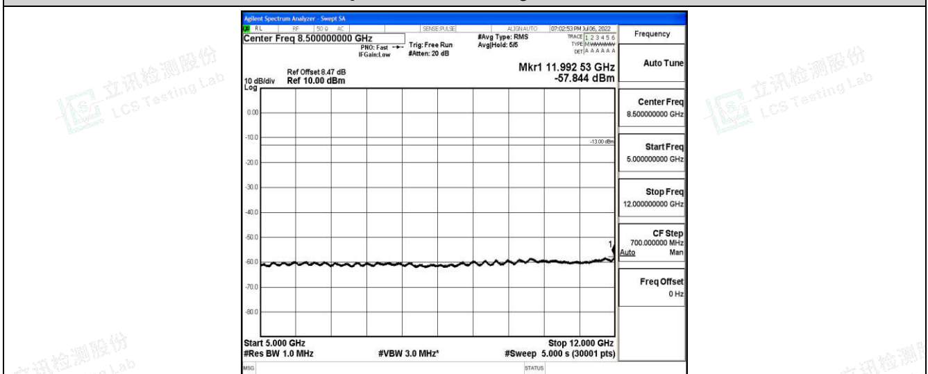
Band66-20MHz-QPSK-132572-1-0-High-5000-12000--57.84-PASS
