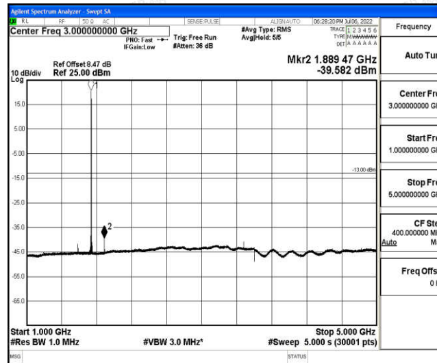
Band66-15MHz-16QAM-132322-1-0-Low-1000-5000--39.58-PASS
