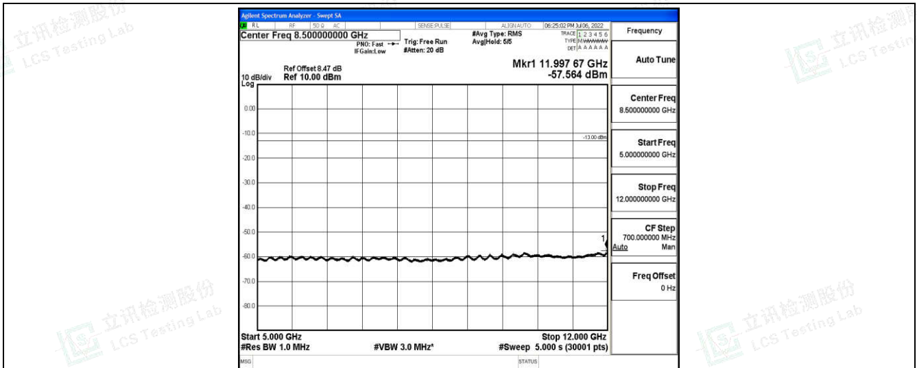
Band66-15MHz-16QAM-132047-1-0-Low-5000-12000--57.56-PASS
