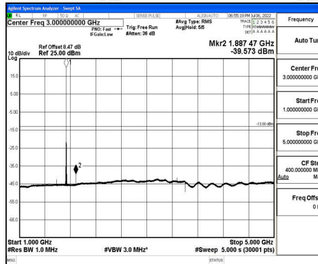
Band66-20MHz-QPSK-132322-1-0-Low-1000-5000--39.57-PASS
