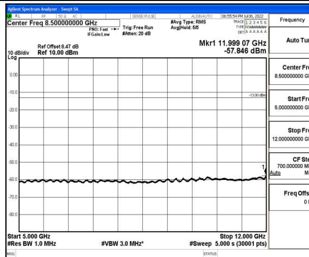
Band66-20MHz-QPSK-132322-1-0-Low-5000-12000--57.85-PASS
