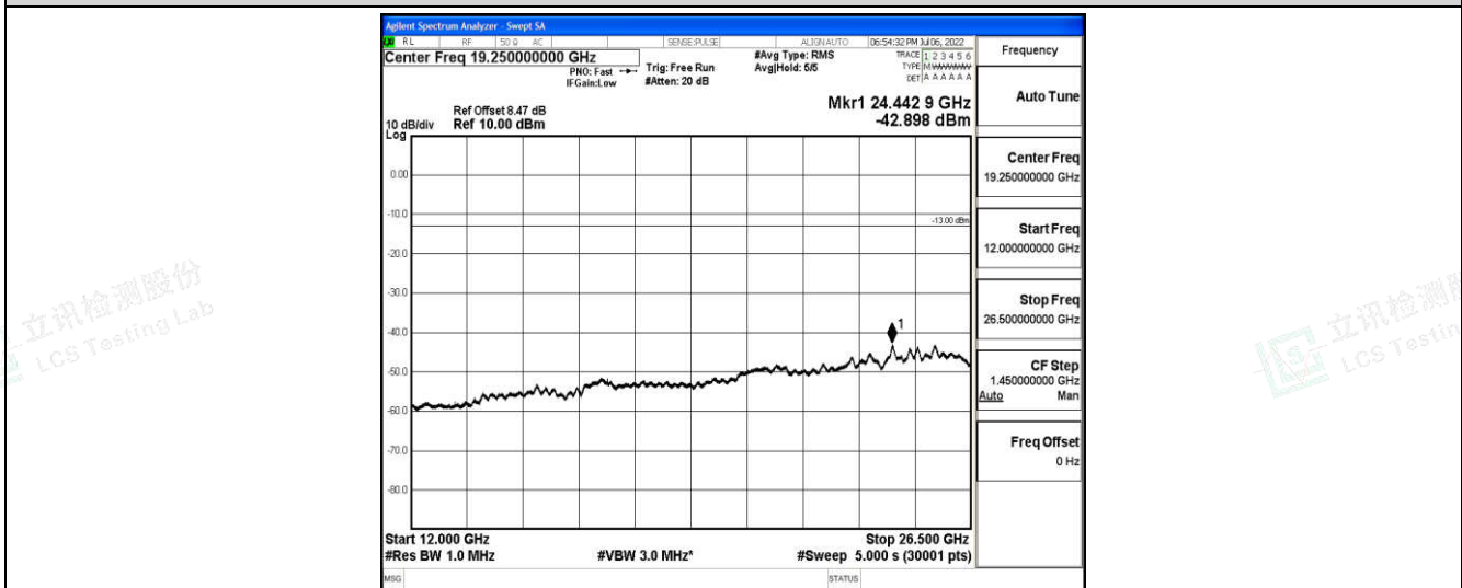
Band66-20MHz-16QAM-132072-1-0-Low-12000-26500--42.9-PASS
