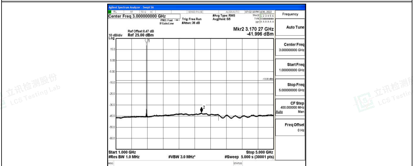
Band66-20MHz-QPSK-132572-1-0-High-1000-5000--42-PASS
