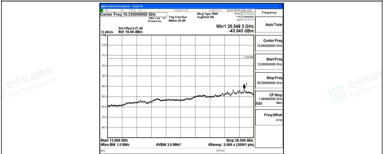
Band66-20MHz-QPSK-132072-1-0-Low-12000-26500--43.04-PASS
