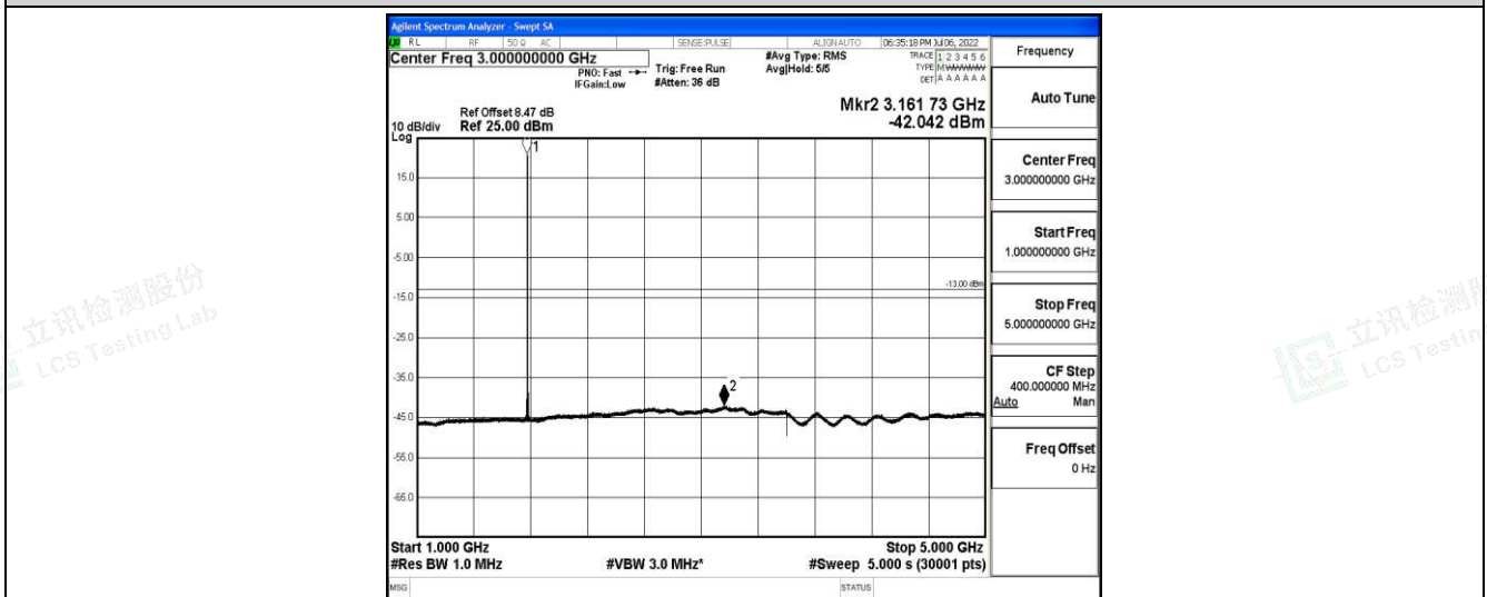
Band66-15MHz-16QAM-132597-1-0-High-1000-5000--42.04-PASS
