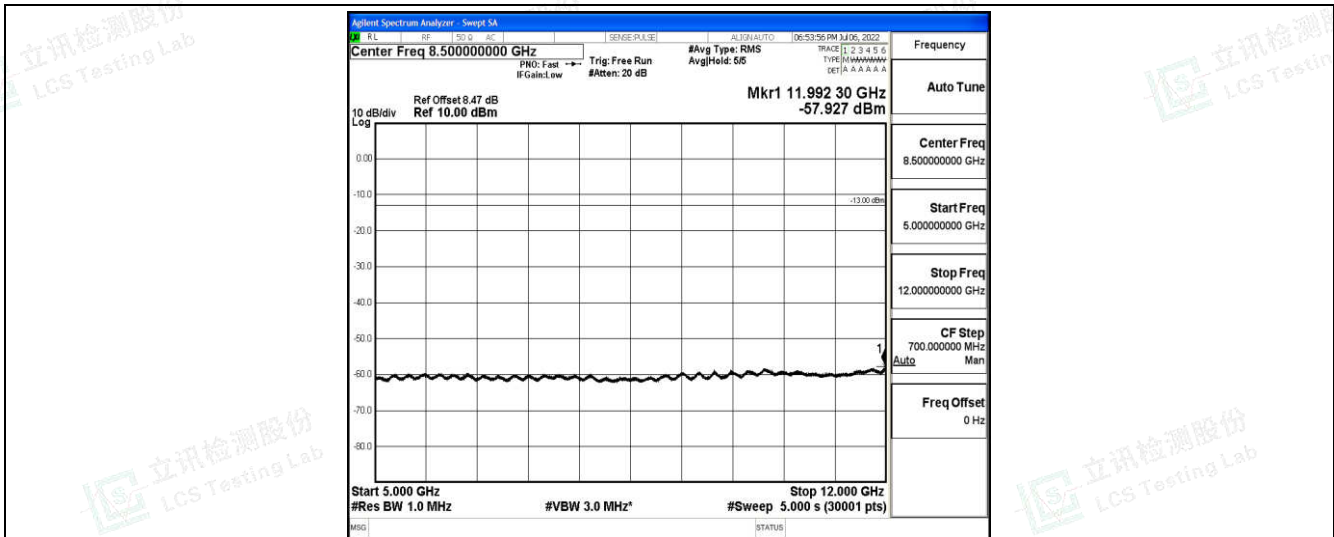
Band66-20MHz-16QAM-132072-1-0-Low-5000-12000--57.93-PASS
