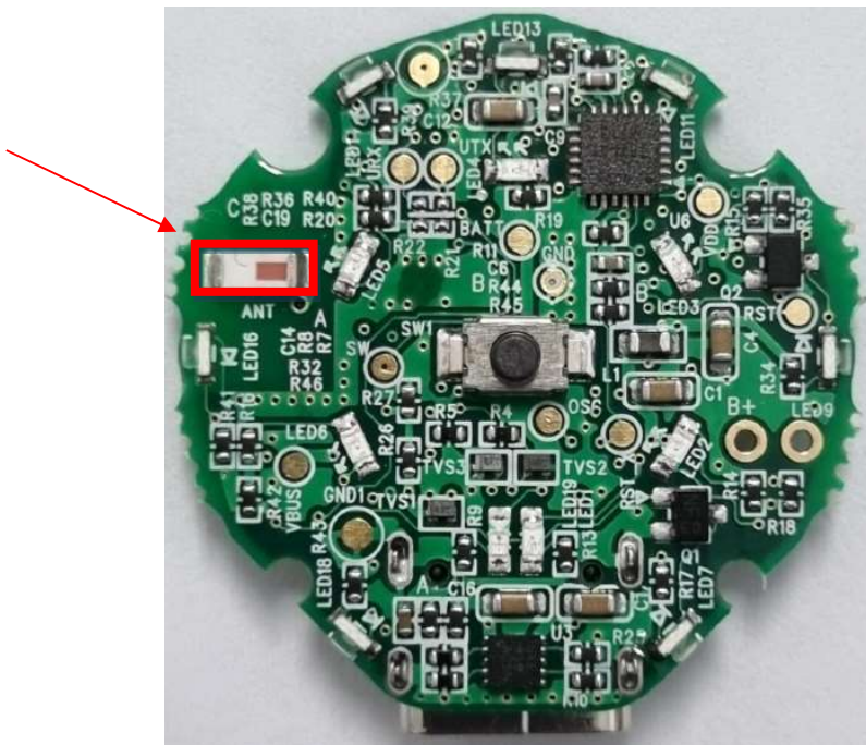
Main board - Front Top
