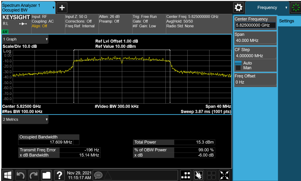
Figure 6: 802.11n(HT20), 5825MHz
