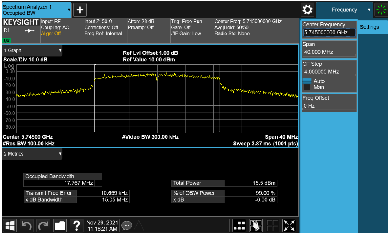
Figure 7: 802.11ac(VHT20), 5745MHz
