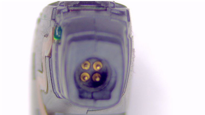
Internal photo of hearing aid with antenna, Rear view
