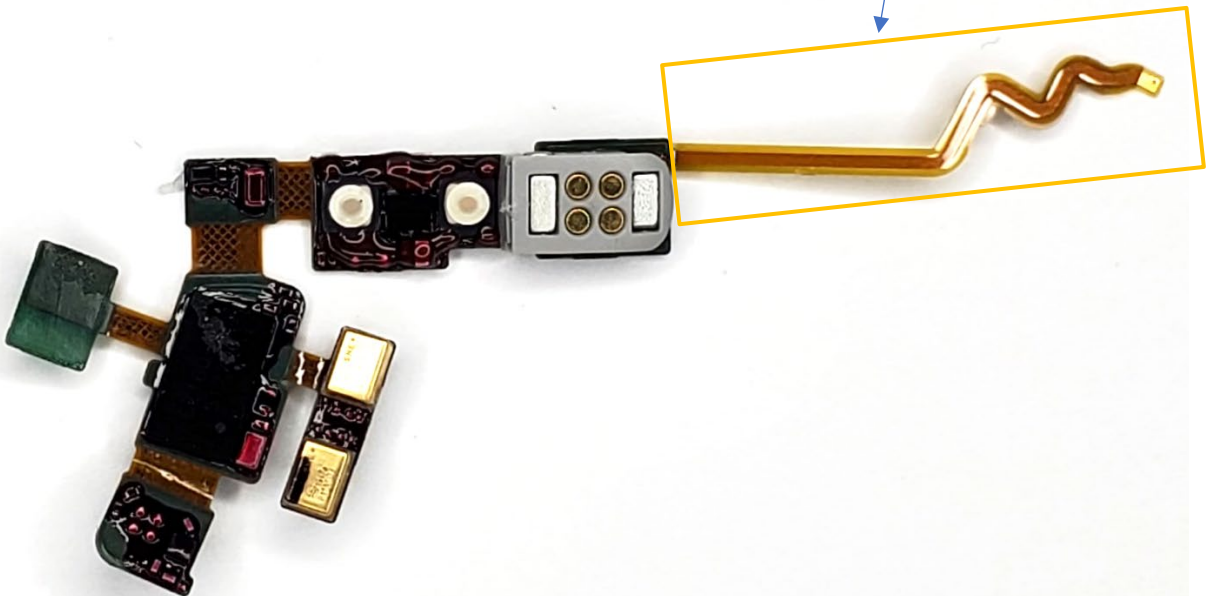
Coated PCBA with Antenna – Top View
