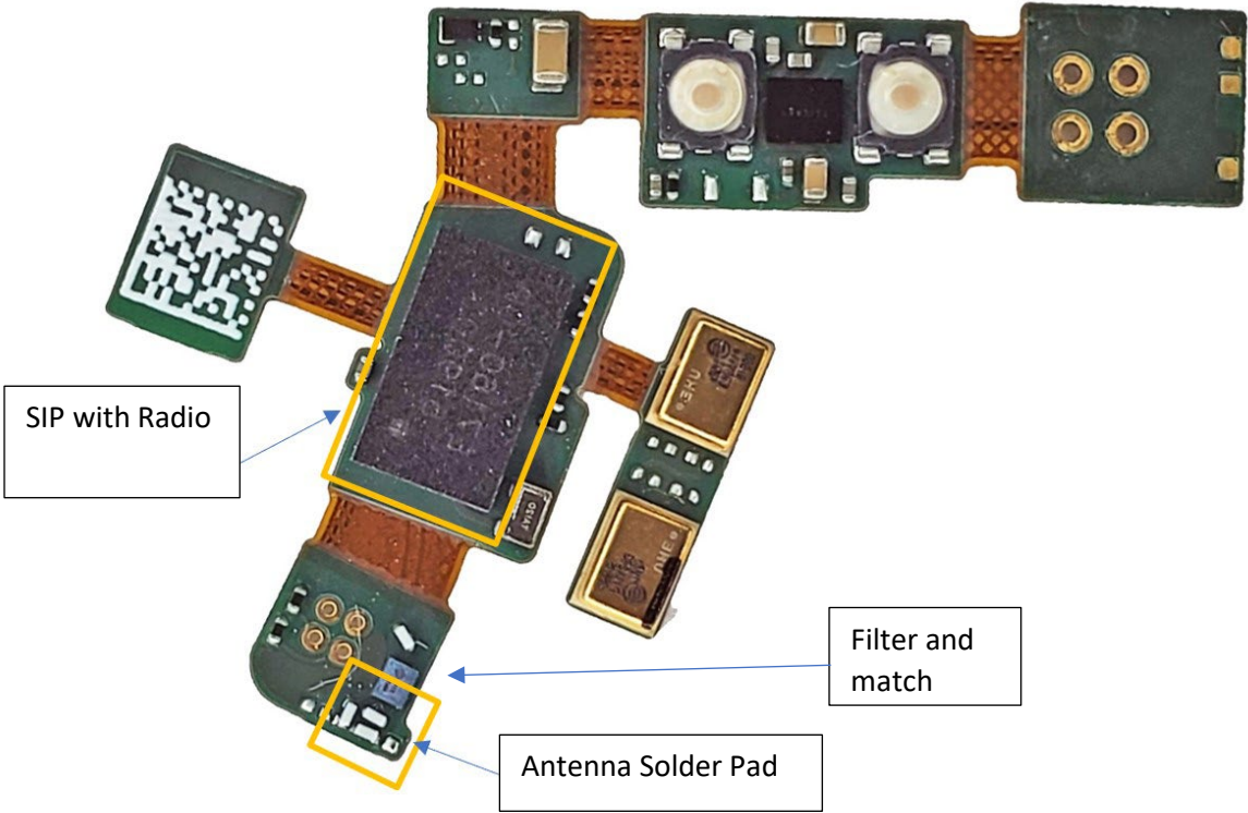
Uncoated PCBA – Top View
