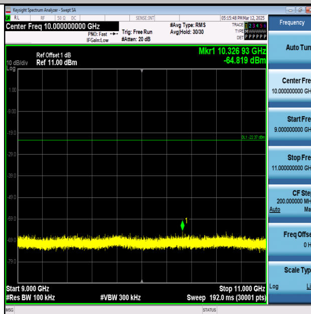
BLE_125K-Ant1-2402-9000~11000-PASS
