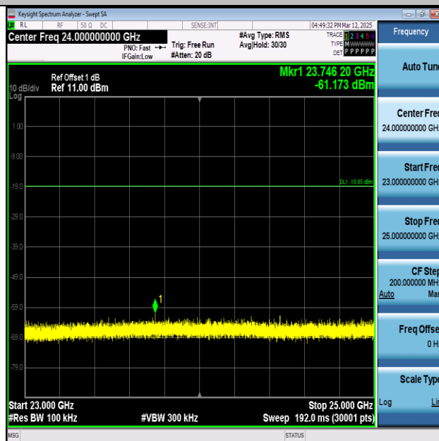
BLE_1M-Ant1-2440-23000~25000-PASS
