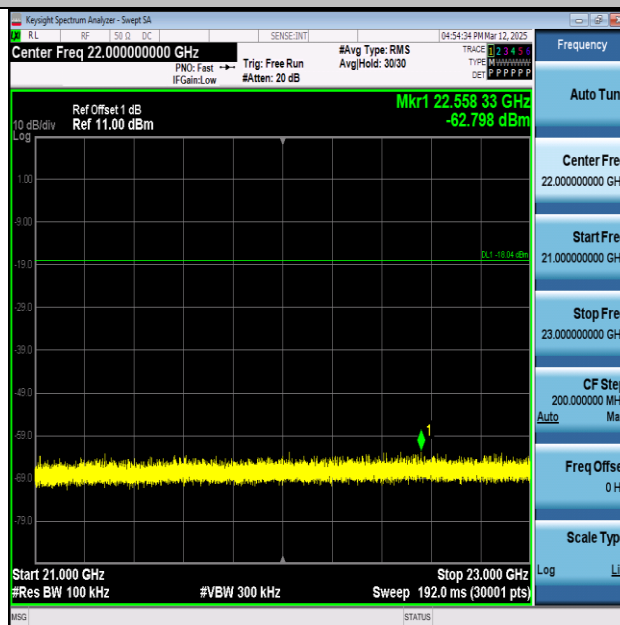
BLE_1M-Ant1-2480-21000~23000-PASS
