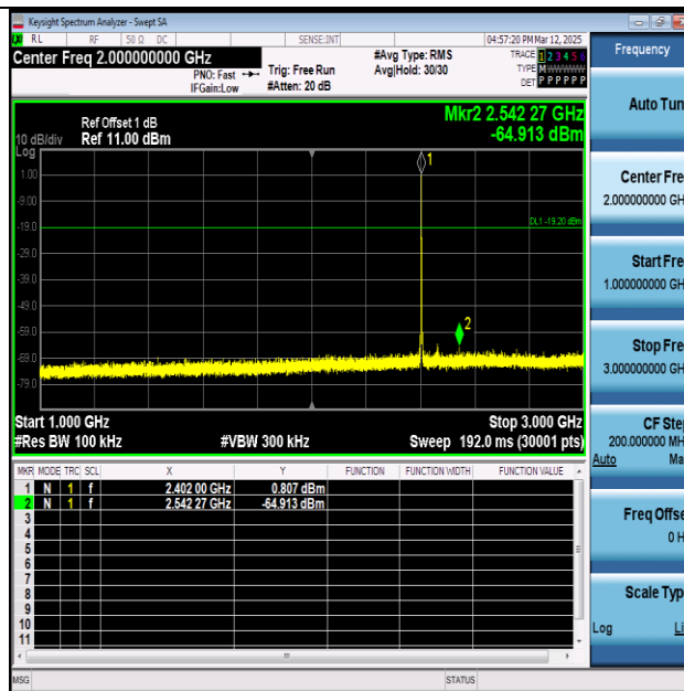
BLE_2M-Ant1-2402-1000~3000-PASS
