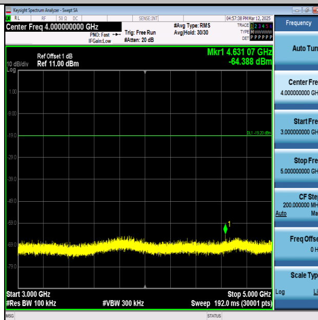
BLE_2M-Ant1-2402-3000~5000-PASS
