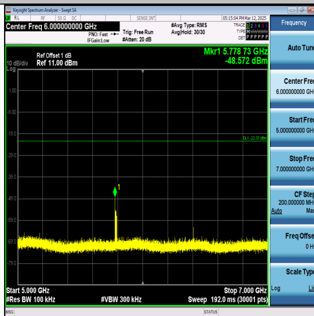
BLE_125K-Ant1-2402-5000~7000-PASS
