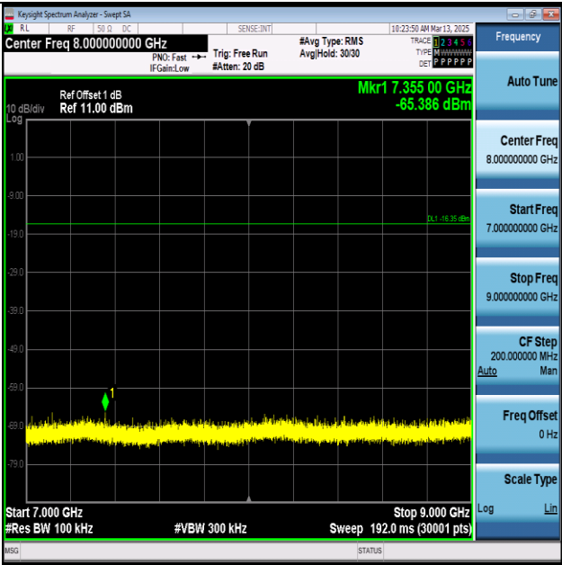
2DH5-Ant1-2441-7000~9000-PASS
