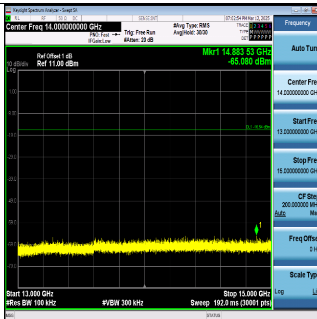
DH5-Ant1-2441-13000~15000-PASS
