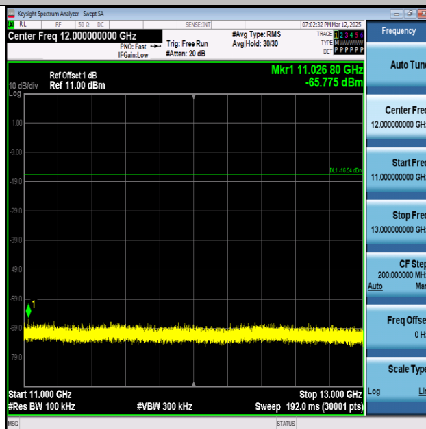
DH5-Ant1-2441-11000~13000-PASS
