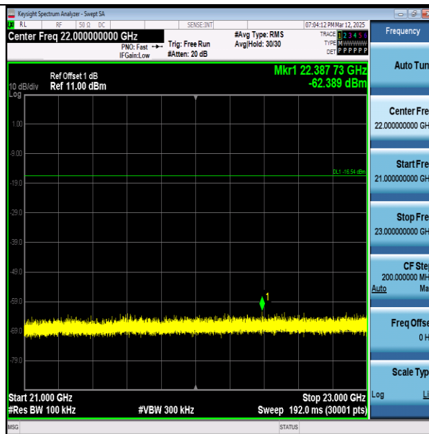
DH5-Ant1-2441-21000~23000-PASS
