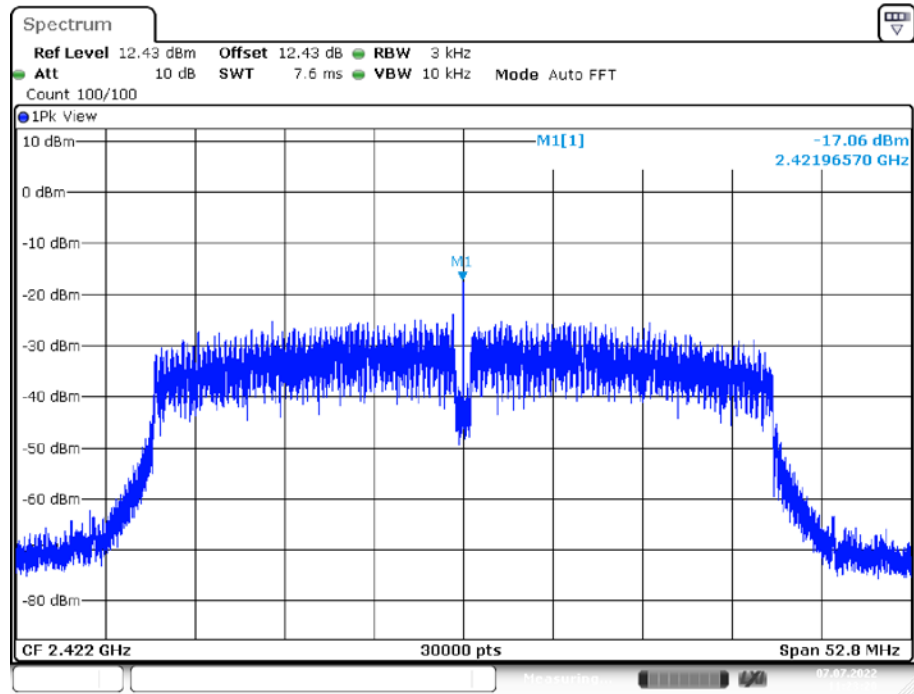
11N40SISO_Ant1_2422
