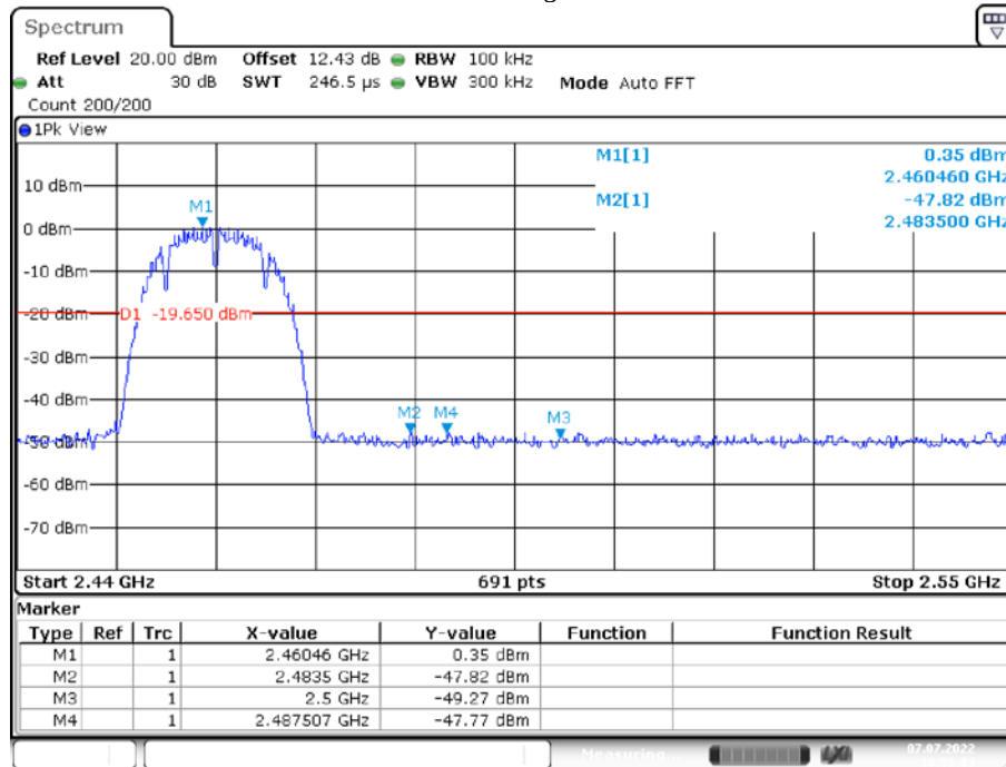
11B_Ant1_High_2462
