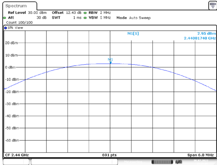
BLE_BT4.0_Ant1_2440
