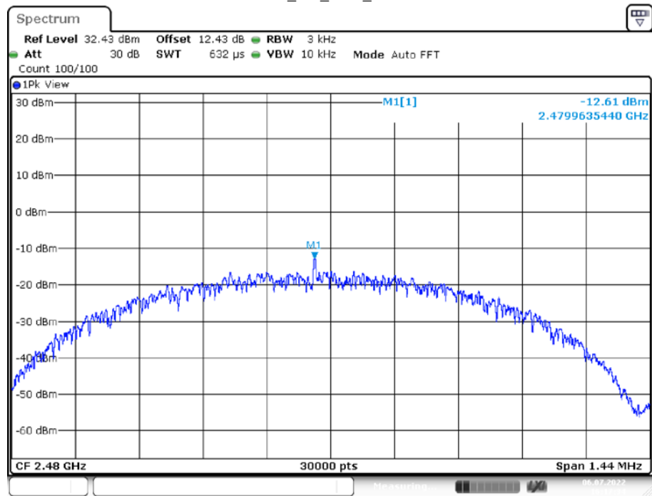
BLE_1M_Ant1_2480
