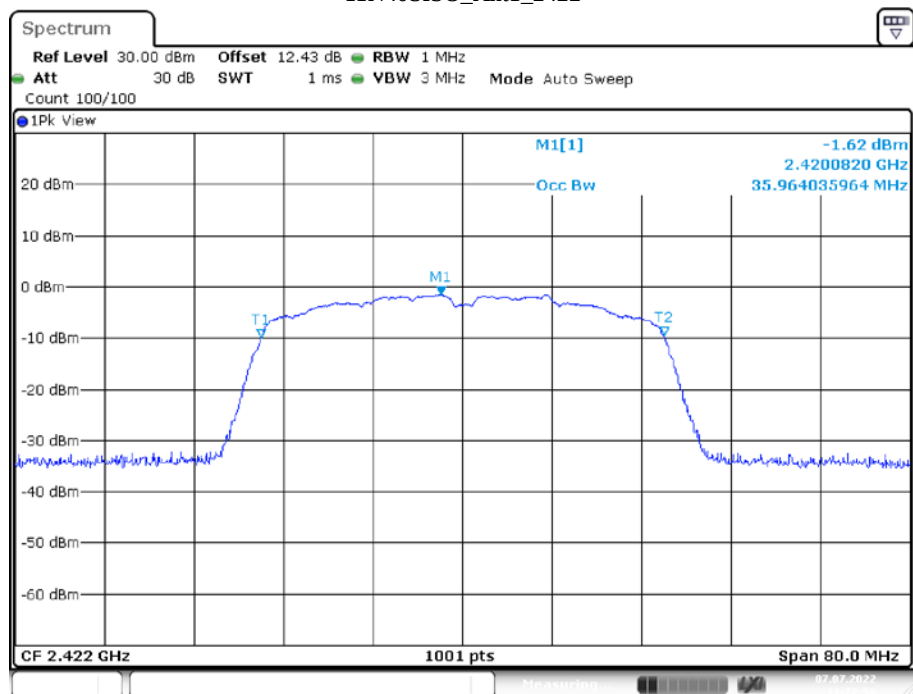
11N40SISO_Ant1_2422
