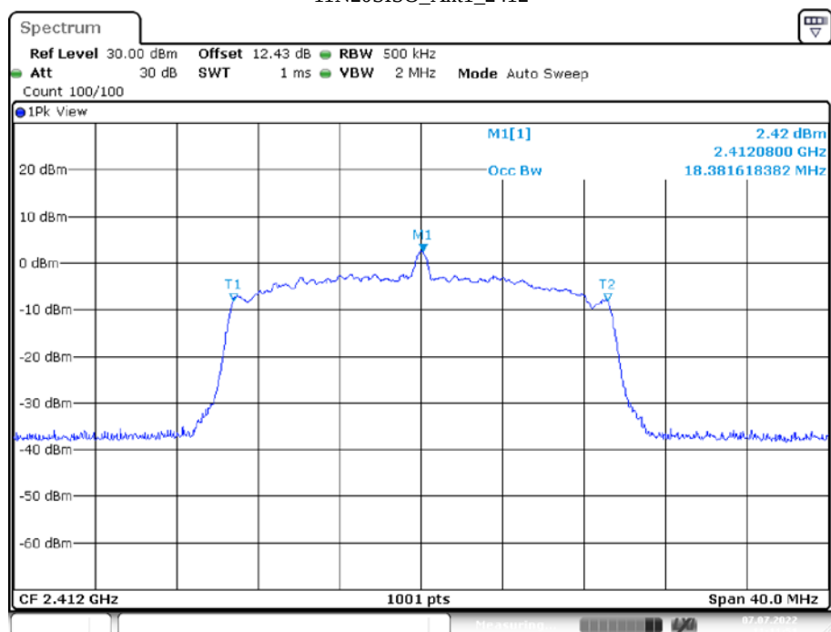
11N20SISO_Ant1_2412
