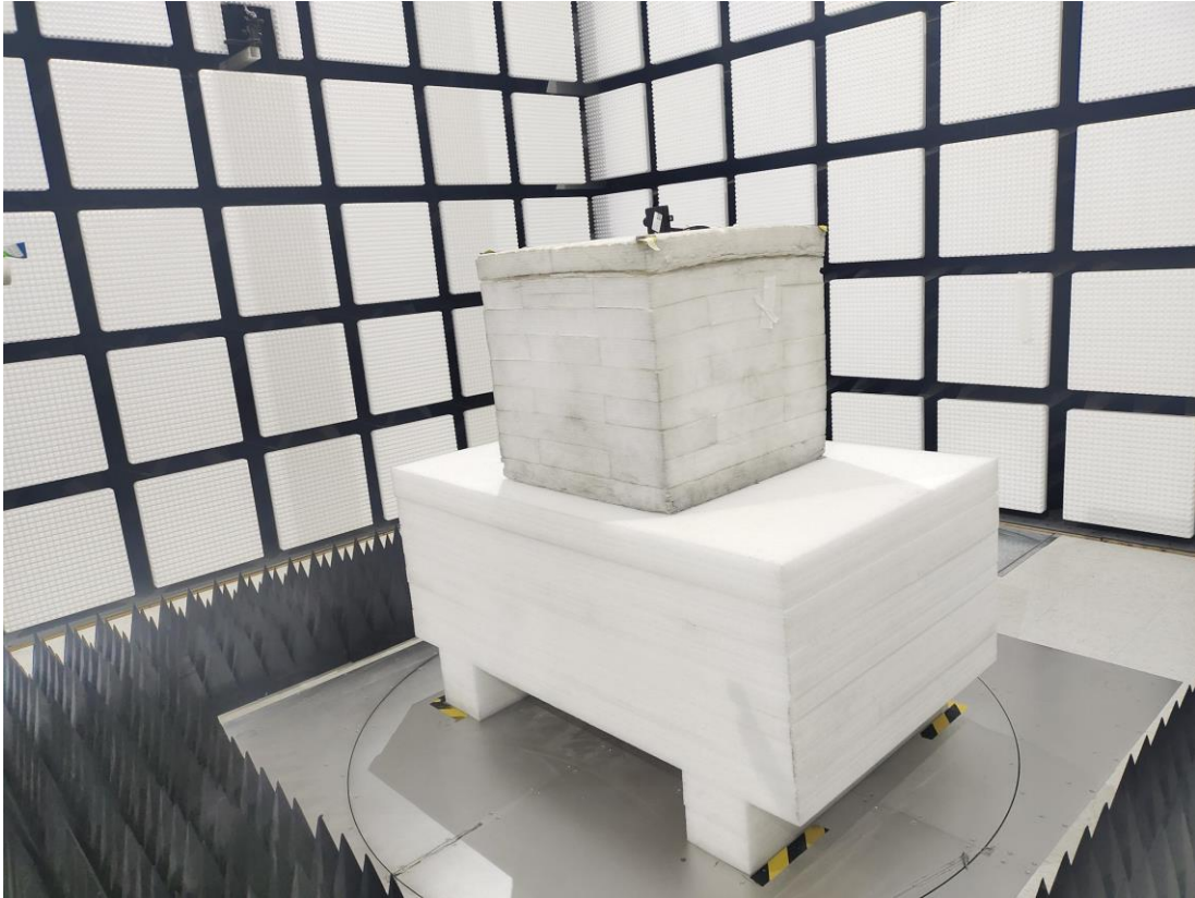
Radiated Emission 40GHz - 60GHz View
