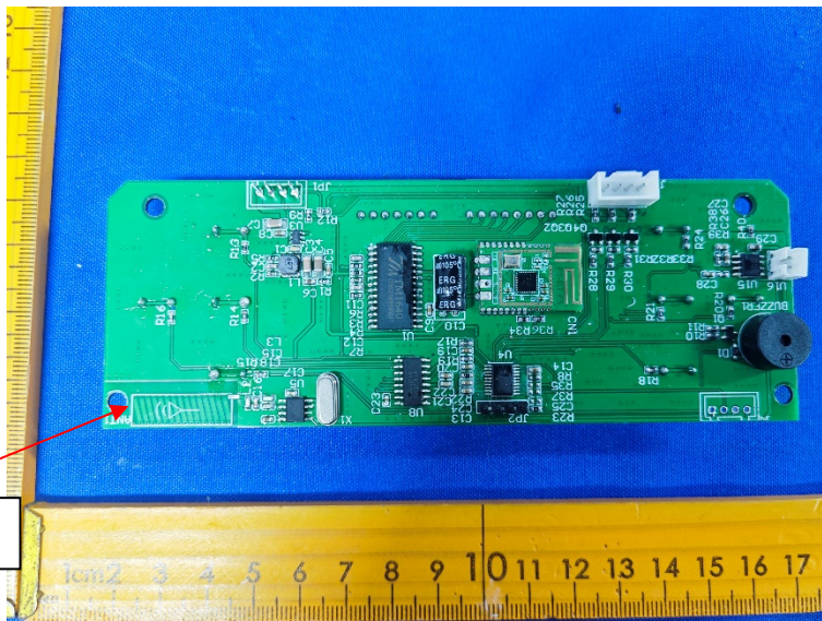
433M RX antenna
