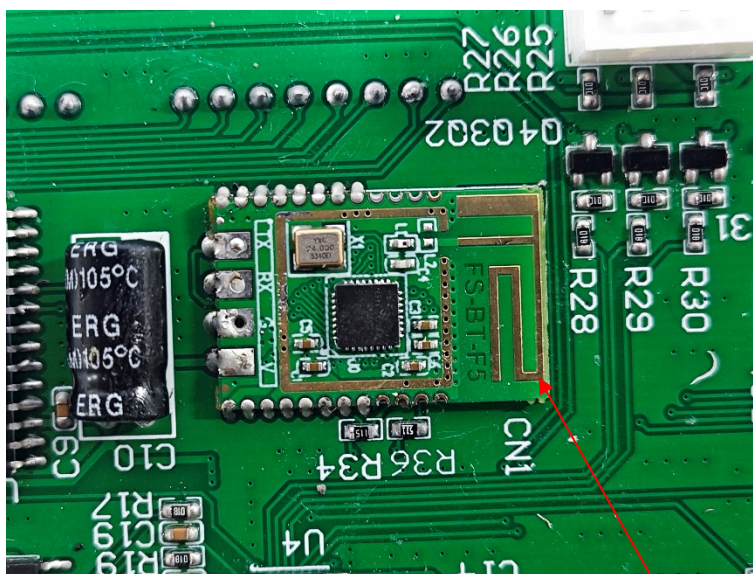
BT antenna
