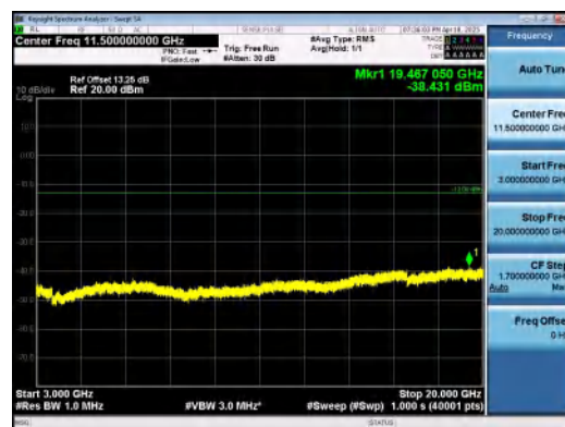
Band2-3MHz-16QAM-19185-15RB#0-3000~200 00-PASS
