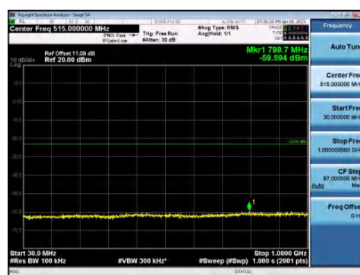
Band2-3MHz-16QAM-19185-15RB#0-30~1000-P ASS
