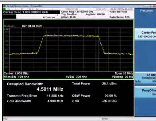
Band2-5MHz-16QAM-19175-25RB#0-PASS
