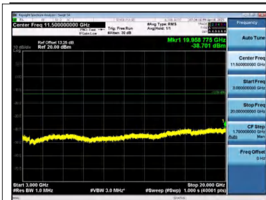
Band2-3MHz-16QAM-19185-1RB#14-3000~200 00-PASS
