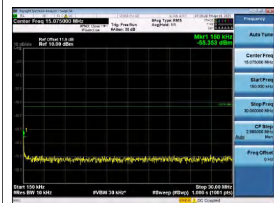
Band2-3MHz-16QAM-19185-15RB#0-0.15~30-P ASS
