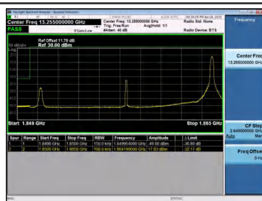
Band2-15MHz-QPSK-18675-1RB#74-PASS
