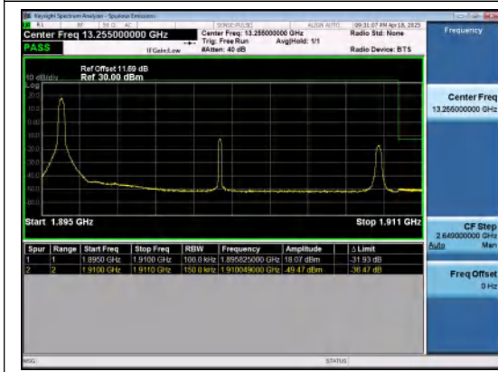
Band2-15MHz-16QAM-18675-1RB#74-PASS
