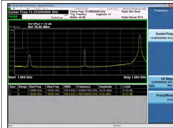
Band2-15MHz-16QAM-18675-1RB#74-PASS
