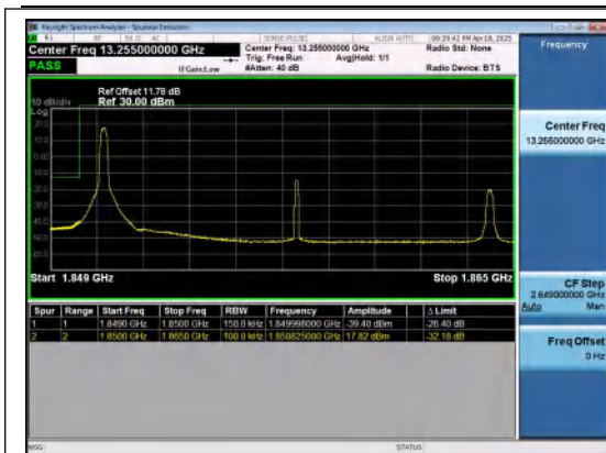
Band2-15MHz-QPSK-18675-1RB#0-PASS
