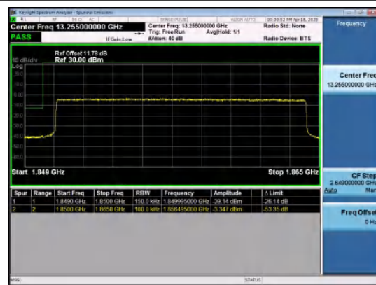
Band2-15MHz-16QAM-18675-75RB#0-PASS
