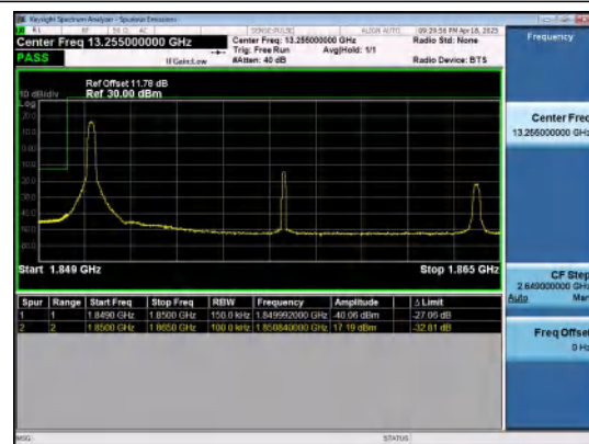
Band2-15MHz-16QAM-18675-1RB#0-PASS
