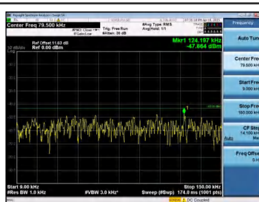
Band2-3MHz-16QAM-19185-15RB#0-0.009~0.1 5-PASS
