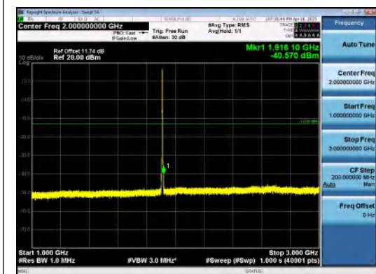
Band2-3MHz-16QAM-19185-15RB#0-1000~300 0-PASS
