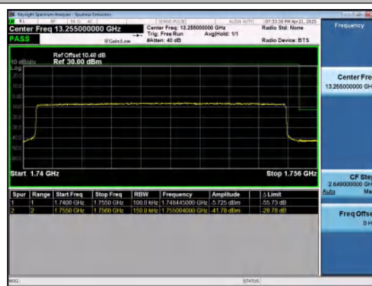
Band4-15MHz-16QAM-20325-75RB#0-PASS
