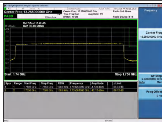
Band4-15MHz-QPSK-20325-75RB#0-PASS
