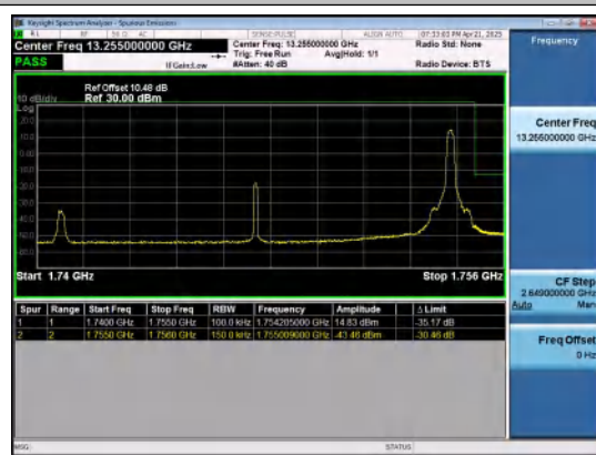
Band4-15MHz-16QAM-20325-1RB#74-PASS
