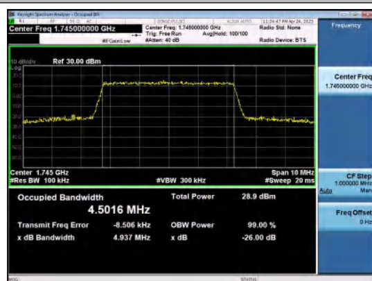
Band66-5MHz-QPSK-132322-25RB#0-PASS
