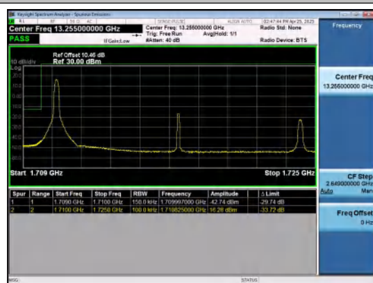
Band66-15MHz-QPSK-132047-1RB#0-PASS
