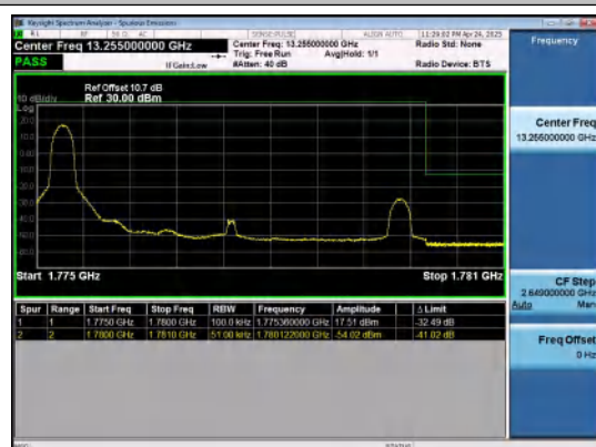
Band66-5MHz-QPSK-132647-1RB#0-PASS
