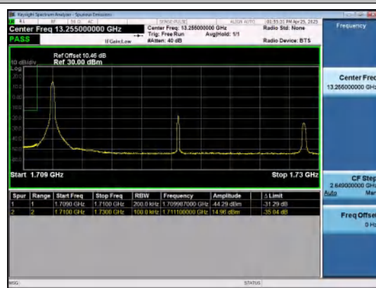
Band66-20MHz-16QAM-132072-1RB#0-PASS
