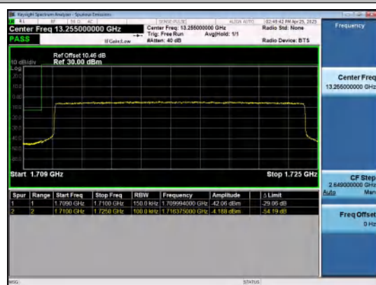
Band66-15MHz-QPSK-132047-75RB#0-PASS
