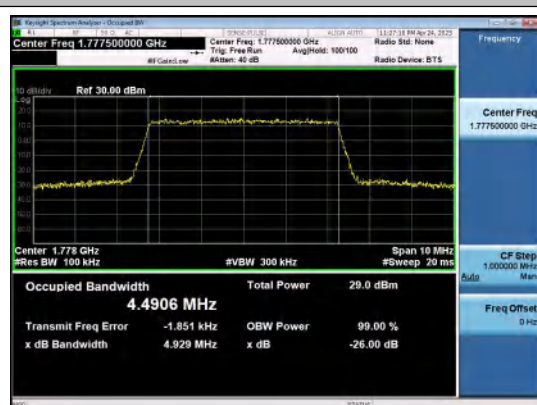
Band66-5MHz-QPSK-132647-25RB#0-PASS
