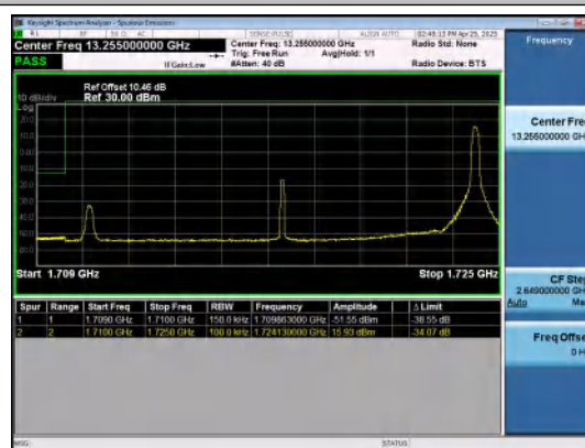
Band66-15MHz-QPSK-132047-1RB#74-PASS
