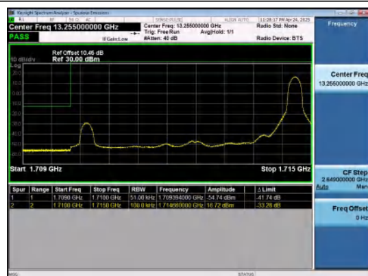
Band66-5MHz-16QAM-131997-1RB#24-PASS
