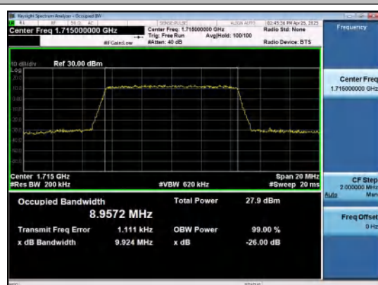
Band66-10MHz-QPSK-132022-50RB#0-PASS
