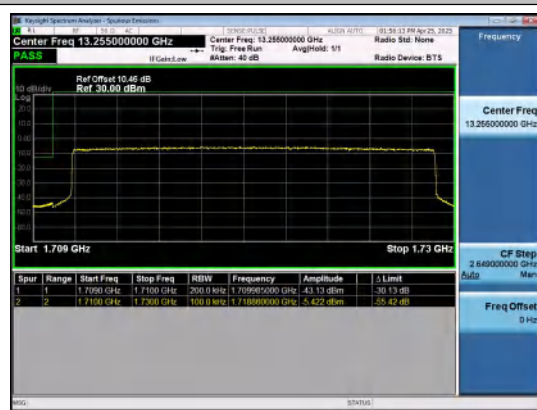
Band66-20MHz-QPSK-132072-100RB#0-PASS
