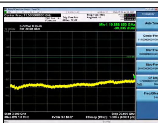
Band66-20MHz-16QAM-132322-1RB#0-3000~20000-PASS
