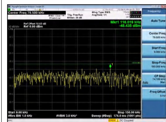
Band66-20MHz-16QAM-132322-1RB#99-0.009~0.15-PASS
