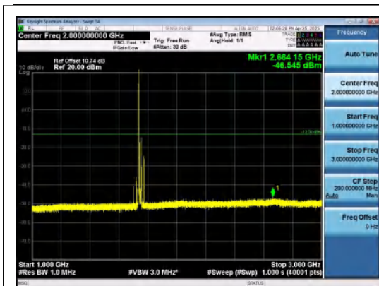
Band66-20MHz-16QAM-132322-1RB#0-1000~3000-PASS
