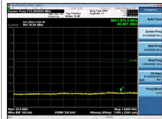
Band66-20MHz-16QAM-132322-1RB#99-30~1000-PASS
