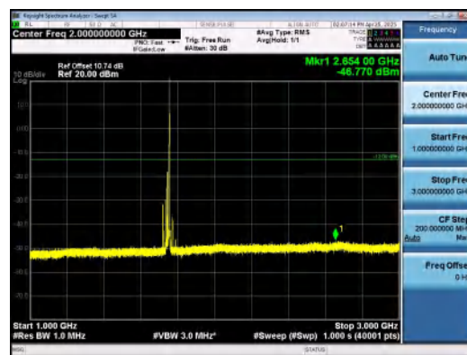
Band66-20MHz-16QAM-132322-1RB#99-1000~3000-PASS
