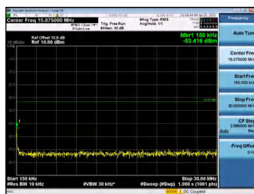
Band66-20MHz-16QAM-132322-1RB#99-0.15~30-PASS
