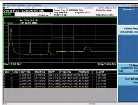
Band7-10MHz-QPSK-21400-1RB#0-PASS
