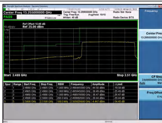
Band7-10MHz-16QAM-20800-50RB#0-PASS
