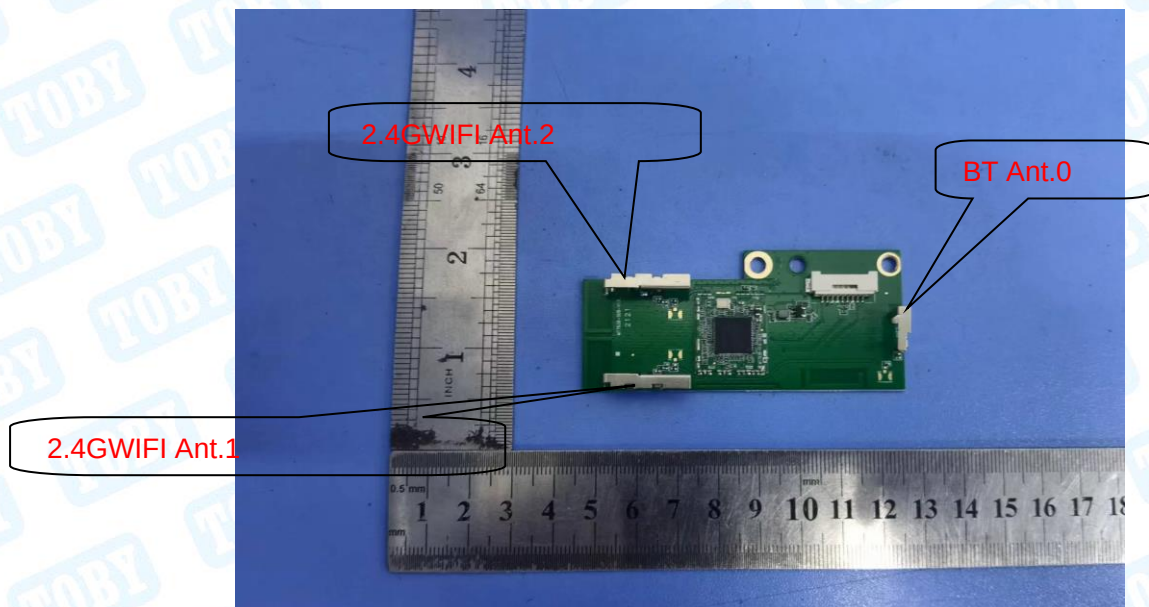
Photo 15 Appearance of PCB
