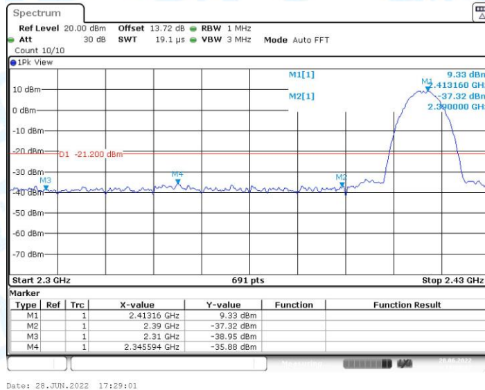
11B-CDD_Ant2_Low_2412_Peak
