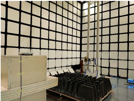
Fundamental & Spurious Emission & Restrict band radiated emission – FCC 15.231(b) and 15.205: 1 GHz – 6 GHz
