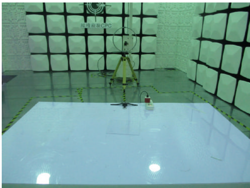
Setup Photo FCC ID: 2A7OT-F2
