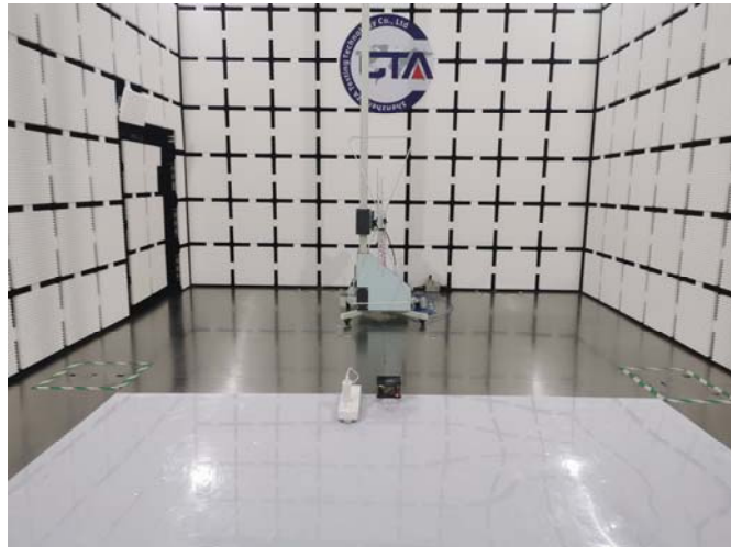
radiation H
