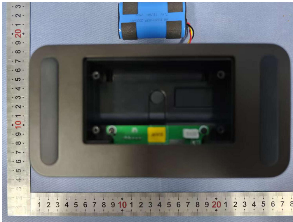
Internal view of unit (Model:NAVA100-BK)
