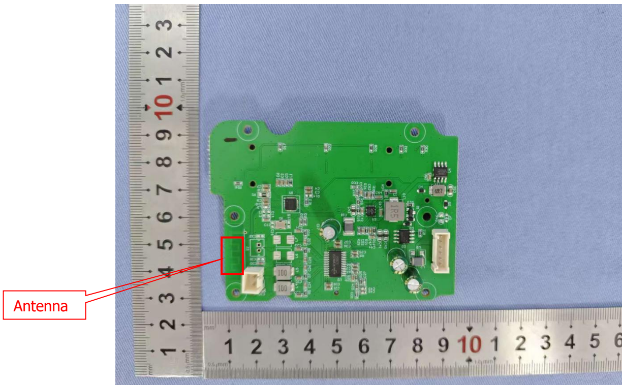
Internal view of unit (Model:NAVA100-WH)
