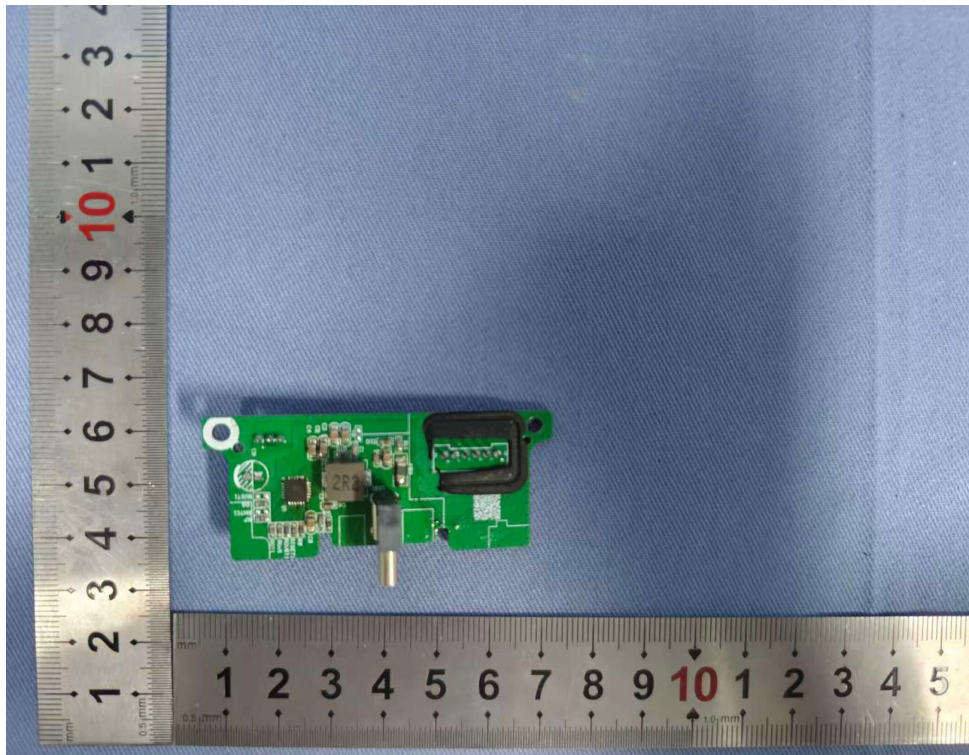
Internal view of unit (Model:NAVA100-BK)
