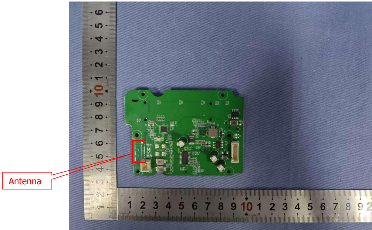
Internal view of unit (Model:NAVA100-BK)
