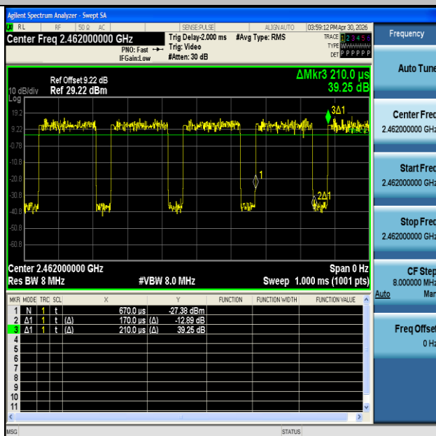
NTNV-11N20MIMO-Ant2-2462
